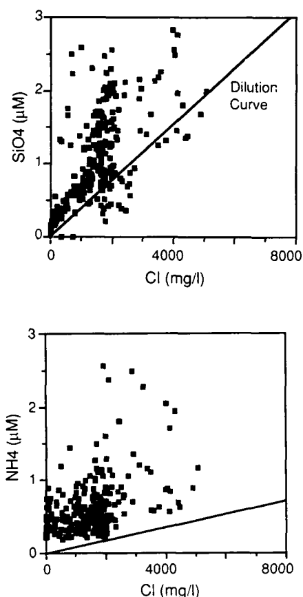
Figure 65. Dilution curves for multiyear ice for all samples combined for \text{SiO}_4 and \text{NH}_4 .
