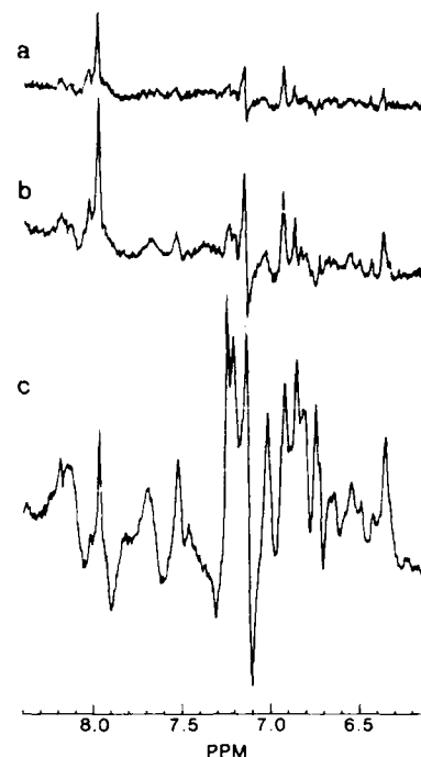
FIGURE 4: Illustrative titration difference spectra: \text{Fab}(\text{0}) - \text{Fab}(\text{SL}) and \text{Fab}(\text{DNP-DG}) - \text{Fab}(\text{SL}) . Signals are due to protons in the 2- and 5-positions of tryptophan, the other positions being deuteriated. \text{Fab}(\text{0}) - \text{Fab}(\text{SL}) for (a) 6.8% and (b) 100% occupancy of the combining site. \text{Fab}(\text{DNP-DG}) - \text{Fab}(\text{SL}) for (c) 100% occupancy of the combining site.
