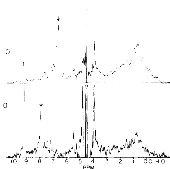
FIGURE 6: NMT difference spectra resulting from saturation of resonances of the recombinant H(II) . (a) The dipole-dipole NMT is from a light chain proton of tryptophan (Trp-91) at 7.93 ppm to the CH_2 groups of DNP-DG at 3.95 ppm and to the aromatic proton at position 6 of DNP at 5.5 ppm. The NMT to the aromatic proton at position 3 of DNP at 9.15 ppm is due to chemical exchange between bound and free hapten. The signals at 7.46 and 7.2 ppm are probably due to intramolecular dipole-dipole NMT within Trp-91. (b) The dipole-dipole NMT is from a tryptophan residue of the heavy chain (probably Trp-47) to the CH_2 groups of DNP-DG. The NMT to the aromatic proton at 9.15 ppm is due to chemical exchange.
