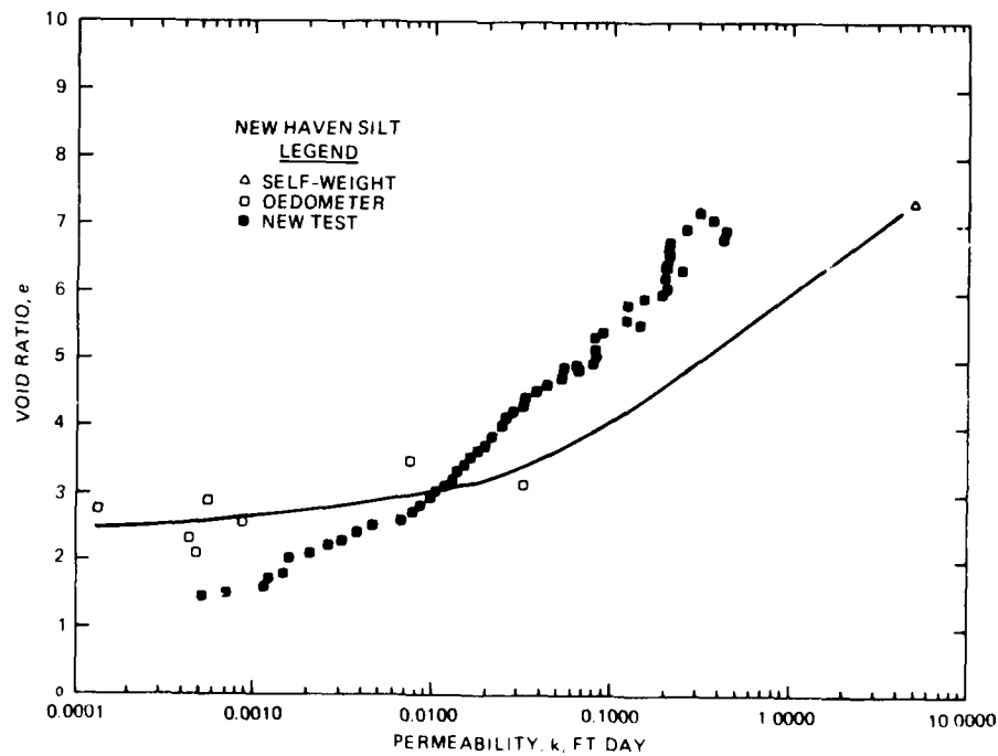
Figure 34. Void ratio-permeability relationship for New Haven silt capping material
