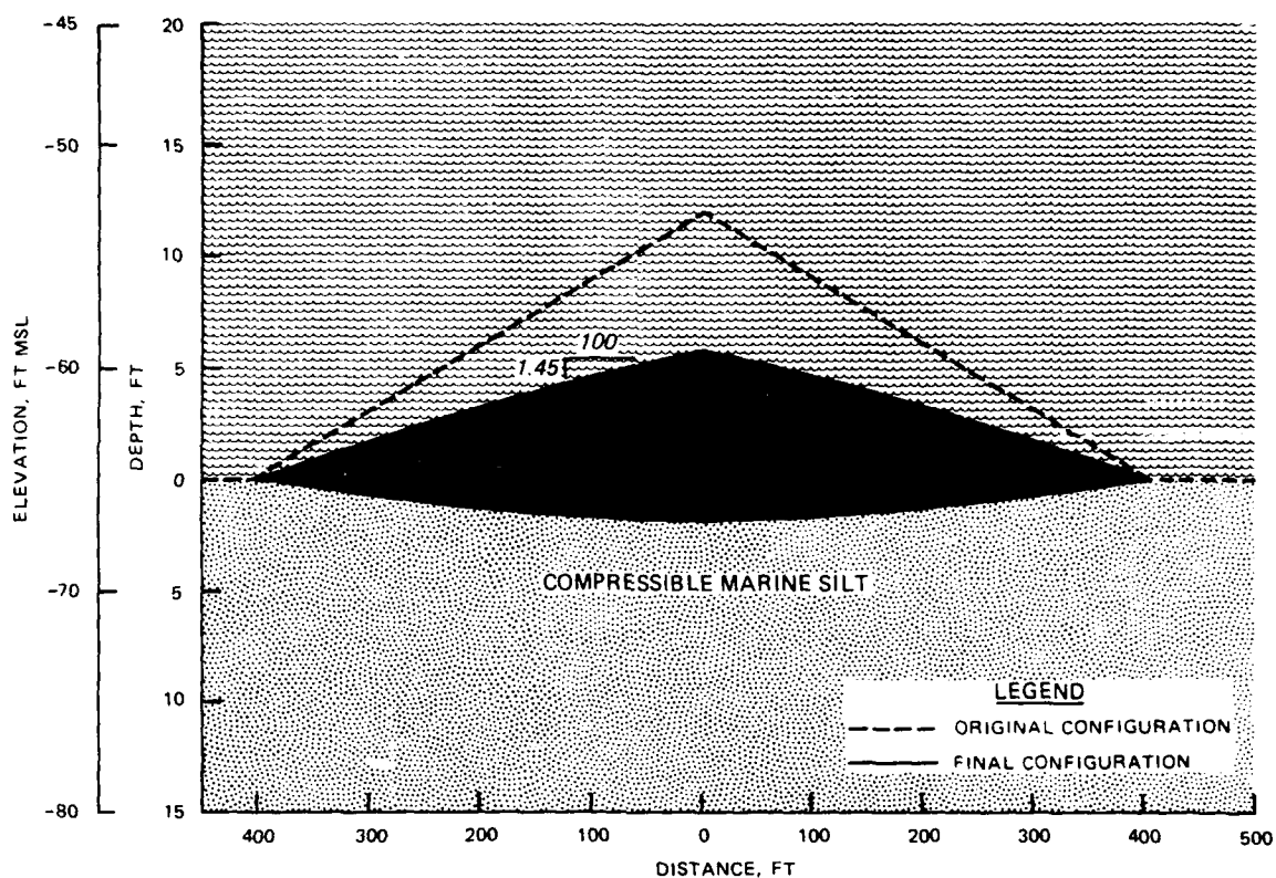
Figure 43. Predicted mound configuration at completion of consolidation of STNH-N mound
