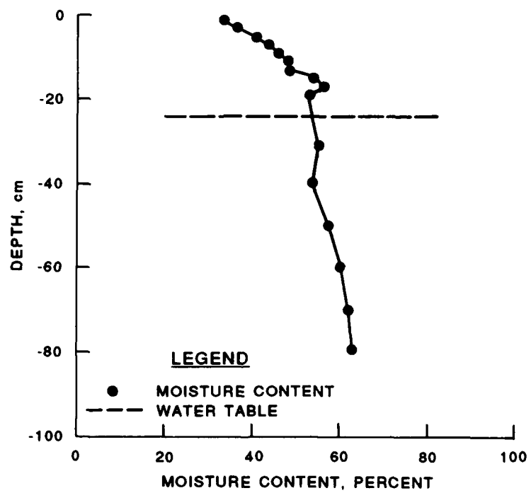
c. Moisture profile, Site 2, 11 September 1987
