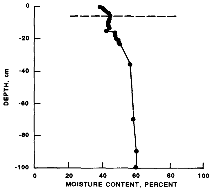
b. Moisture profile, Site 1, 21 August 1987
