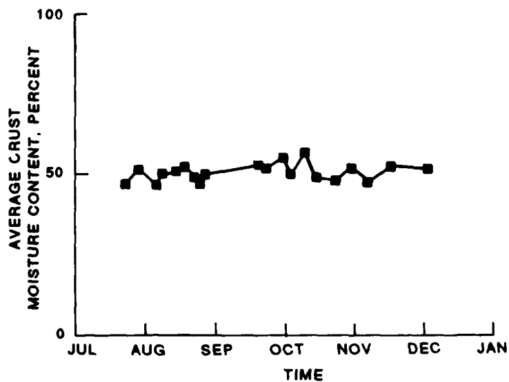
Figure 14. Crust moisture content as a function of time for the five sites (Continued)
