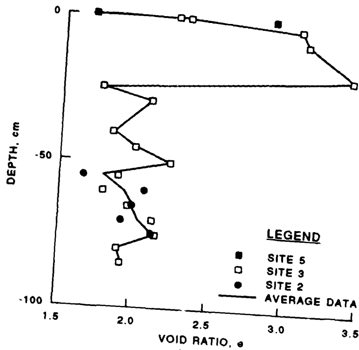
Figure 10. Void ratio profiles for three sites and the averaged profile
