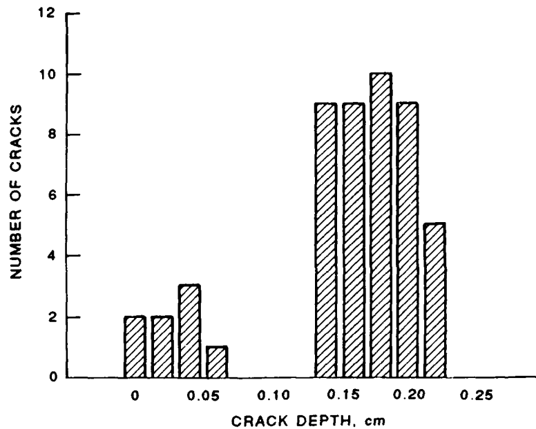
Figure 13. Frequency distribution of crack depths for Site 2, 5 August 1987
