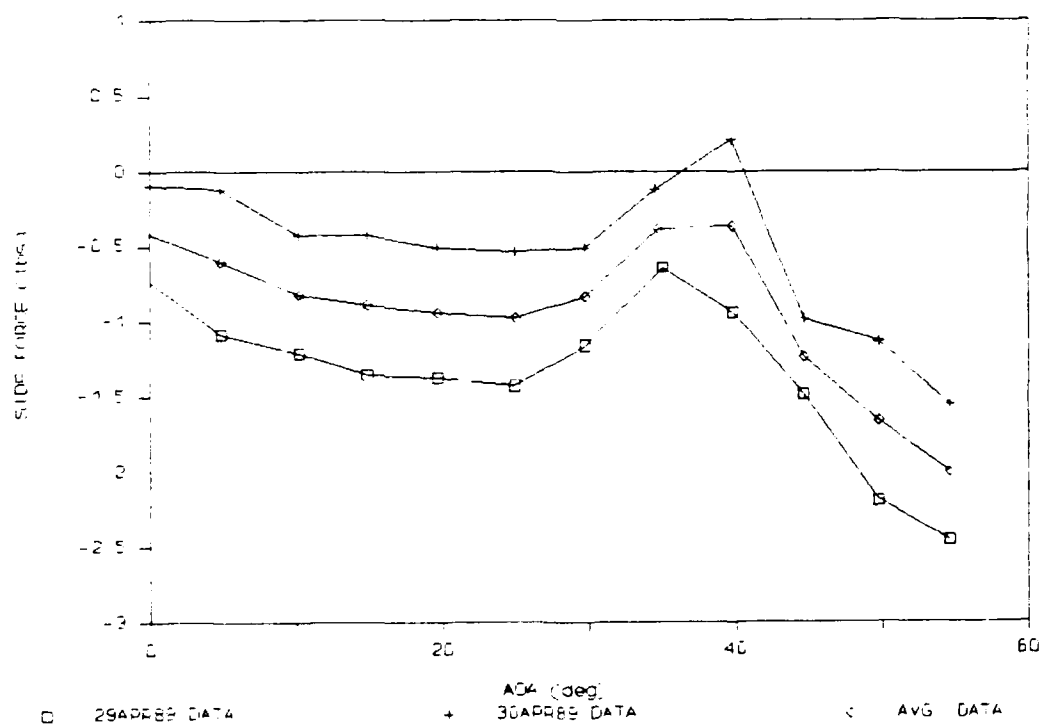
Figure 35. Side Force (Fwd: Inboard Long, Aft: Nozzle Short)
