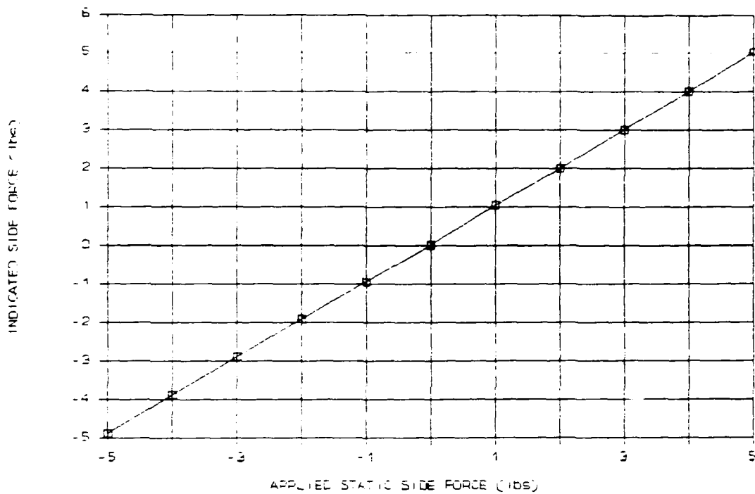
Figure 16. Side Force Static Calibration
