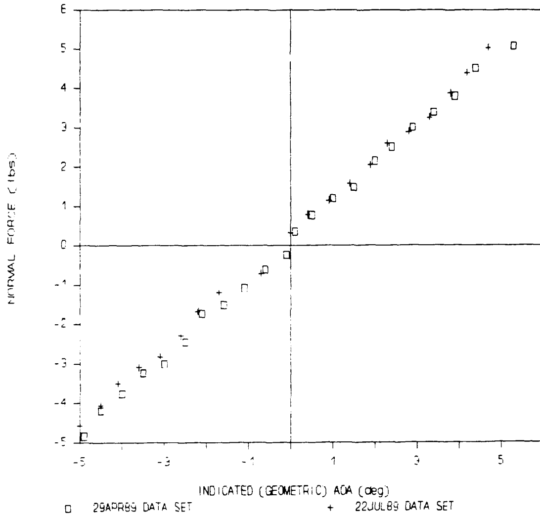
Figure 20. Determination of the Zero-Lift AOA
