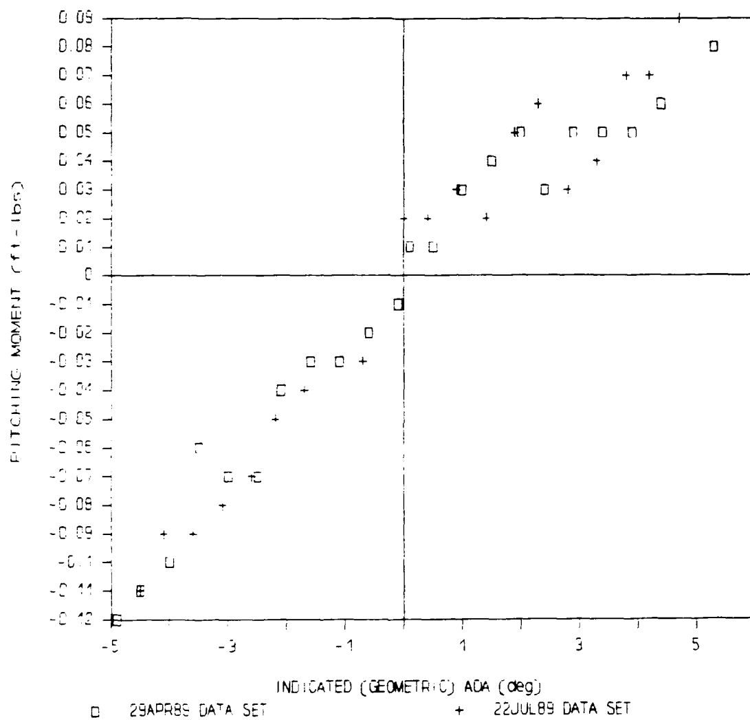
Figure 21. Determination of the Trim AOA
