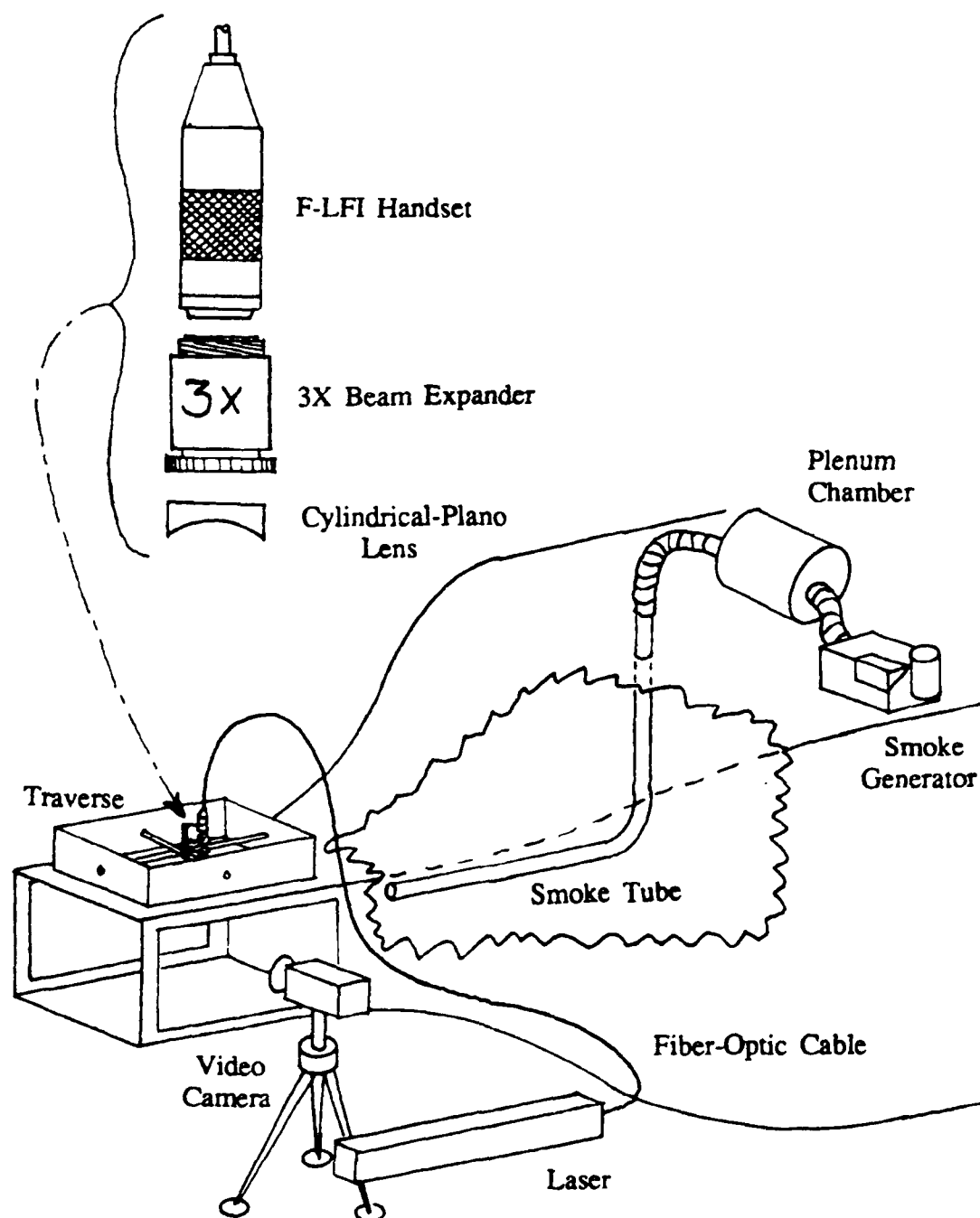
Figure 13. Flow Visualization System
