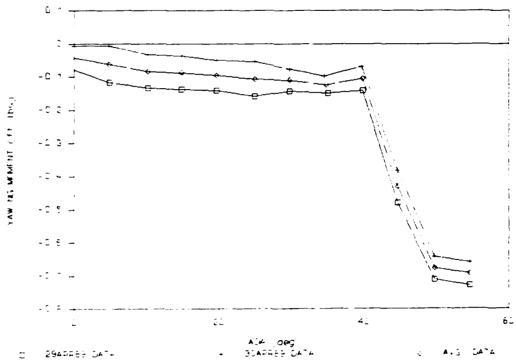
Figure 39. Yawing Moment (Fwd: Inboard Long. Aft: Nozzle Short)
