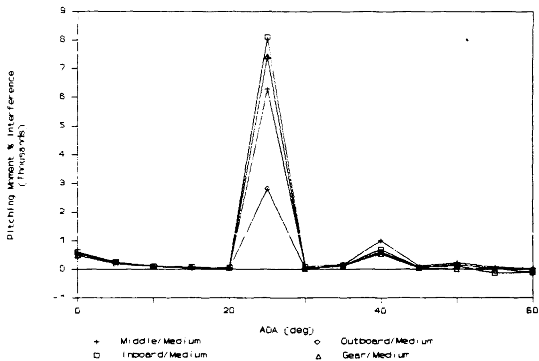
Figure 121. Pitching Moment % Interference (Aft: Hook/Long)
