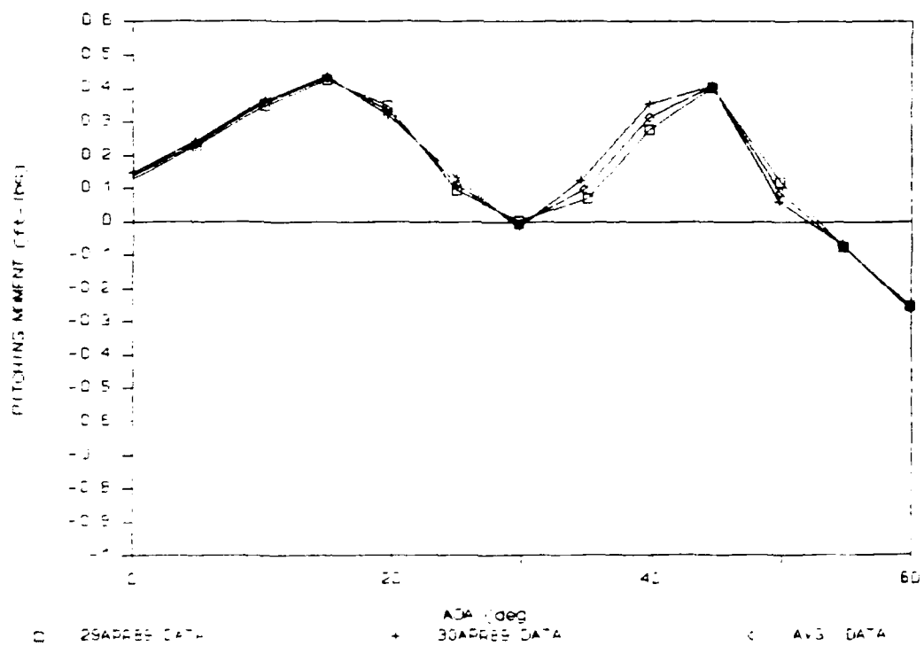
Figure 43. Pitching Moment (Fwd: Middle Long. Aft: Hook short)
