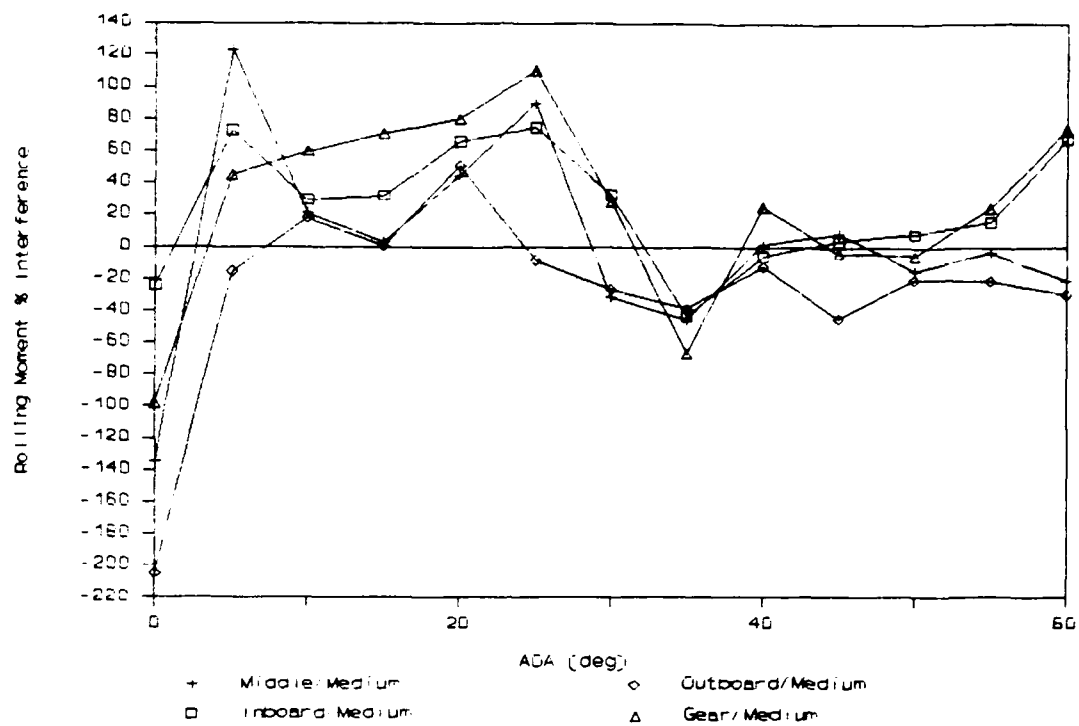
Figure 122. Rolling Moment % Interference (Aft: Hook/Long)
