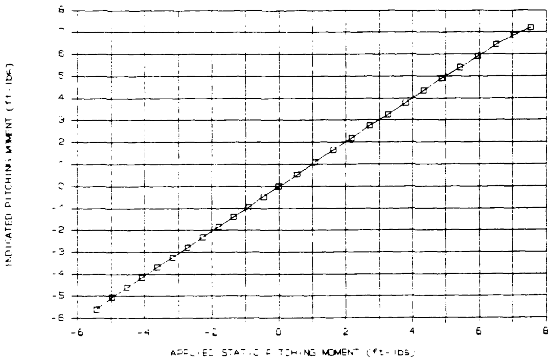
Figure 17. Pitching Moment Static Calibration
