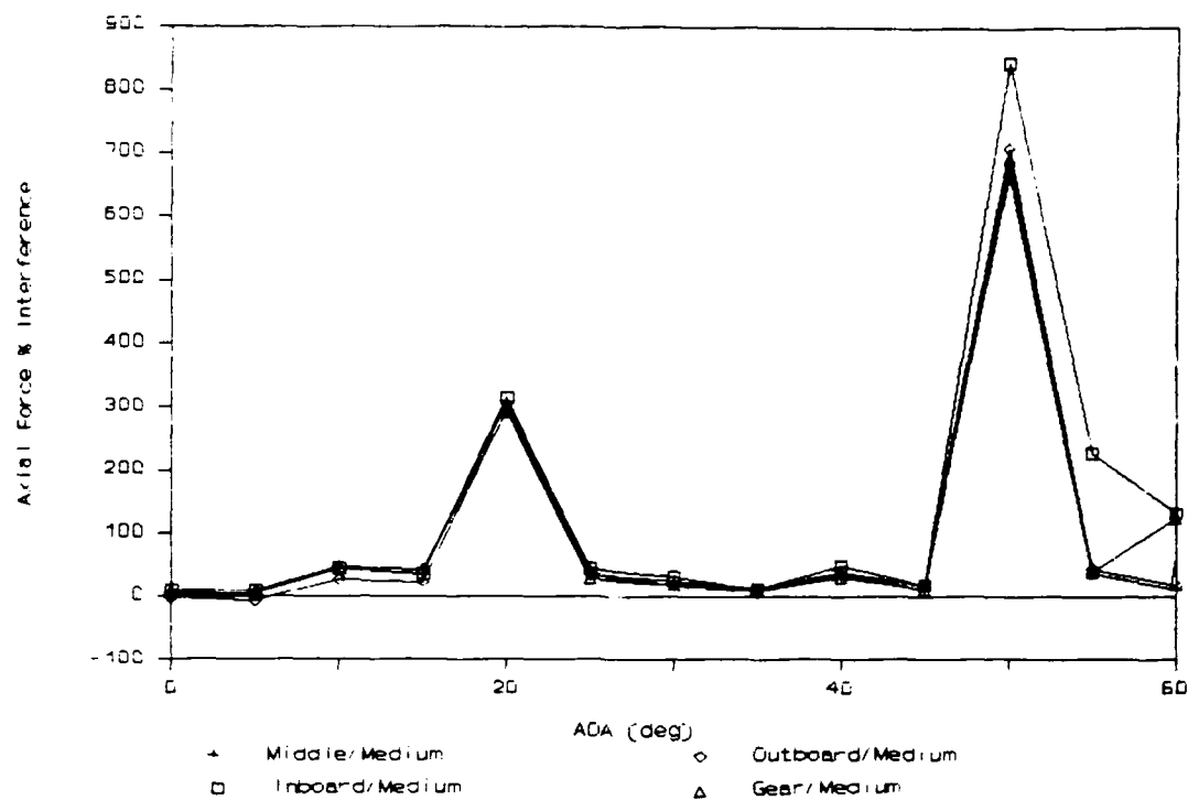
Figure 120. Axial Force % Interference (Aft: Hook/Long)
