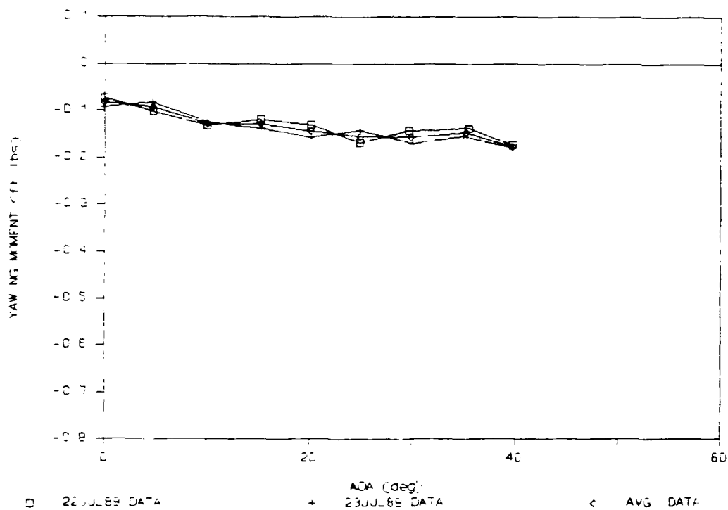
Figure 87. Yawing Moment (Fwd: Middle Medium, Aft: Nozzle Long)
