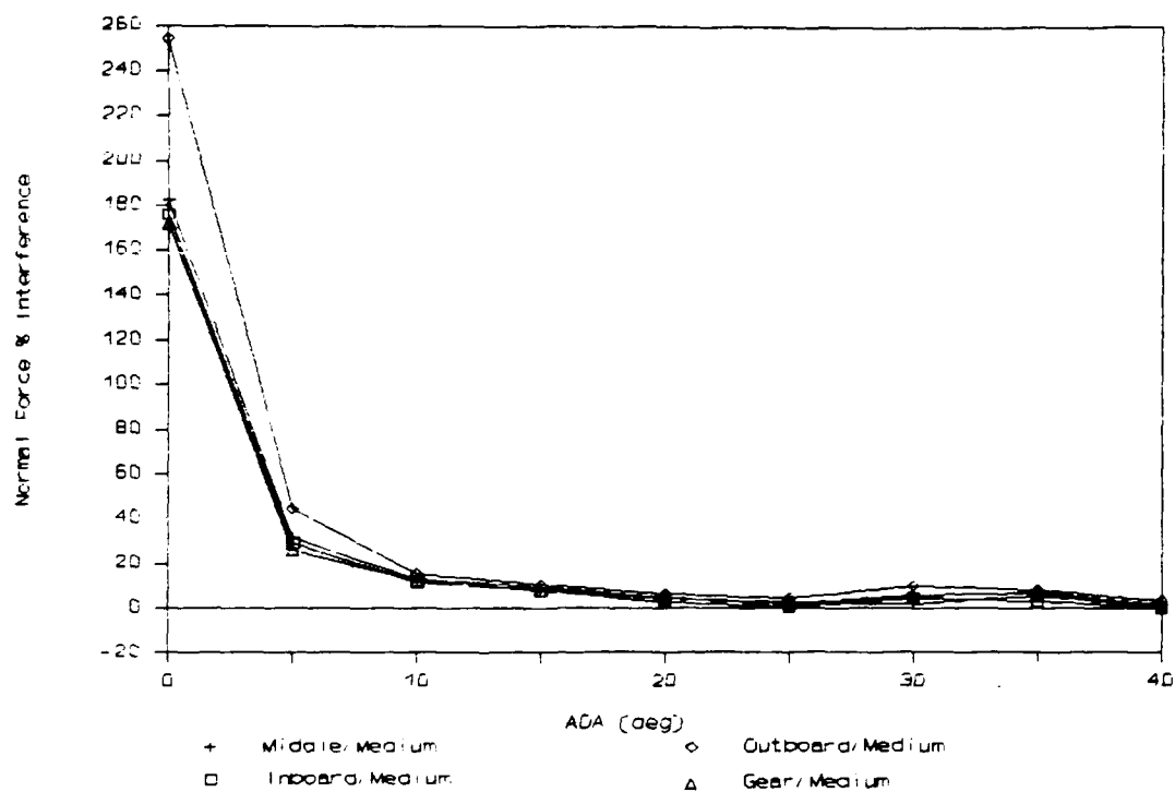
Figure 130. Normal Force % Interference (Aft: Nozzle/Long)
