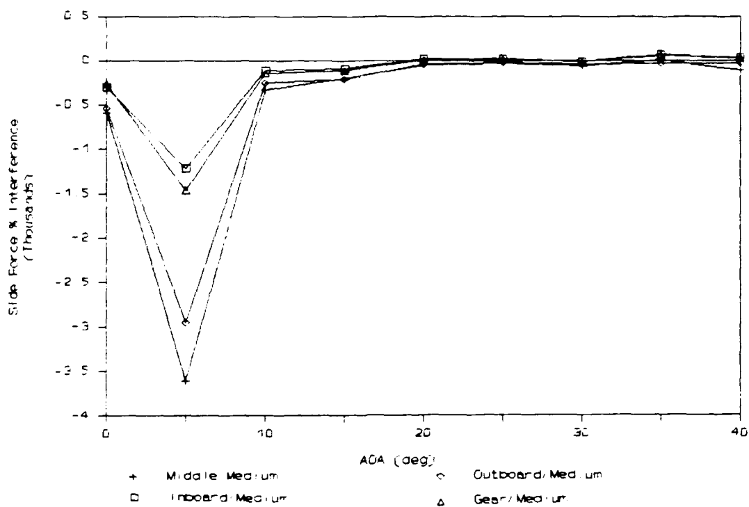
Figure 131. Side Force % Interference (Aft: Nozzle/Long)
