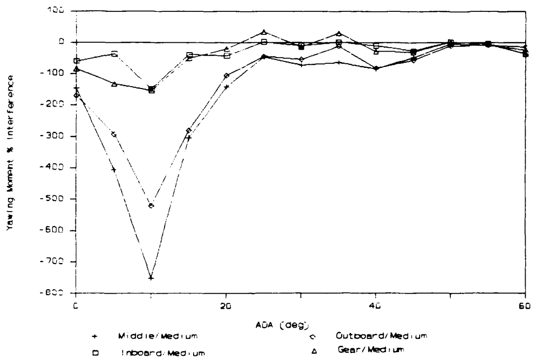
Figure 123. Yawing Moment % Interference (Aft: Hook/Long)
