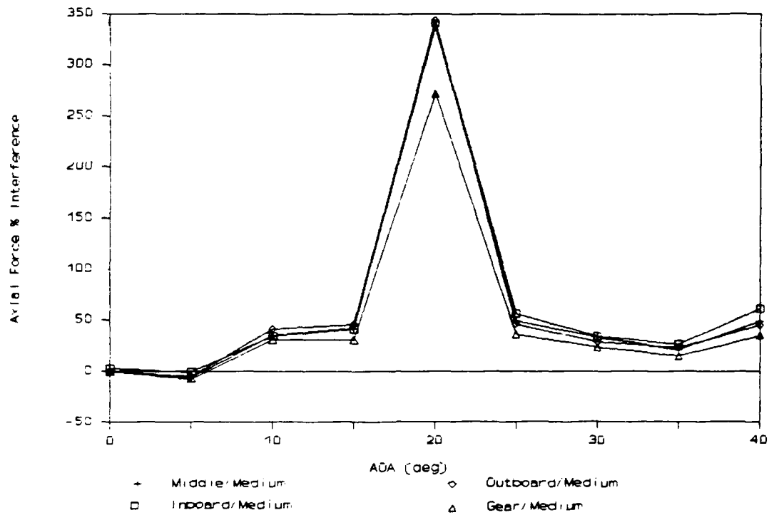
Figure 132. Axial Force % Interference (Aft: Nozzle/Long)
