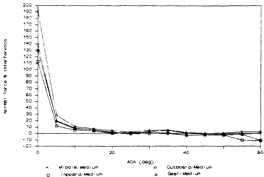
Figure 118. Normal Force % Interference (Aft: Hook/Long)
