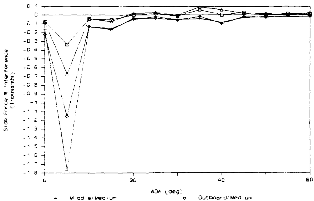
Figure 119. Side Force % Interference (Aft: Hook/Long)
