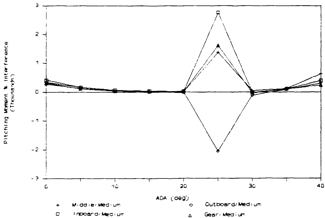
Figure 133. Pitching Moment % Interference (Aft: Nozzle/Long)
