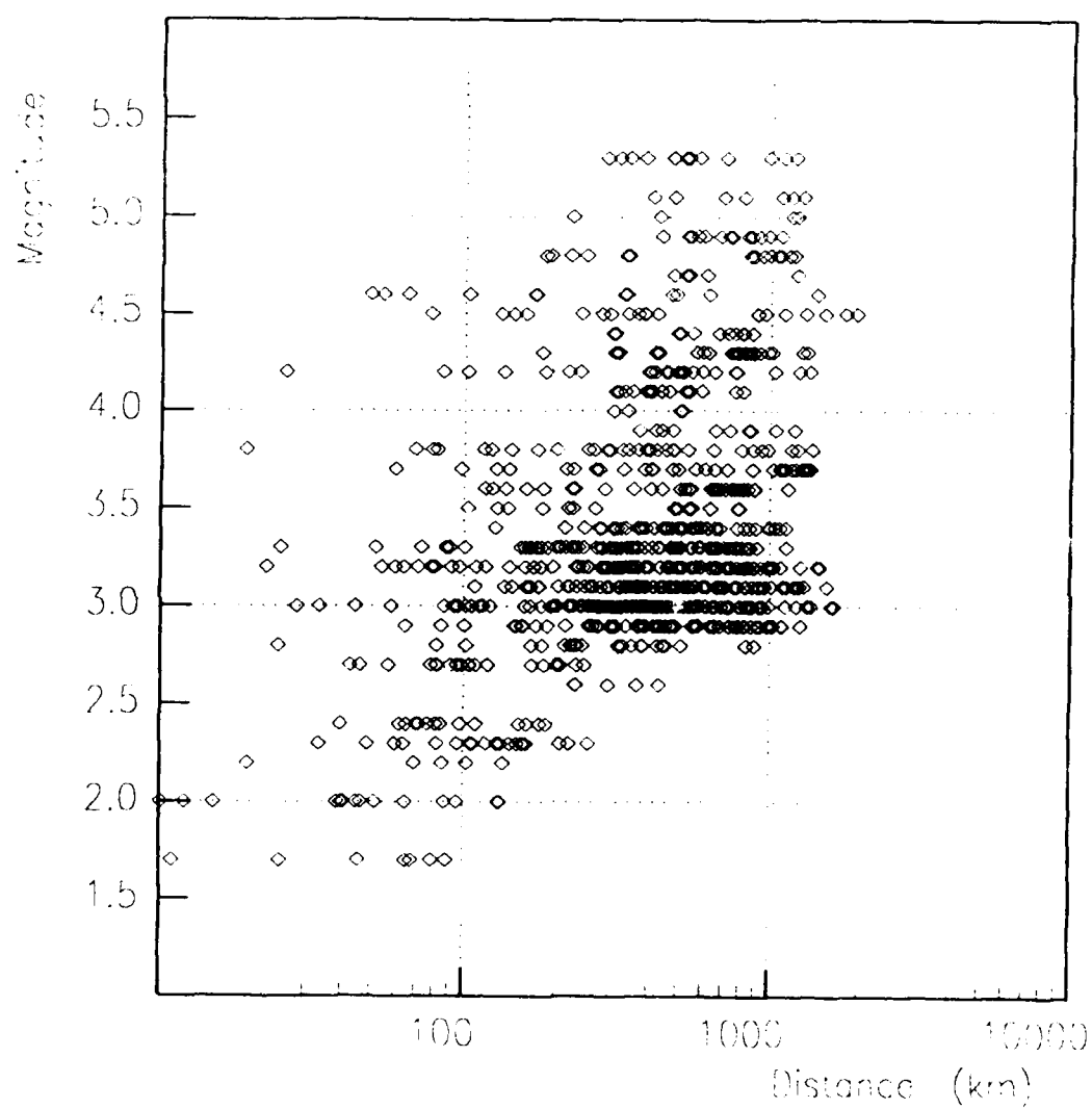
Fig. 2.3.2. Magnitude-distance distribution for all of the data in the data base (203 events, 1028 records).
