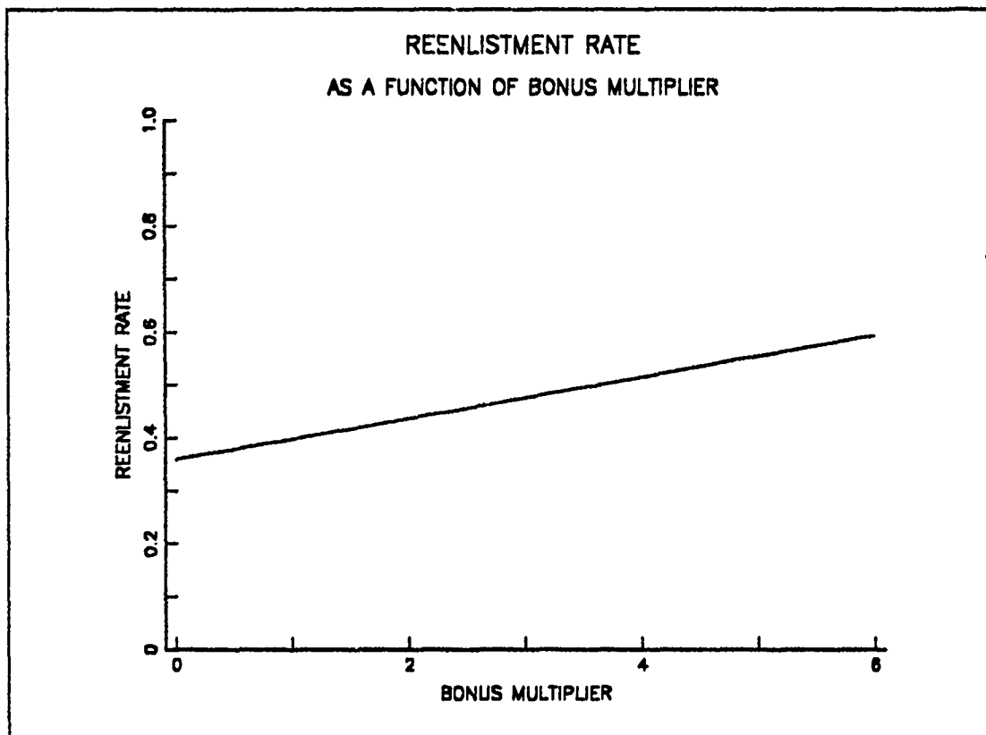
Figure 1. Sample of Input Required for Bonus Model (Hypothetical)
