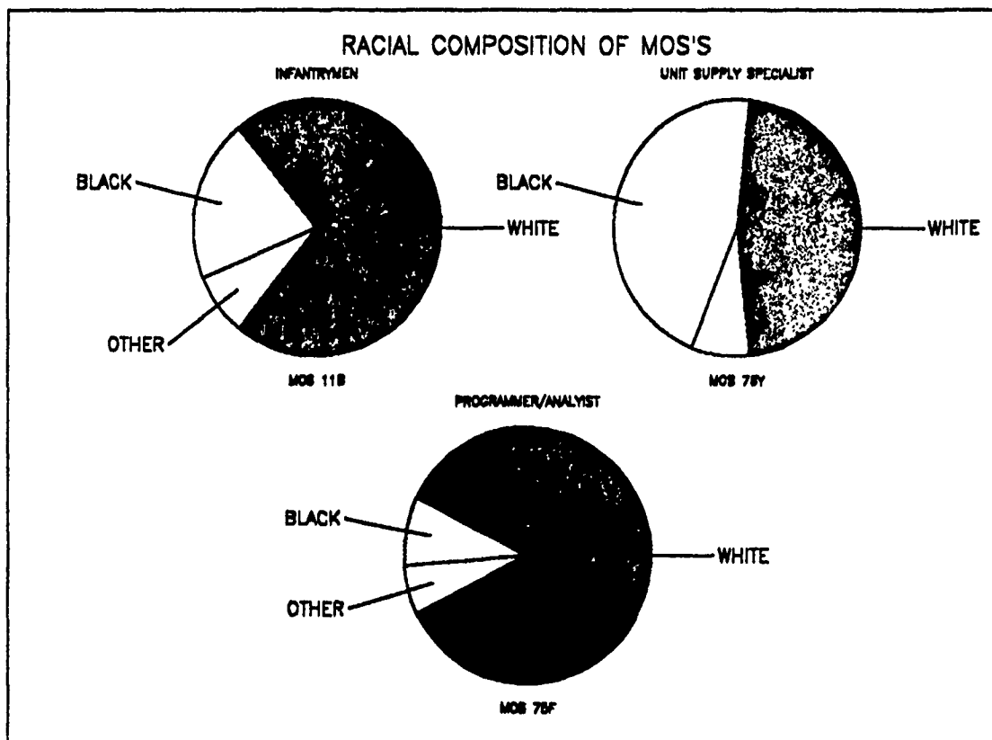
Figure 8. Racial Composition of Three MOS's
