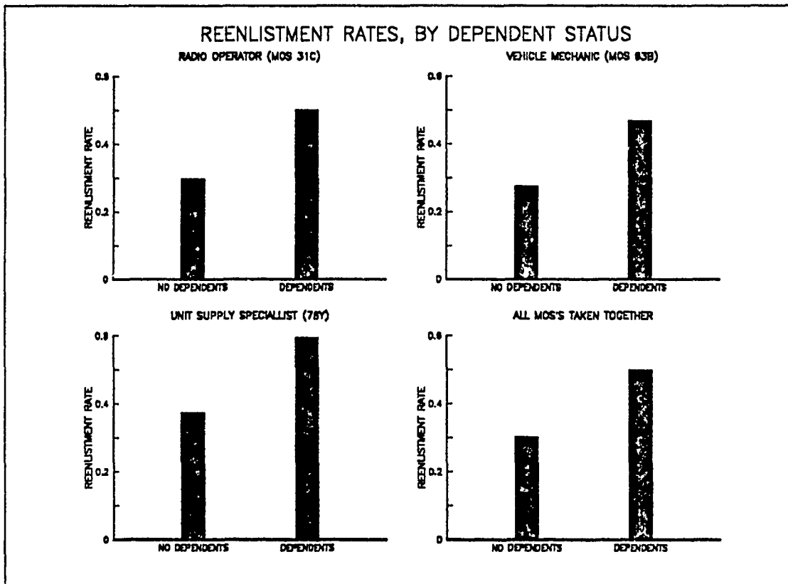
Figure 6. Reenlistment Rates for Differing MOS's by Dependent Status
