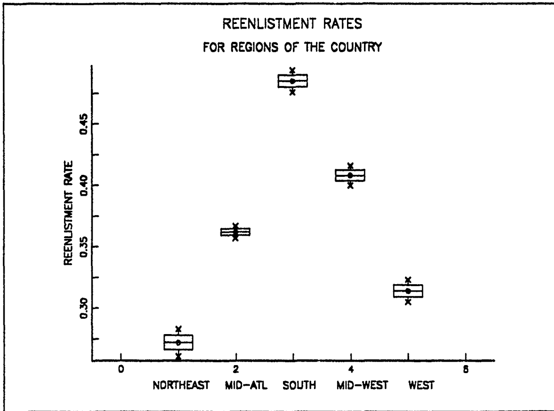
Figure 12. Reenlistment Rates for Regions of the Country
