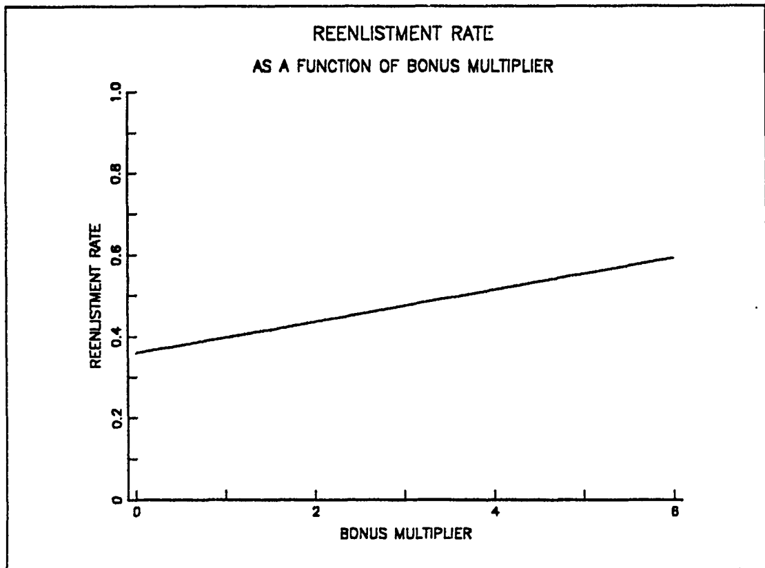
Figure 14. Plot of Bonus Level vs Reenlistment Probability
