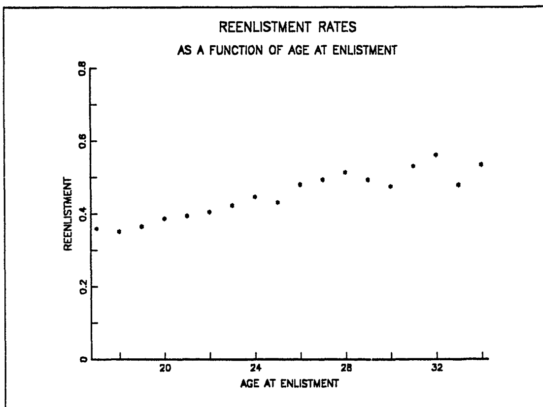
Figure 10. Reenlistment Rates for all MOS's, by Age at Enlistment
