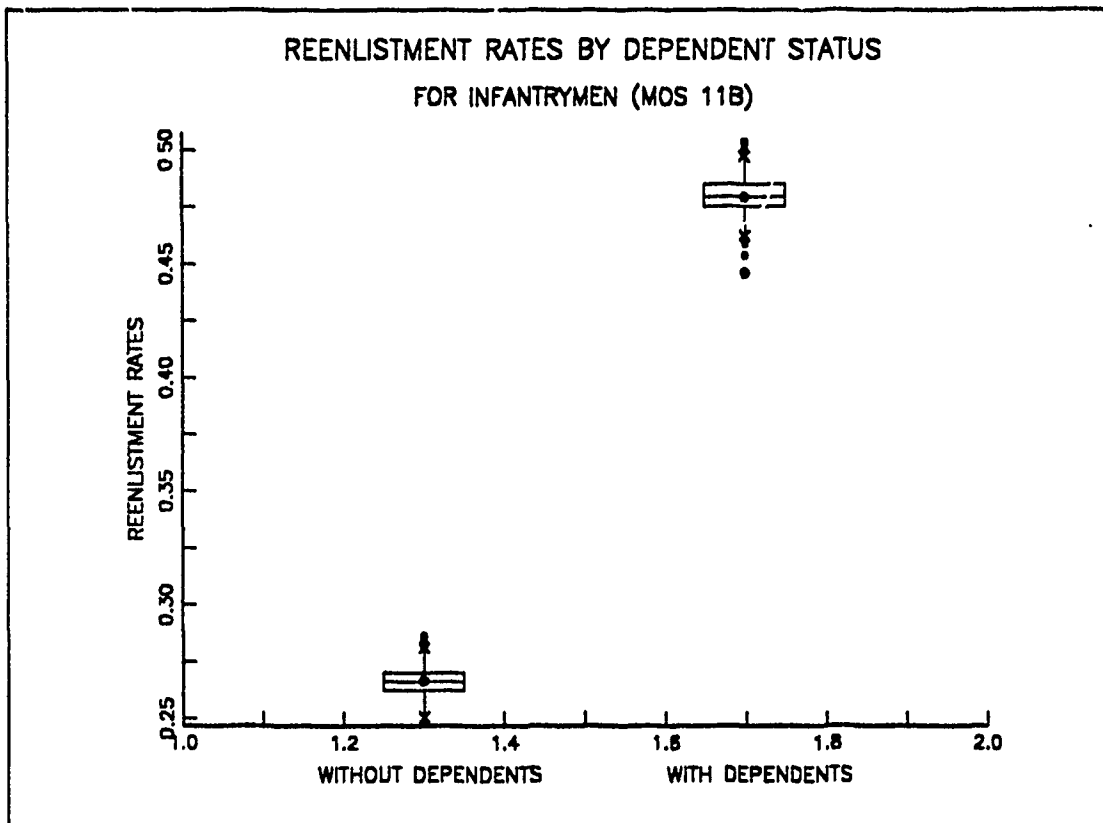
Figure 5. Reenlistment Rates for MOS 11B, Zone A by Dependent Status
