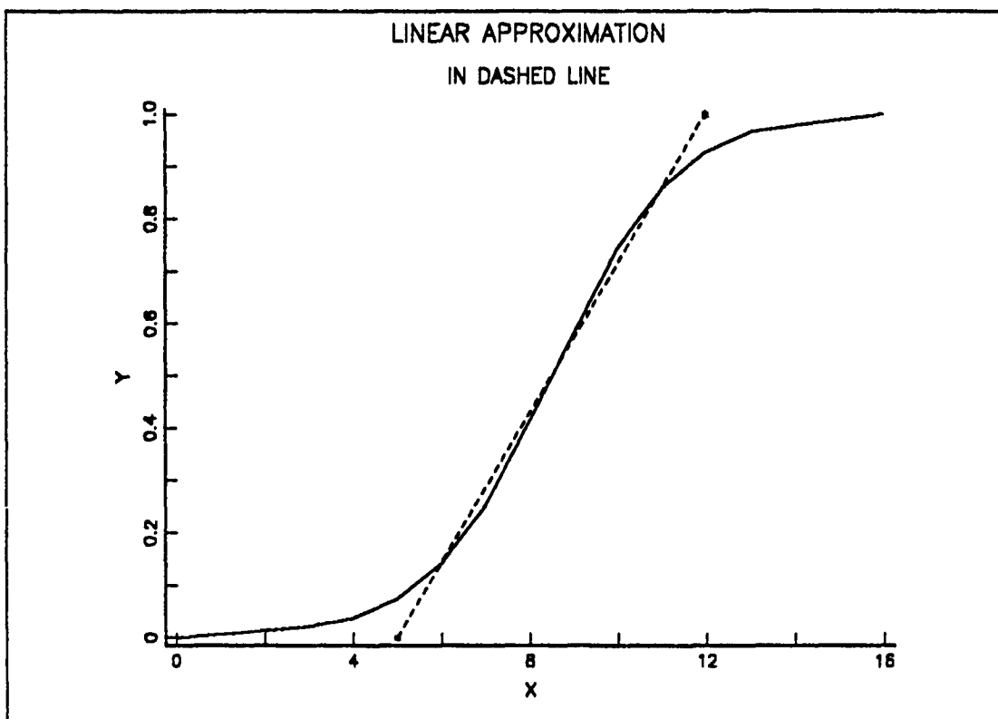
Figure 18. Linear Approximation to a Probability Function
