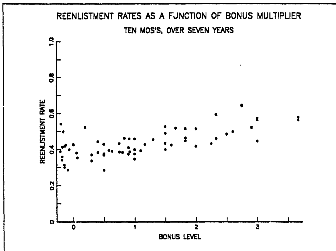
Figure 2. Yearly Reenlistment Rates for Ten MOS's Over Seven Years
