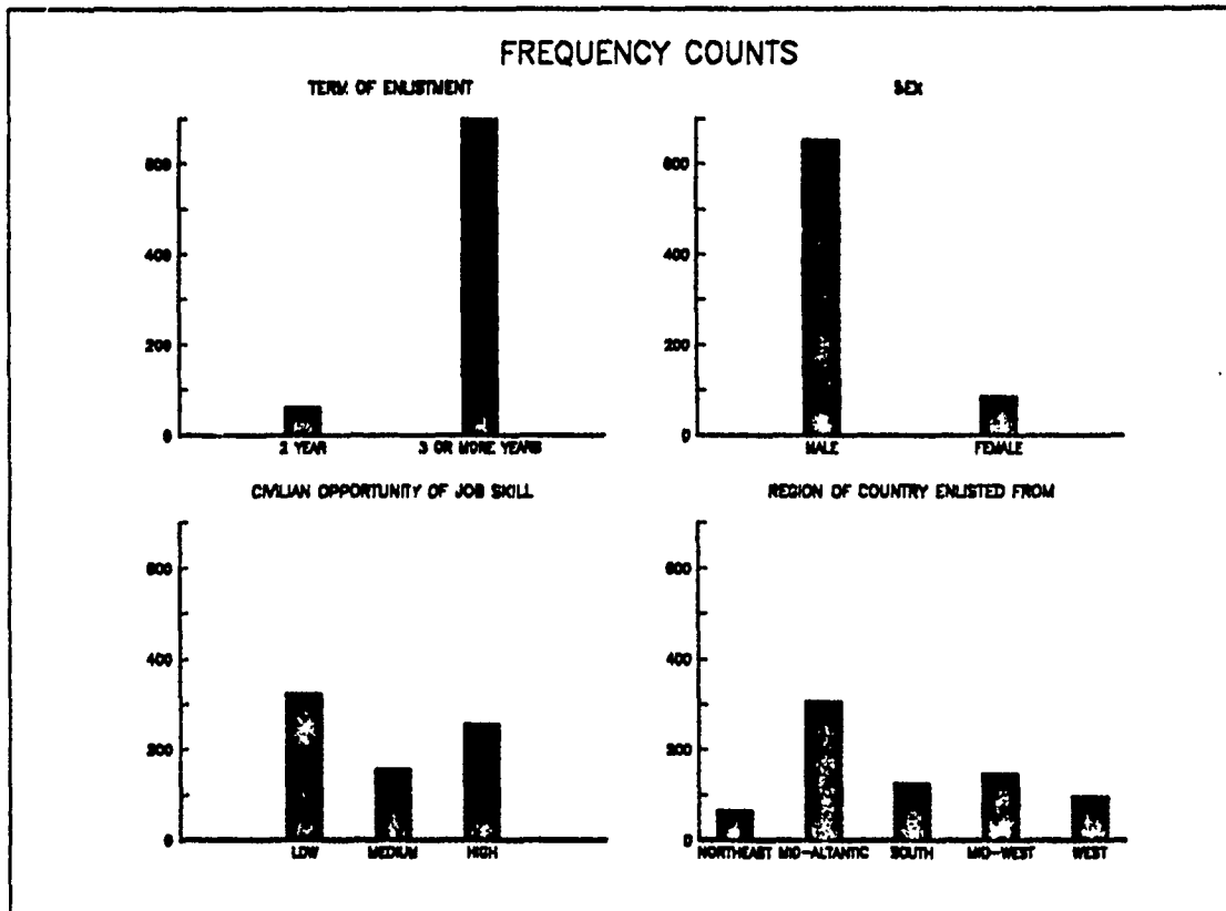
Figure 9. Frequency Counts For Selected MOS's
