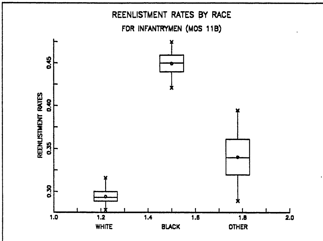
Figure 7. Reenlistment Rates for MOS 11B, Zone A by Race
