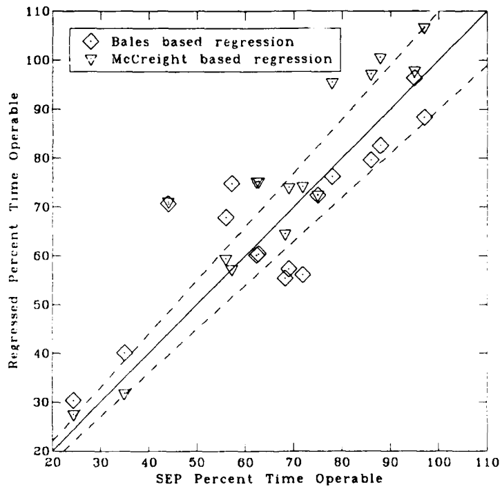
Fig. 7. Regressed PTOs based on Bales and McCreight variables compared with SEP PTO.
