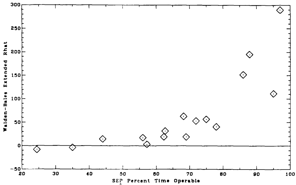
Fig. 5. Comparison of \hat{R}_e and PTO for representative fleet.
