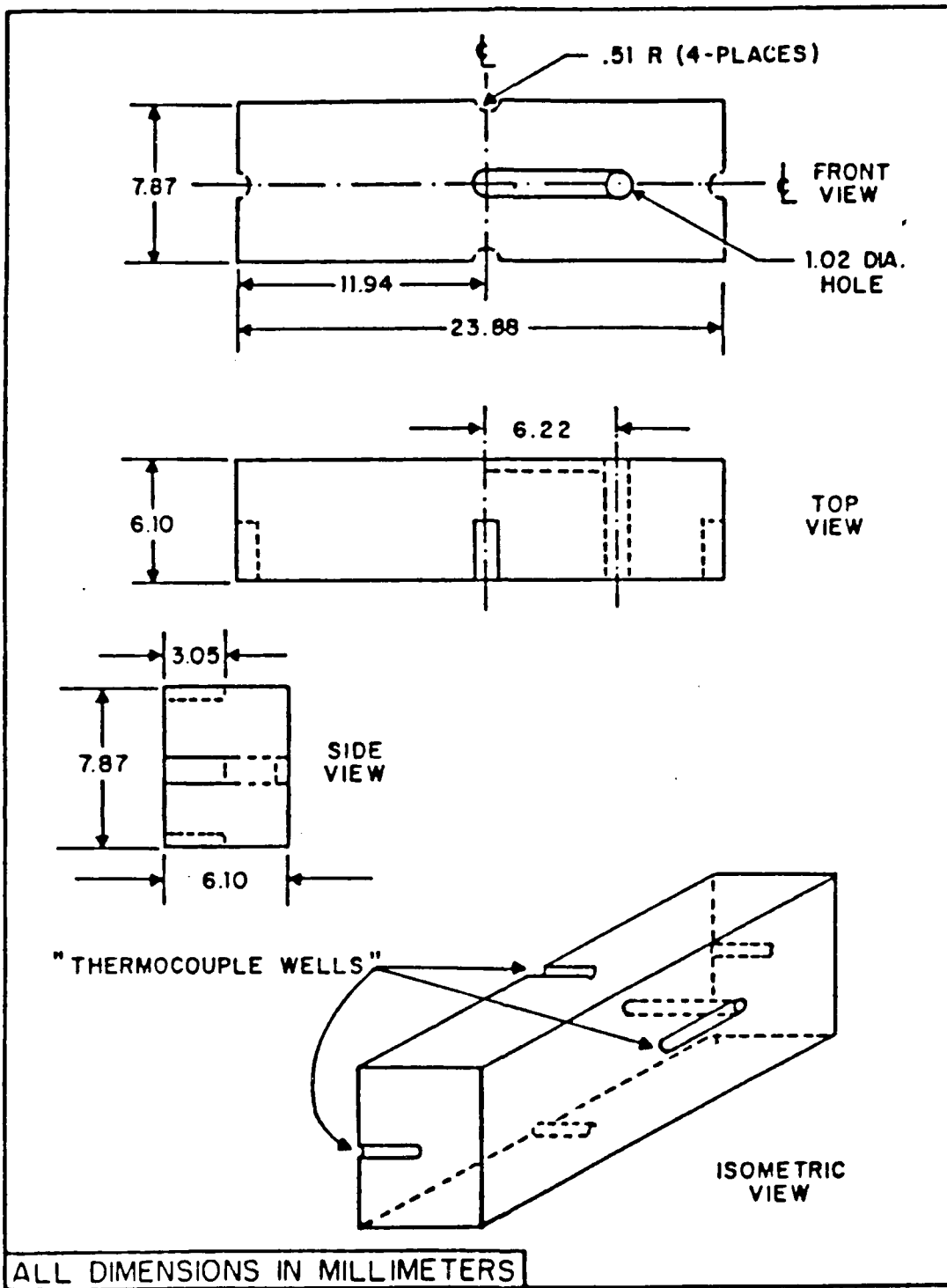
Figure 2.4 Heating Element and Thermocouple Locations
