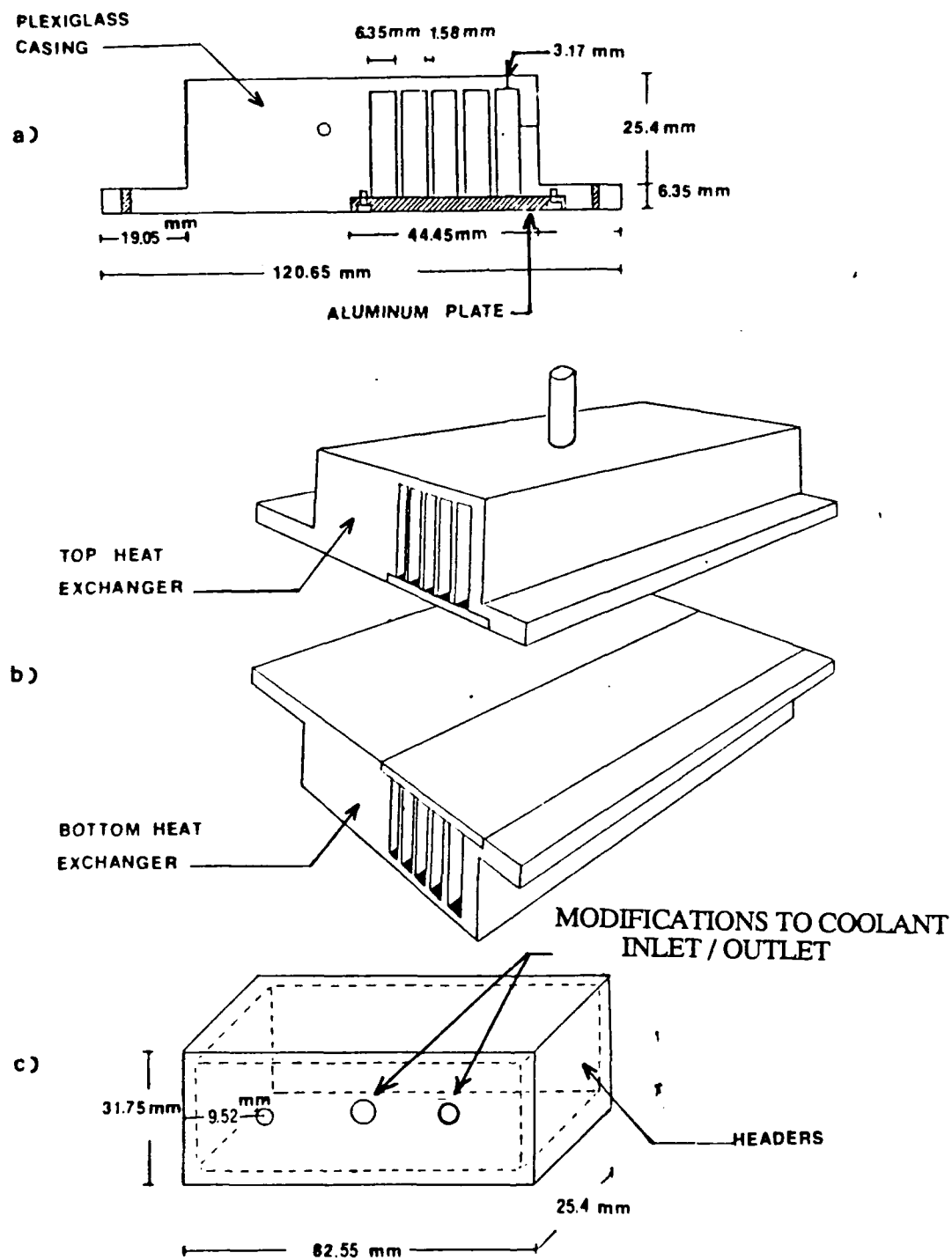
Figure 2.3 Heat Exchangers (a) Cross Sectional View; (b) Isometric View; (c) Inlet and Outlet Headers
