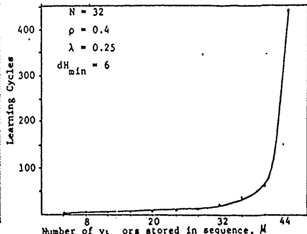
Fig. 2: Learning cycles needed for correct recall of a sequence of correlated vectors versus number of vectors, M in the sequence.
