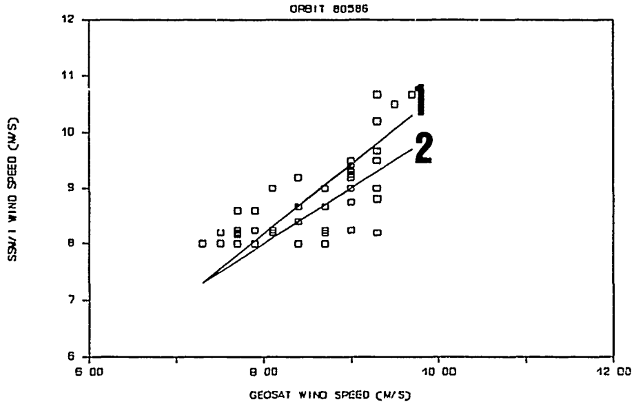
Figure 22 SSM/I vs. GEOSAT wind speed: orbit 80586. Line 1 represents an actual correlation of 0.935, while line 2 represents a reference correlation of 1.0.
