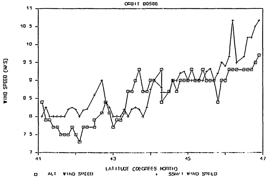
Figure 23 SSM/I vs. GEOSAT winds vs. latitude: orbit 8058(6).
