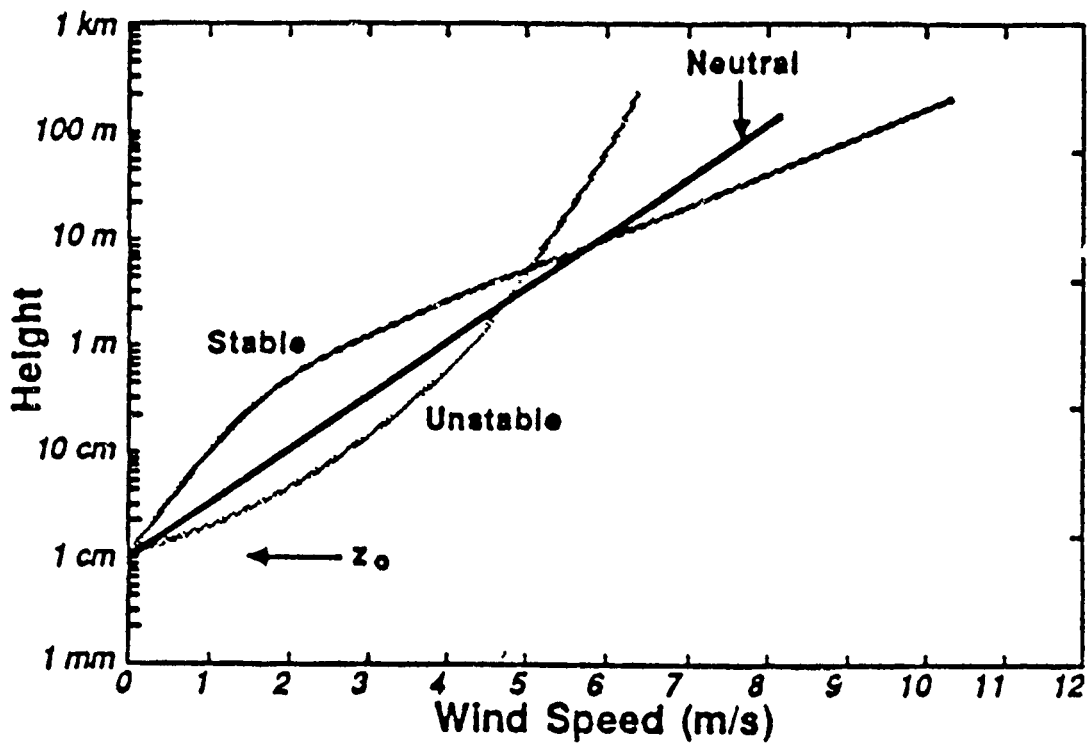
Figure 3 Typical wind speed profiles versus static stability in the surface layer.
