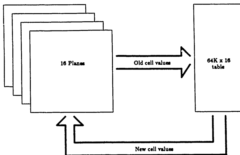
Figure 7.11: A layer of CAM-7, consisting of 16 plane-modules. As the planes are scanned, a stream of 16-bit cell values are sent as addresses to a 64K \times 16 lookup table—the 16-bit results are put back into the planes, as the new cell values.
