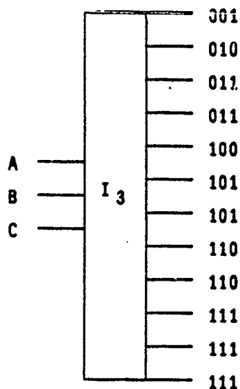
Figure 1.10: A 3 line bit-conserving demultiplexer
