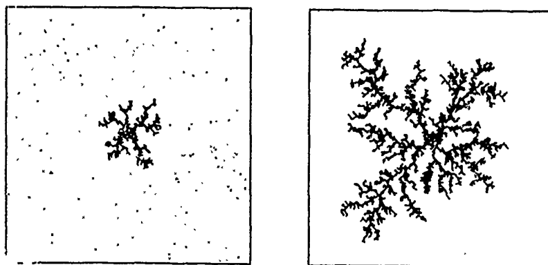
Figure 7.8: Dendritic growth by diffusion-limited aggregation. The process was started from a one-cell seed in the middle, and with a 10% density of diffusing particles.
