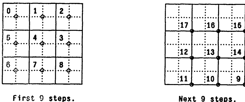
Figure 6.2: A 6×6 lattice with periodic boundaries. All 2×2 blocks in the solid partition are updated, and then all blocks in the dotted partition. Because of periodicity, 9 through 17 mark the centers of dotted blocks.
