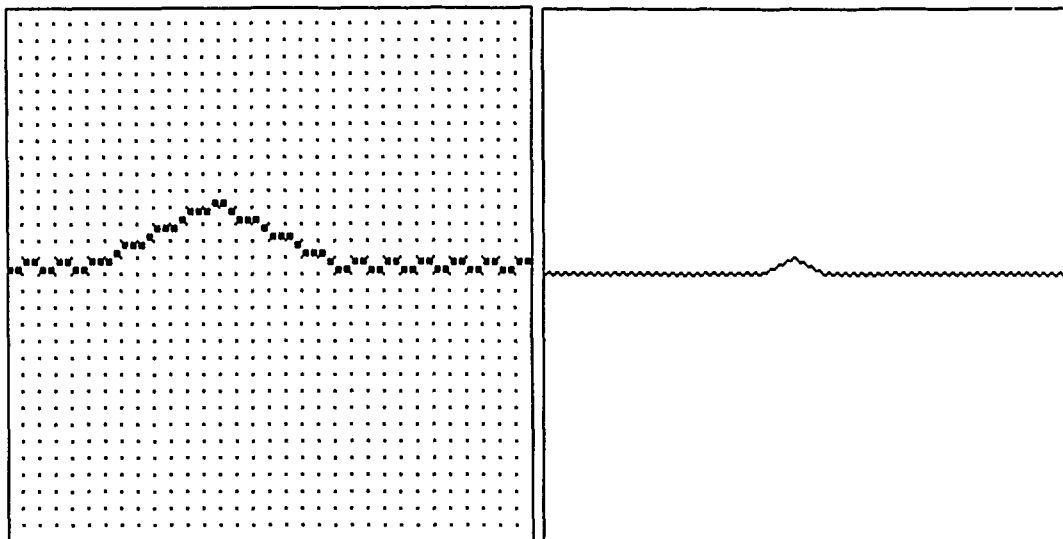
Figure 4.7: In (a) we have a closeup of part of the right-going wave shown in (b).
