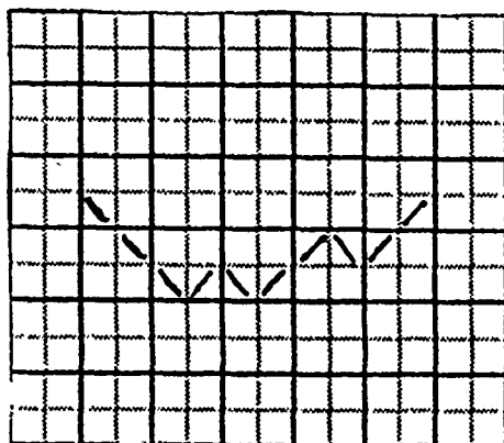
Figure 4.6: String corresponding to the sequence “\\\\//\\//.”
