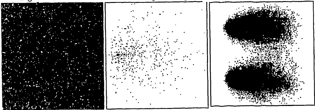
Figure 7.7: (a) The direction of drift is invisible if the fluid has uniform density. (b) Markers ejected by a smokestack diffuse in the fluid. (c) On a larger-scale simulation, the streamlines start becoming visible.
