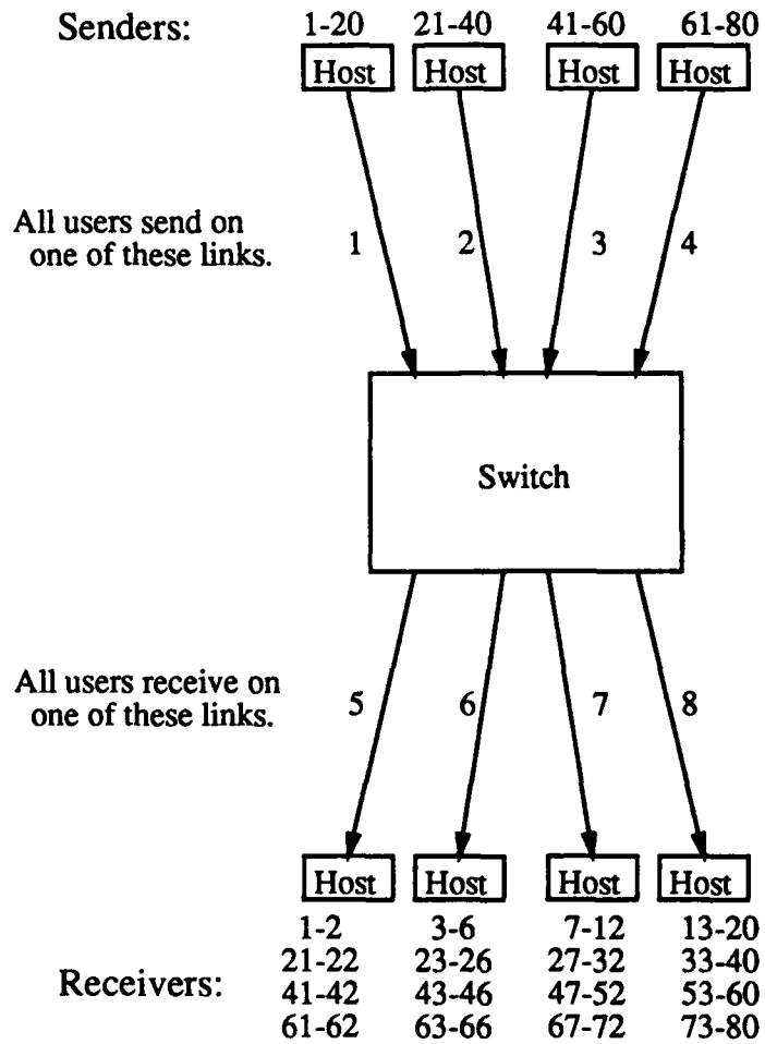
Figure 3-1: Mosely's Topology
