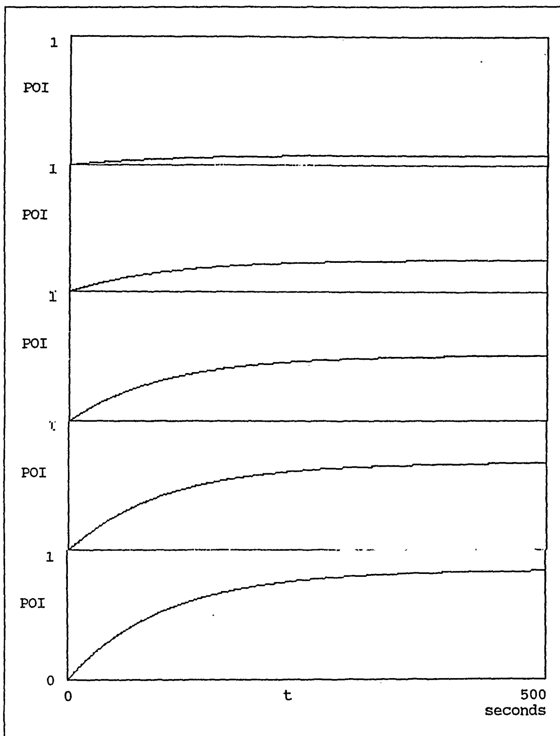
Figure 10. POIT plot(1): Intercept time with signal power variation: \beta = 0.01 , P_r = 10, 50, 100, 500, 1000 milliwatts
