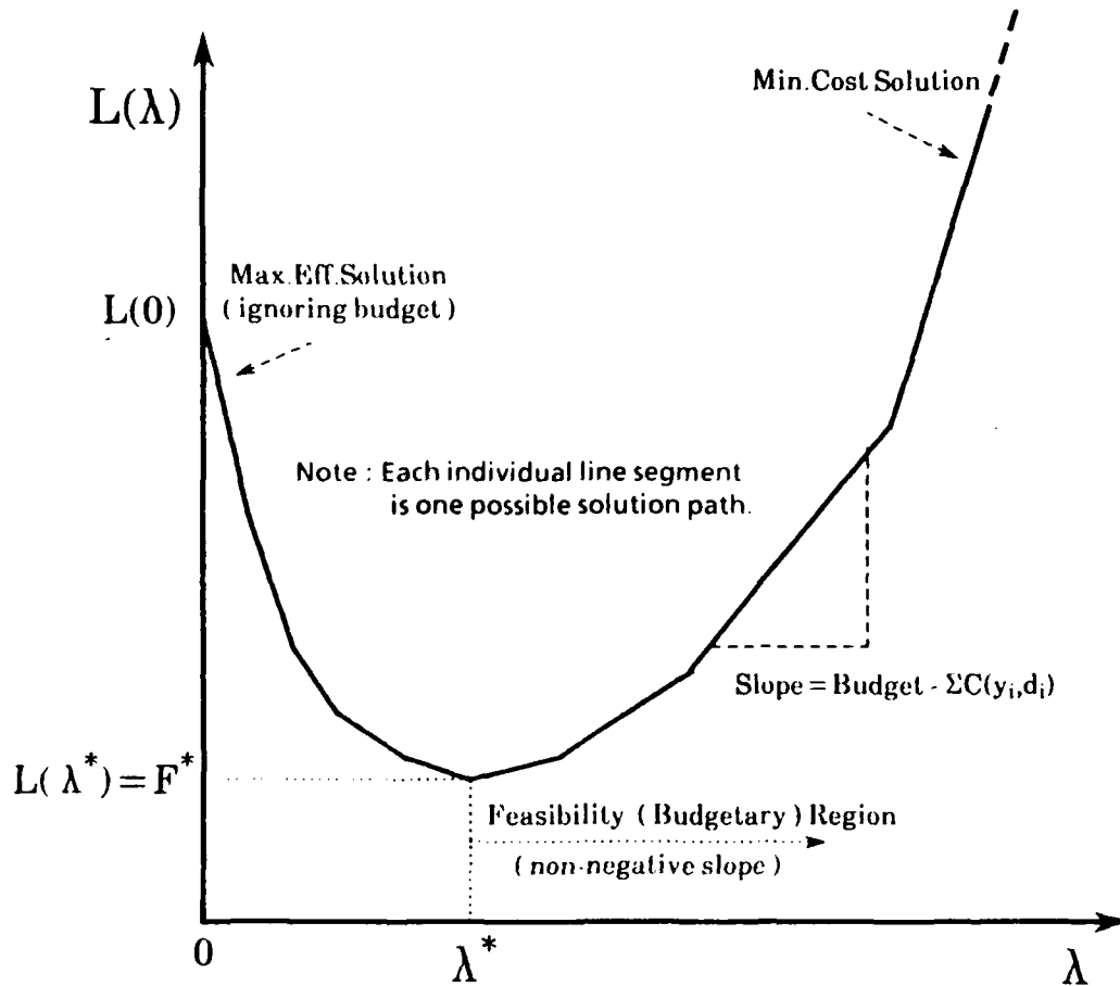
Figure 3.3: Lagrangian Function L(\lambda)
