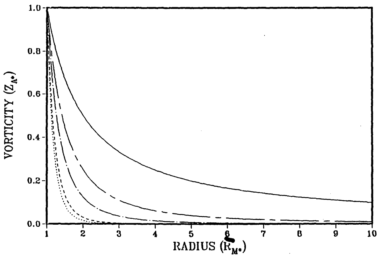
Fig. 3.2 Radial dependence of initial perturbation vorticity ( Z_A, \zeta_0^* ) for convection-induced ( k=2 , dot; k=1 , dash), motion-induced (chaindot), shear-induced (chaindash) and \beta -induced (solid) asymmetries.
