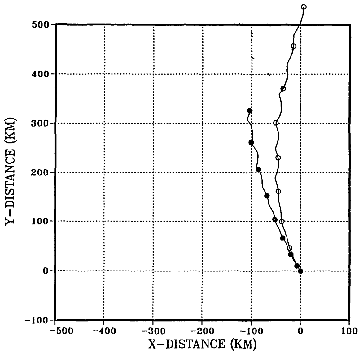
Fig. 5.12 Tracks and 6-hour positions predicted by the numerical model for \beta -induced TC propagation in an zonal current with linear anticyclonic shear of Z_e = -5.0 \times 10^{-6} s^{-1} using the symmetric initial TC wind profile of Fig. 5.9 with (open circles) and without (solid circles) BSAM-generated wavenumber one gyres.
