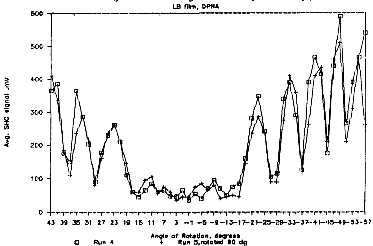
Fig. 2 Second harmonic signal vs. angle for Langmuir-Blodgett film.
