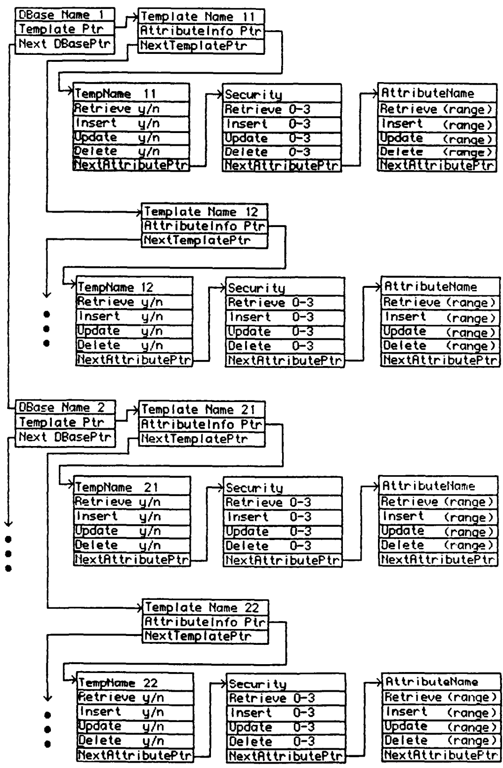
Figure 3.3 User Profile Linked-List Data Structure
