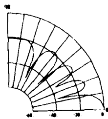
Figure 5. Sum beam pattern.
