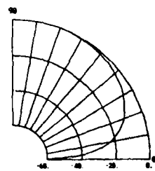
Figure 7. Difference beam pattern.
