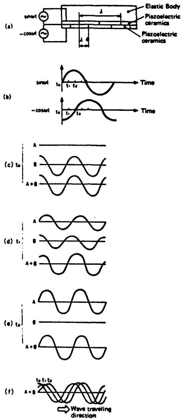
Figure 12. a) Two plates of alternately poled segmented piezoelectric materials are offset and attached to an elastic body. b) Each plate is excited with sinusoidal driving signals 90 degrees out of phase. c) d) and e) Deformation along the body at various time steps. f) A wave of deformation moves along the body over time. [Panasonic].
