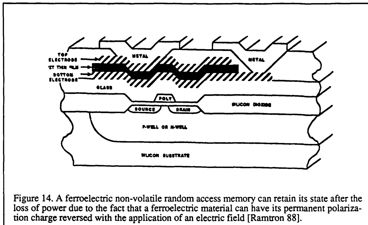
Figure 14. A ferroelectric non-volatile random access memory can retain its state after the loss of power due to the fact that a ferroelectric material can have its permanent polarization charge reversed with the application of an electric field [Ramtron 88].
