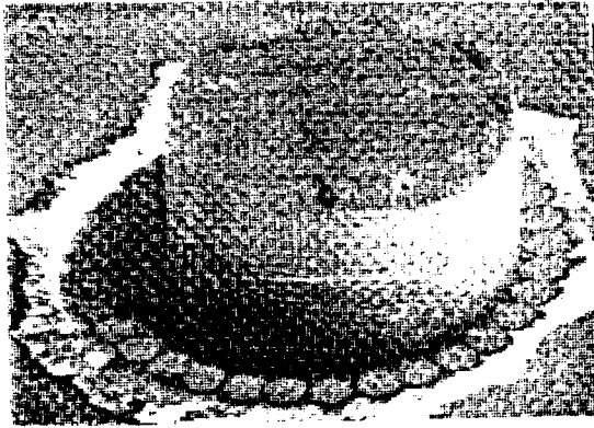
Figure 7. A wobble motor, extruded as opposed to silicon micromachined, uses electrostatic forces applied by the surrounding stator electrodes to force the rotor to "wobble" much like a harmonic gear [Jacobsen et al 89]. Reprinted by permission.
