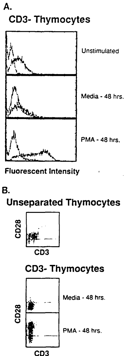
Figure 2. The CD28 surface Ag is inducible on CD3 - thymocytes. A. CD3 - thymocytes were negatively selected by immunoadsorption using magnetic beads and then cultured with media alone, or media plus PMA (10 ng/ml) for 48 h. Cells were stained with anti-CD28-PE mAb either before culture or after 48 h in culture. Cells stained with PE-labeled nonspecific mouse Ig (Mslg) served as negative controls. B. CD3 - thymocytes selected and stimulated as above were also analyzed by two-color flow cytometry to verify that they remained CD3 - in culture. Staining of unseparated and cultured cells was done with anti-CD3-FITC plus anti-CD28-PE. Cursor placement was determined by simultaneous staining of cells with FITC- and PE-labeled Mslg. In both panels fluorescent intensity is displayed on a 3-log scale.
