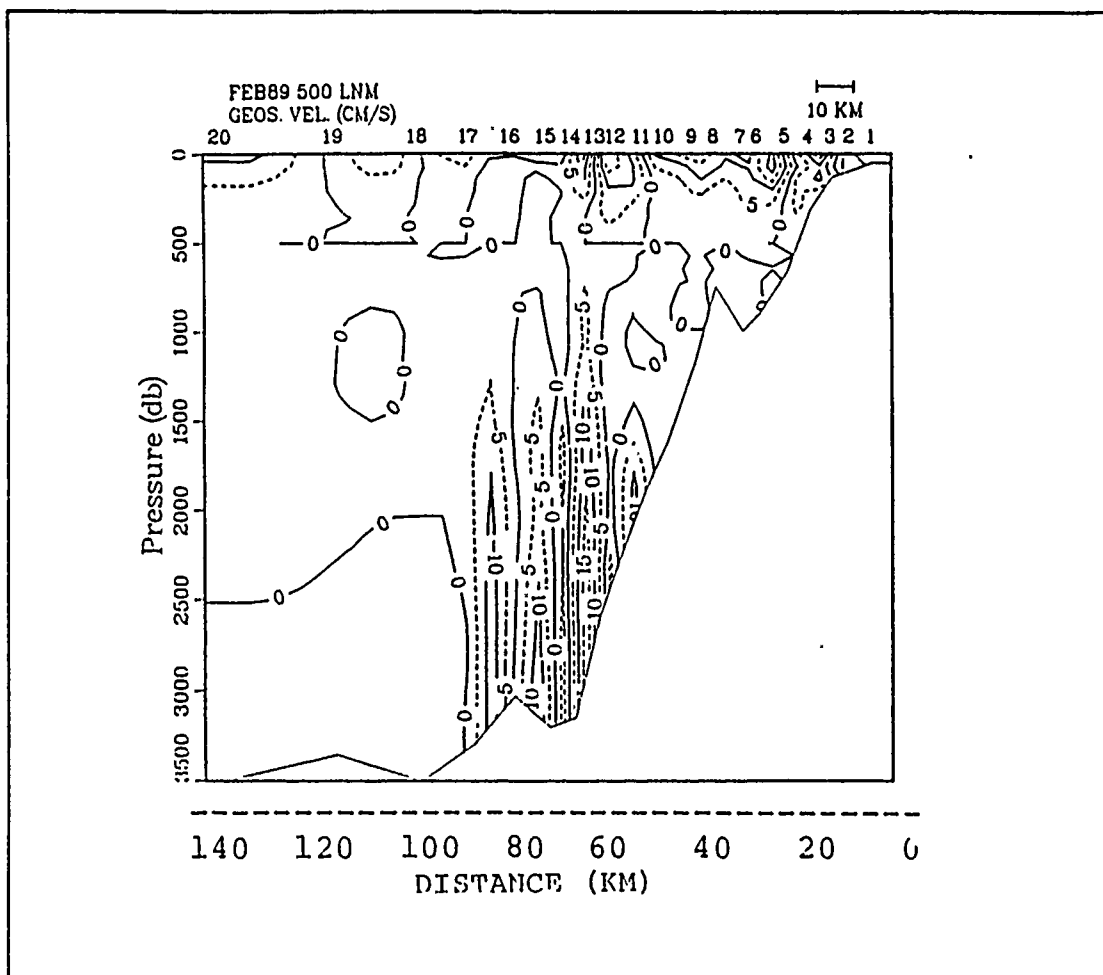
Figure 10. Geostrophic velocity (0-3500 m): meridional (N-S) velocity component. Level of no motion is 500 m. Positive values indicate poleward flow, negative values equatorward flow. Contour interval is 5 cm/s.
