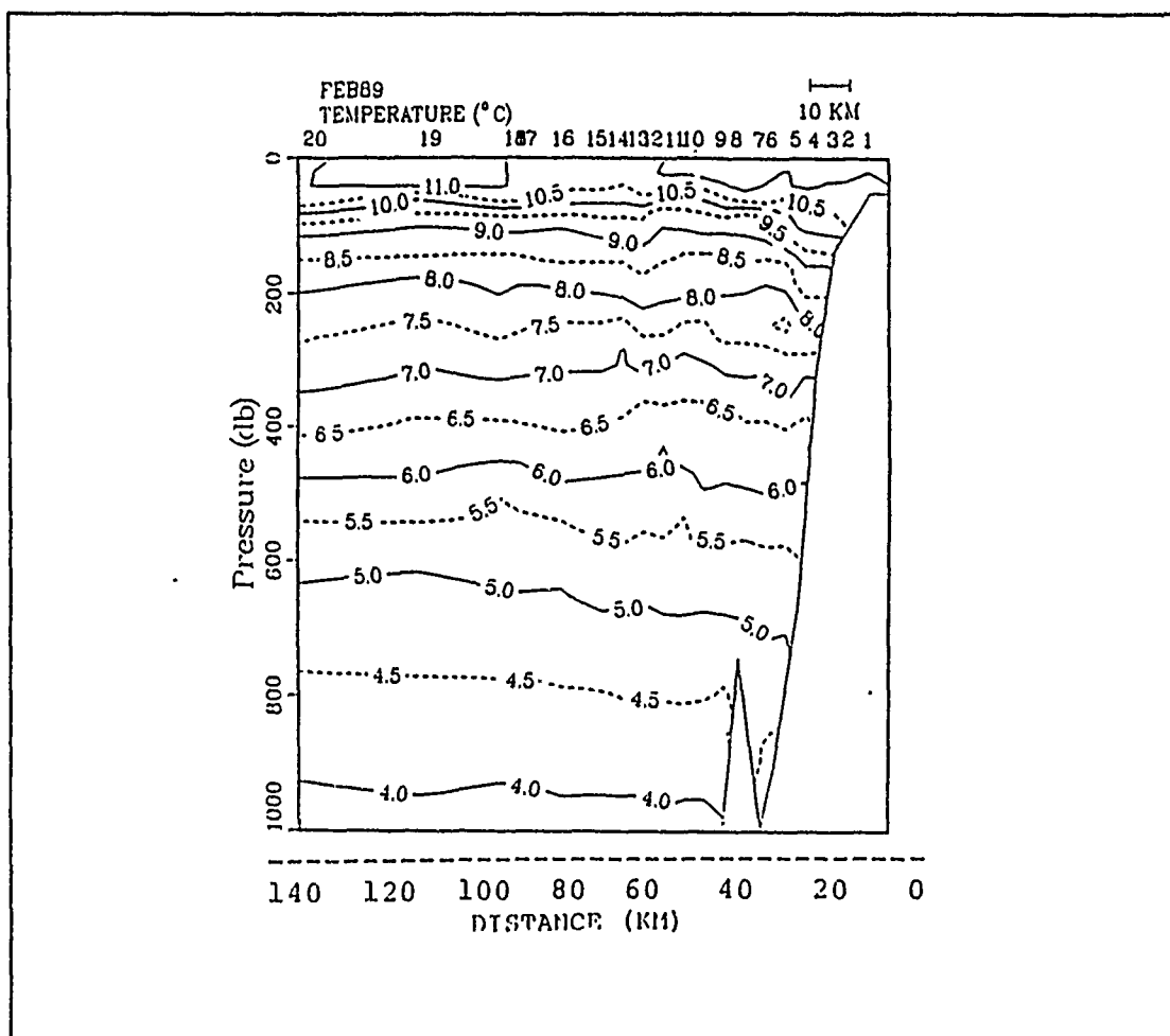
Figure 12. CTD Temperature (0-1000 m): the temperature field along the Point Sur Transect. Contour interval is .5°C.
