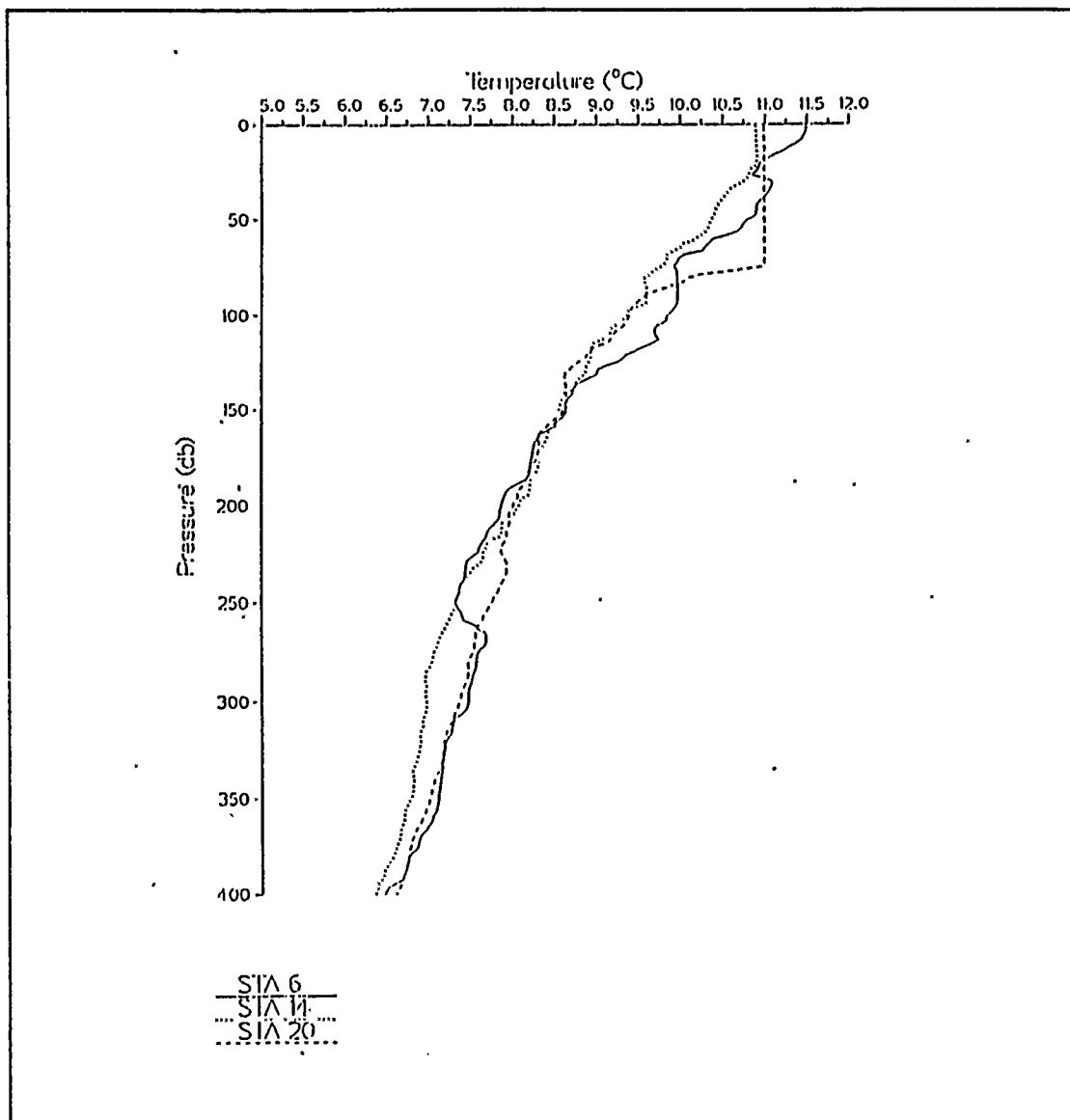
Figure 13. Temperature profiles from 3 CTD stations (°C): profiles from CTD stations 6,14,20 indicate how the mixed-layer deepens further offshore.
