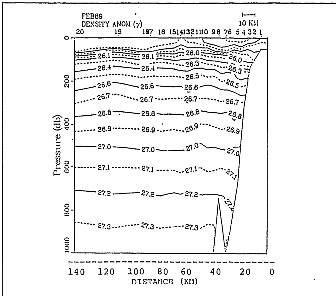
Figure 17. Density anomaly ( \gamma ) cross-section of Pt. Sur Transect: contour interval is .1 kg/m 3 .
