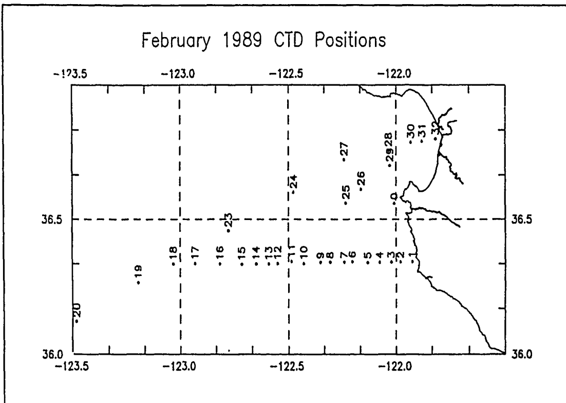
Figure 2. Point Sur Transect: these are the locations of CTD stations 1-20 along the transect.
