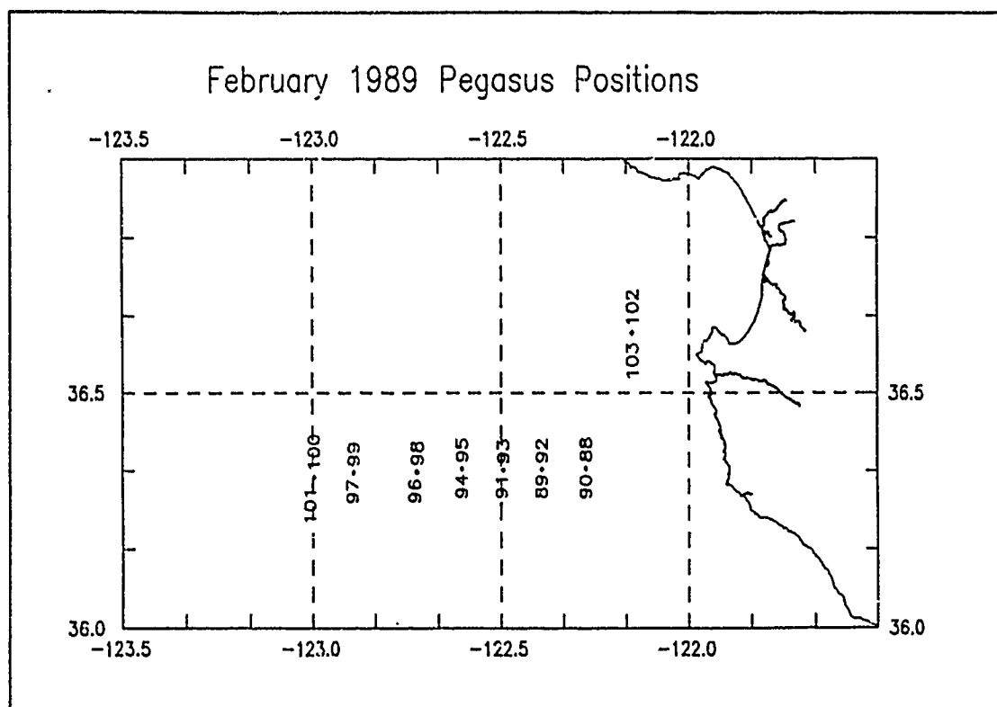
Figure 1. Pegasus cast locations along 36°20'N: station C1 (casts 88,90) is 33 km offshore. Station C7 (casts 100,101) is 100 km offshore.
