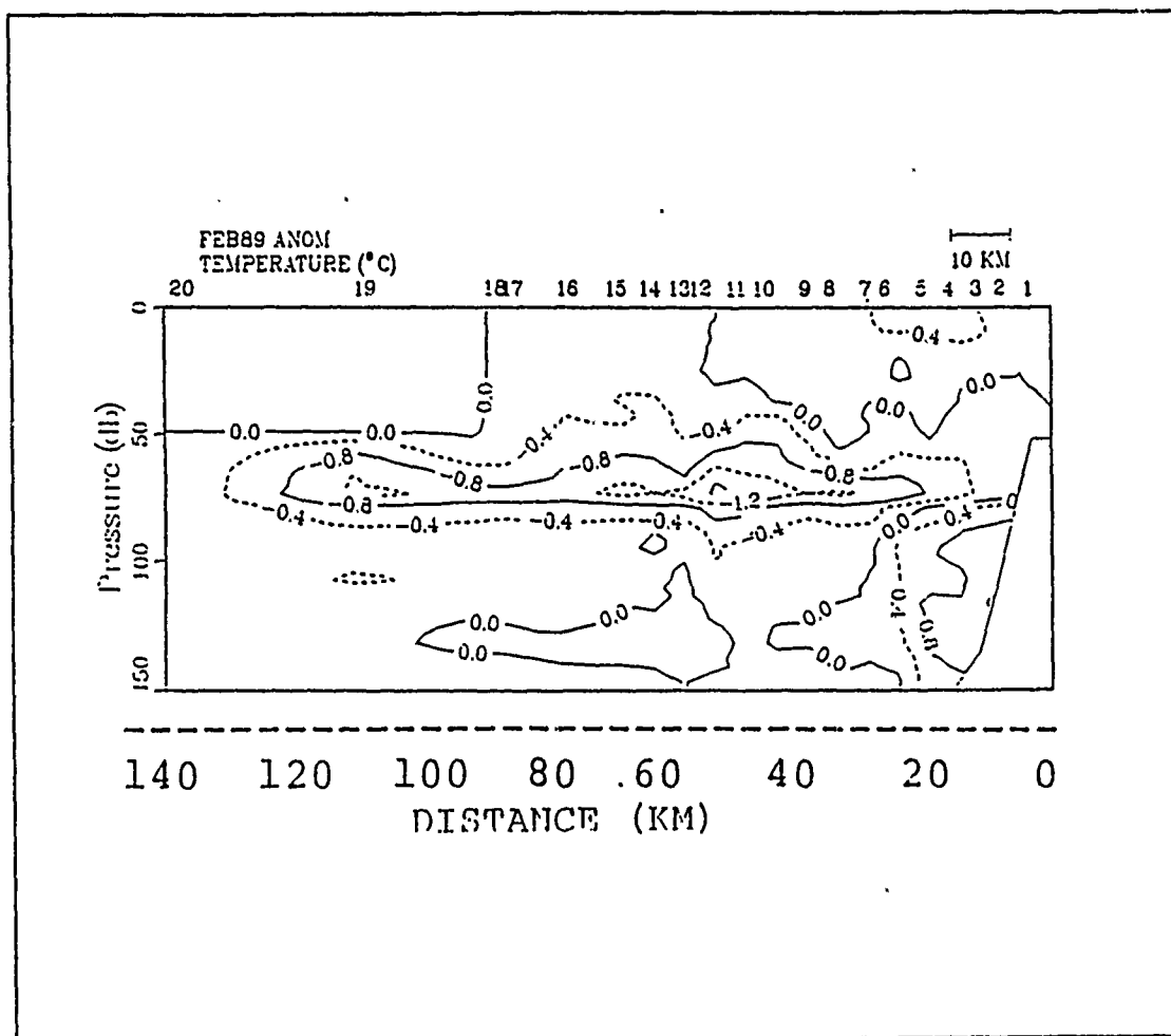
Figure 14. Temperature anomalies( ^{\circ}\text{C} ): the temperature field as seen by CTD is normalized by the temperature profile at station 20. The long band of negative temperature anomaly from 50-80 m is due to the fact that the mixed layer deepens further offshore. Contour interval is .4^{\circ}\text{C} .
