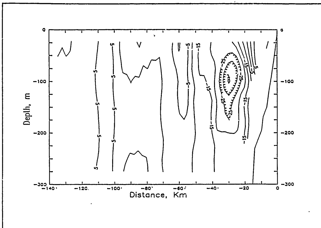
Figure 8. ADCP cross-section of U (20-280 m): zonal (E-W) velocity component. Positive values indicate onshore flow, negative values offshore flow. Contour interval is 5 cm/s.
