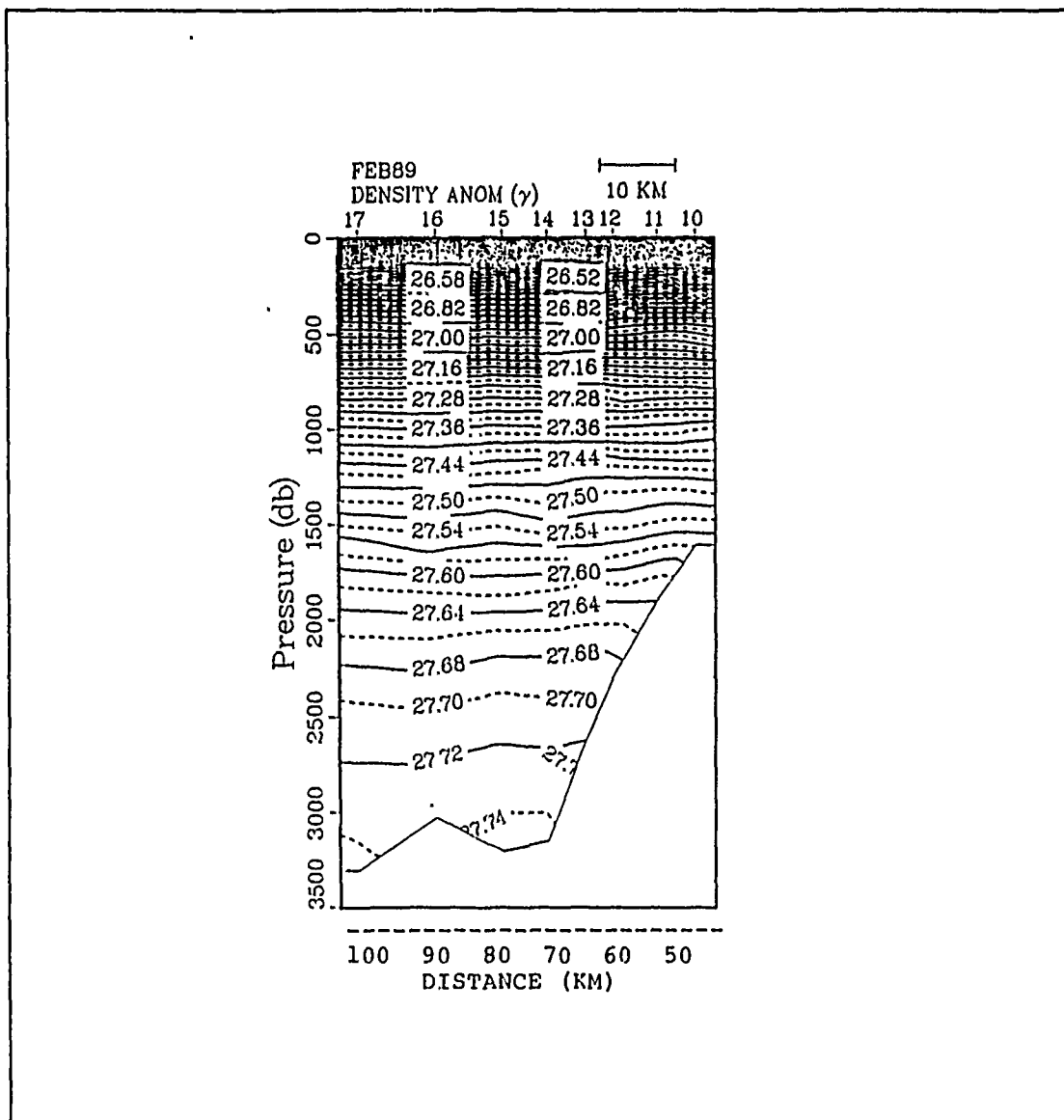
Figure 18. Density anomaly ( \gamma ) cross-section: this section covers CTD stations 10-17, corresponding to the banded shear zone. There is considerable wave structure in the deep isopycnals, especially 27.70. Note the severe slope of the 27.74 isopycnal at the bottom, which supports the large (10-15 cm's) geostrophic velocities evident in the earlier figures at the bottom. The contour interval is .02 kg/m 3 .
