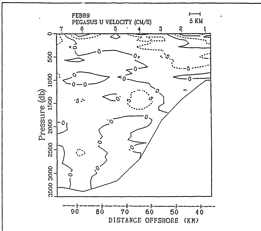
Figure 5. Pegasus cross-section of U (0-3500 m): zonal (E-W) velocity component. Positive values indicate onshore flow, negative values offshore flow. Contour interval is 5 cm/s.
