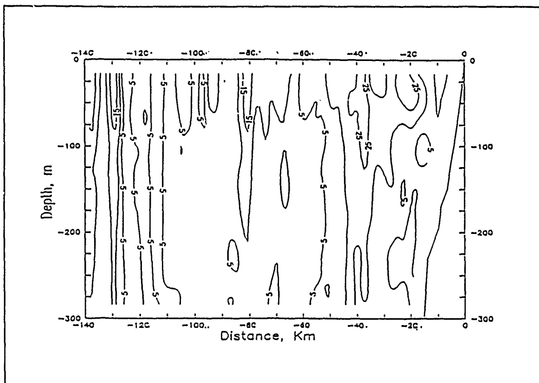
Figure 7. ADCP cross-section of V (15-290 m): meridional (N-S) velocity component. Positive values indicate poleward flow, negative values equatorward flow. Contour interval is 5 cm/s.
