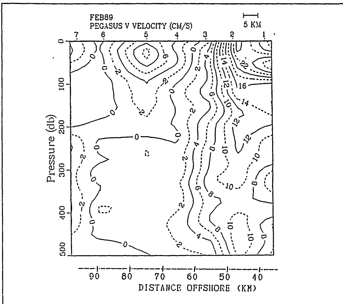
Figure 4. Pegasus cross-section of V (0-500 m): meridional (N-S) velocity component. Positive values indicate poleward flow, negative values equatorward flow. Contour interval is 2 cm/s.
