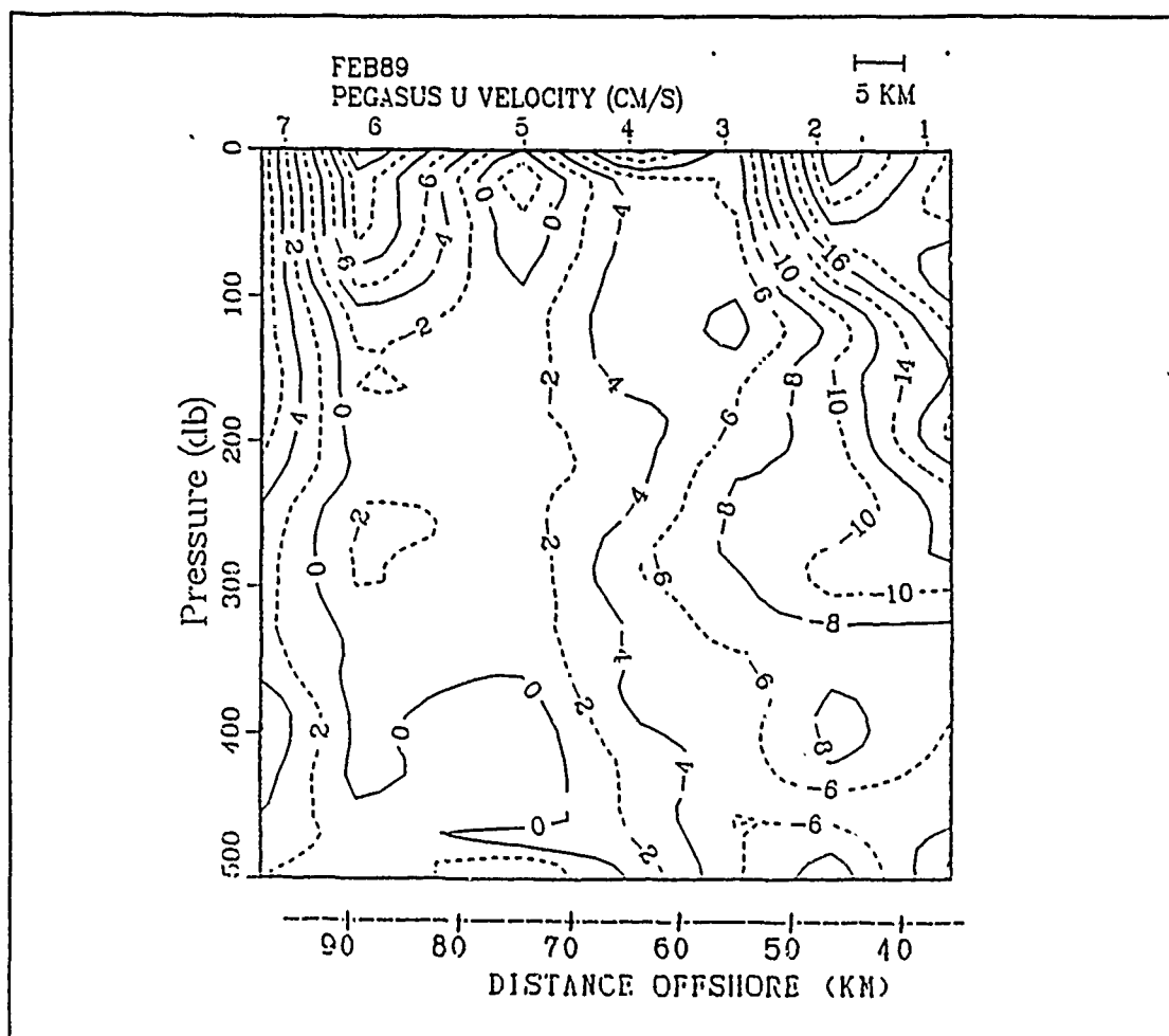
Figure 6. Pegasus cross-section of U (0-500 m): zonal (E-W) velocity component. Positive values indicate onshore flow, negative values offshore flow. Contour interval is 2 cm/s.
