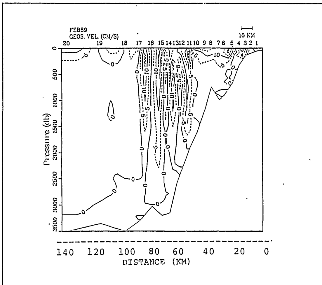
Figure 9. Geostrophic velocity(3500 m): LNM is the deepest common point between adjacent stations. Note the 200 m ridge present at station 8. Contour interval is 5 cm/s.
