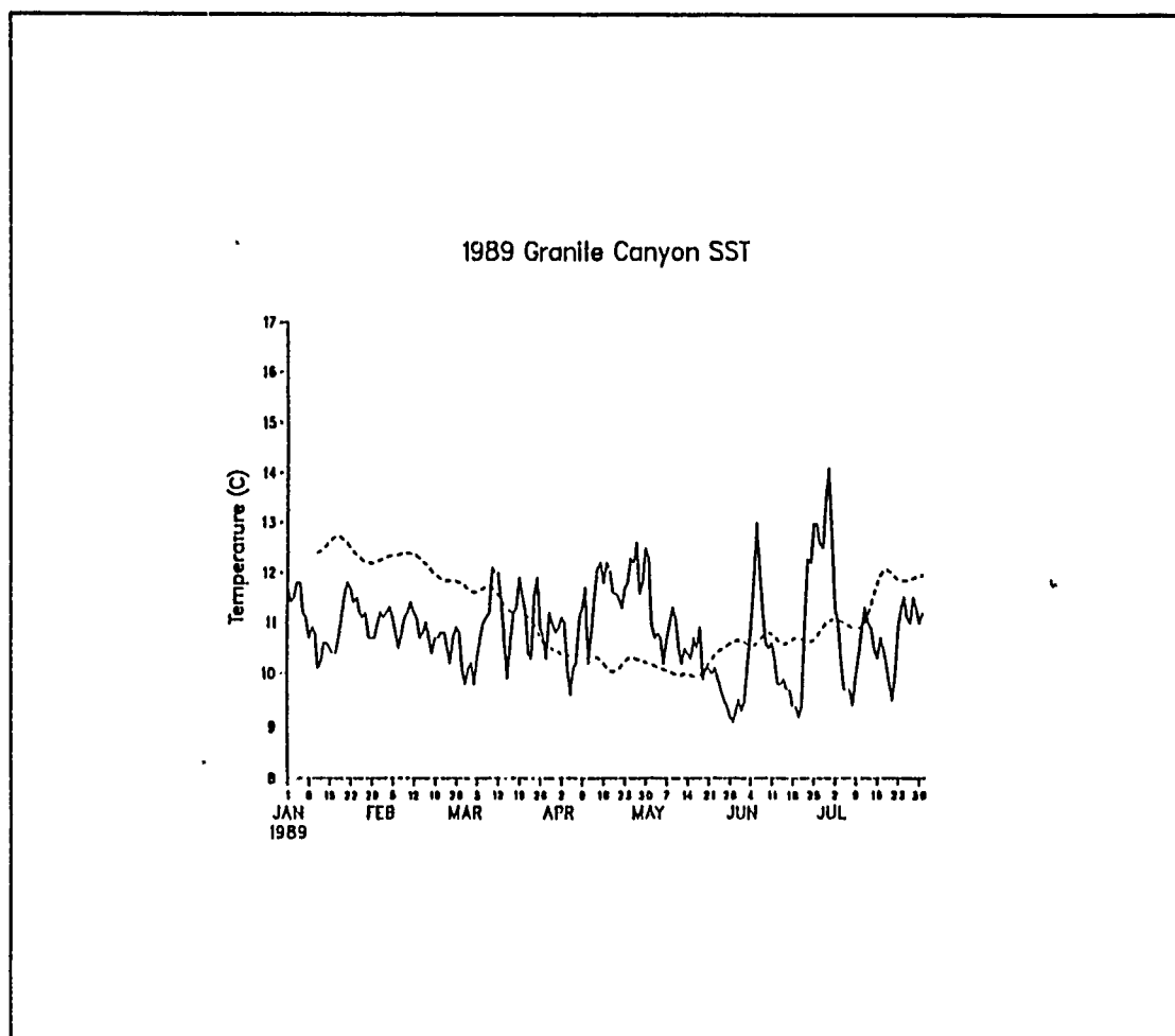
Figure 15. 1989 Granite Canyon SST( ^{\circ}\text{C} ): sea-surface temperatures observed at Granite Canyon (near Point Sur. Solid line is 1989; dashed line is 15-year average.
