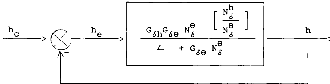
Figure 8-18 Simplified Block Diagram for Altitude Hold System
