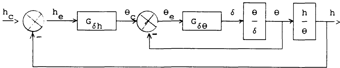
Figure 8-17 Block Diagram for Altitude Hold Autopilot
