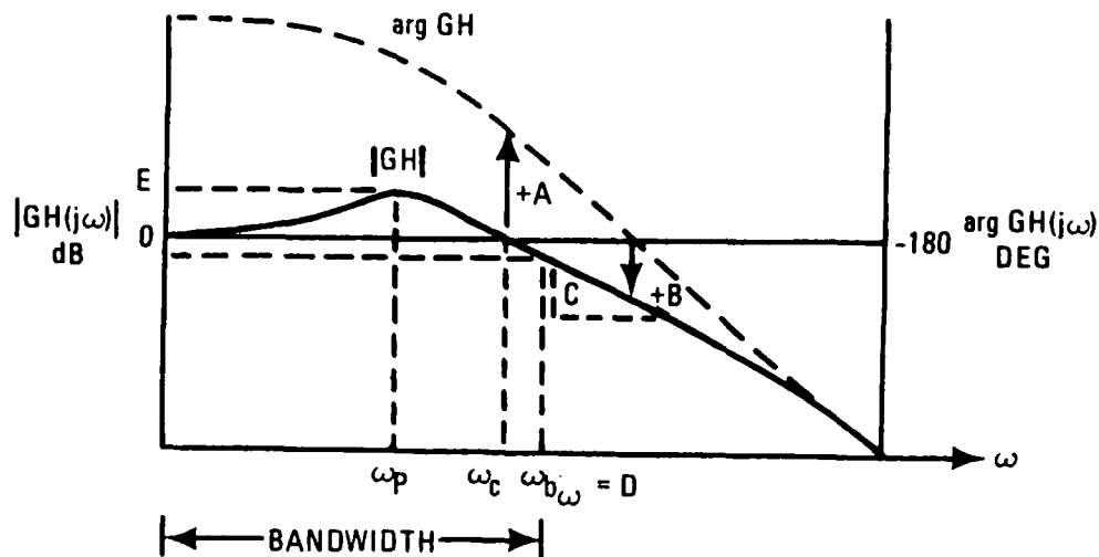
Figure 7-2 Bode Plot Criteria
