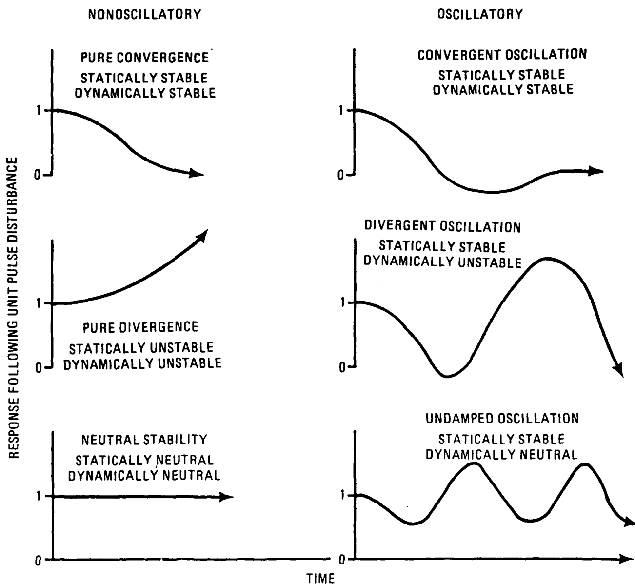
Figure 5-2 Illustration of Stability Options
