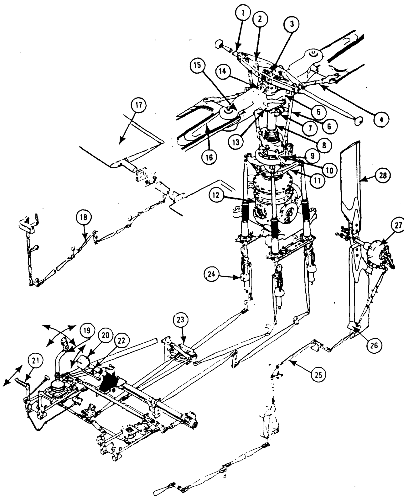
Figure 6-1 Mechanical Flight Control System From Reference 27
