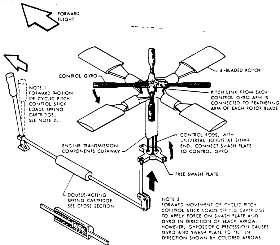
Figure 6-3 Lockheed Rigid-Rotor Control System From Lockheed Brochure
