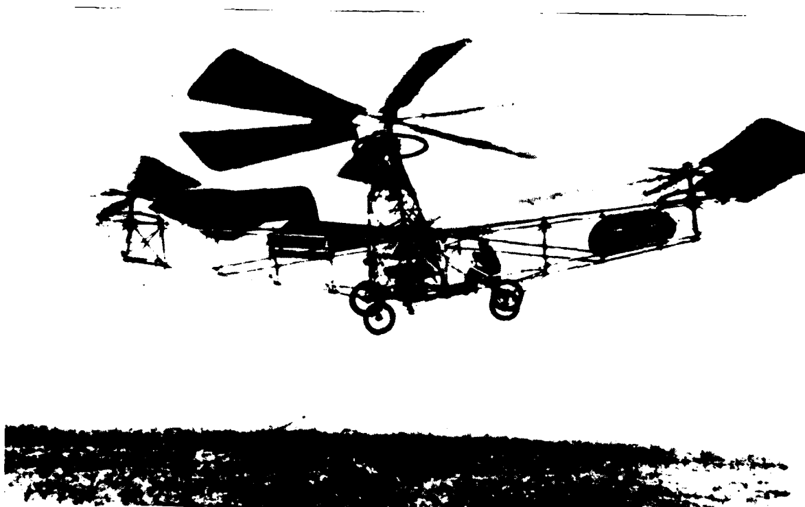
Figure 2-1 de Bothezat Helicopter Courtesy American Helicopter Society (AHS)
