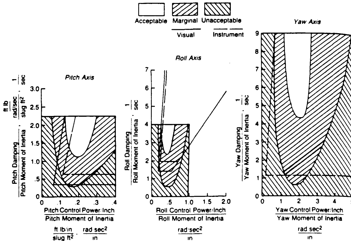
Figure 6-7 Damping and Control Power for Acceptable Handling Qualities (From Reference 11)
