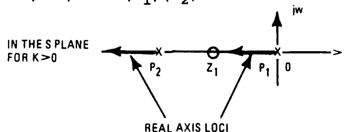
Figure 7-1 Root Locus Plot Showing Real Axis Loci
