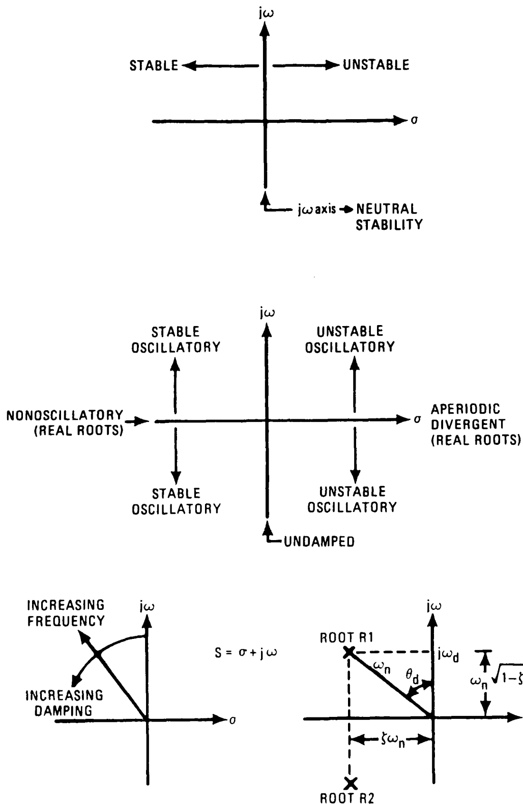
Figure 5-3 Effect of Root Location on Stability in the S Plane
