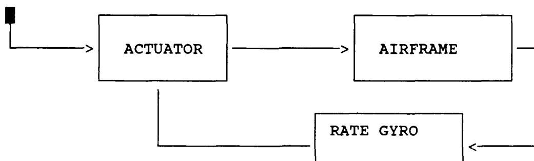
Figure 6-4 Functional Block Diagram of SAS
