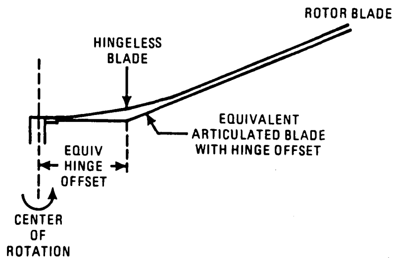
Figure 3-3 Sketch Showing Hingeless Rotor Hub and Equivalent Articulated Blade Representation of a Hingeless Blade
