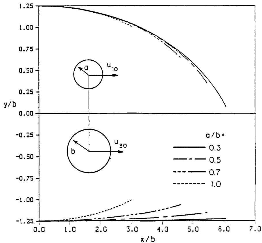
Figure 19. Trajectories of two spheres moving initially parallel to each other with \rho_2/\rho = 0.39 , x_{10}/b = x_{30}/b = 0 , x_{20}/b = -x_{40}/b = 1.25 , u_{10} = u_{30} = 1 , and u_{20} = u_{40} = 0 .
