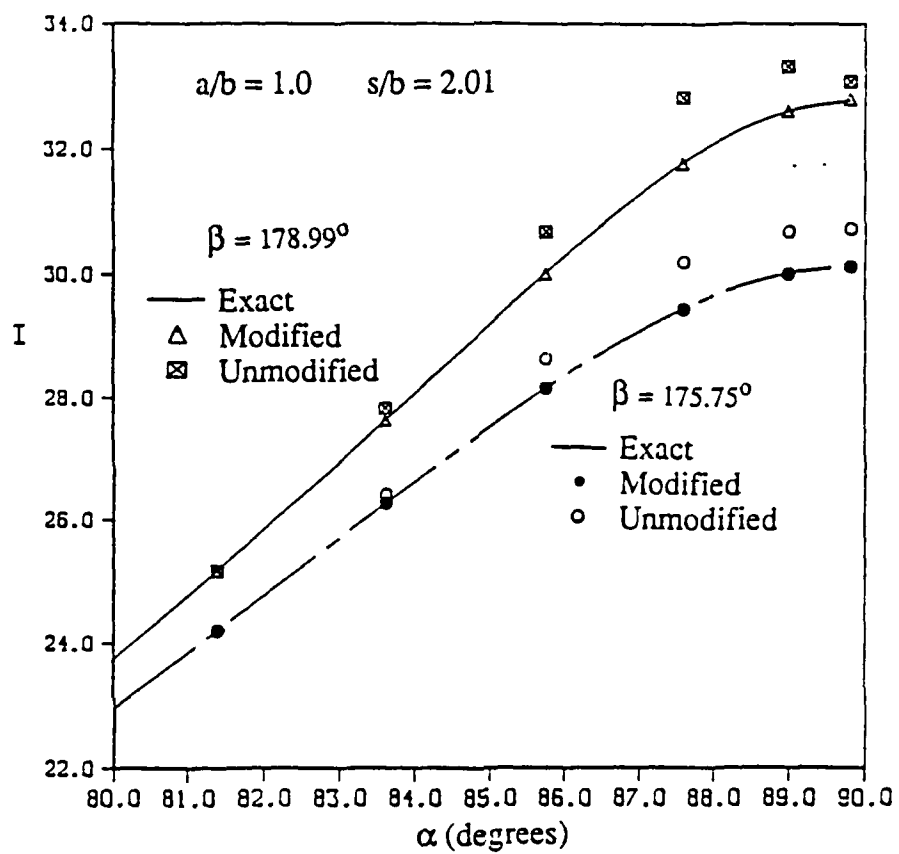
Figure 8. Comparison of numerical result of integral I (51) obtained with and without rotating coordinates.
