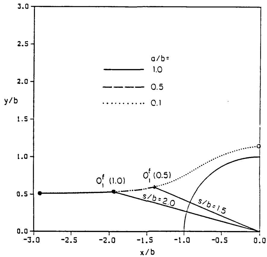
Figure 13. Trajectories of a moving sphere with various radius ratios.
