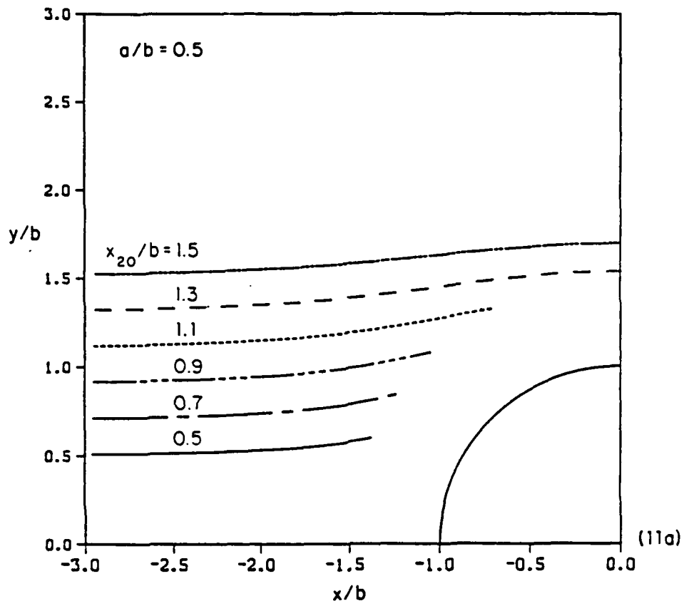
Figure 11. Trajectories of a moving sphere with x_{10}/b = -20 , u_{10}/U_0 = 1 , u_{20}/U_0 = 0 , and \rho_2/\rho = 0.89 .
