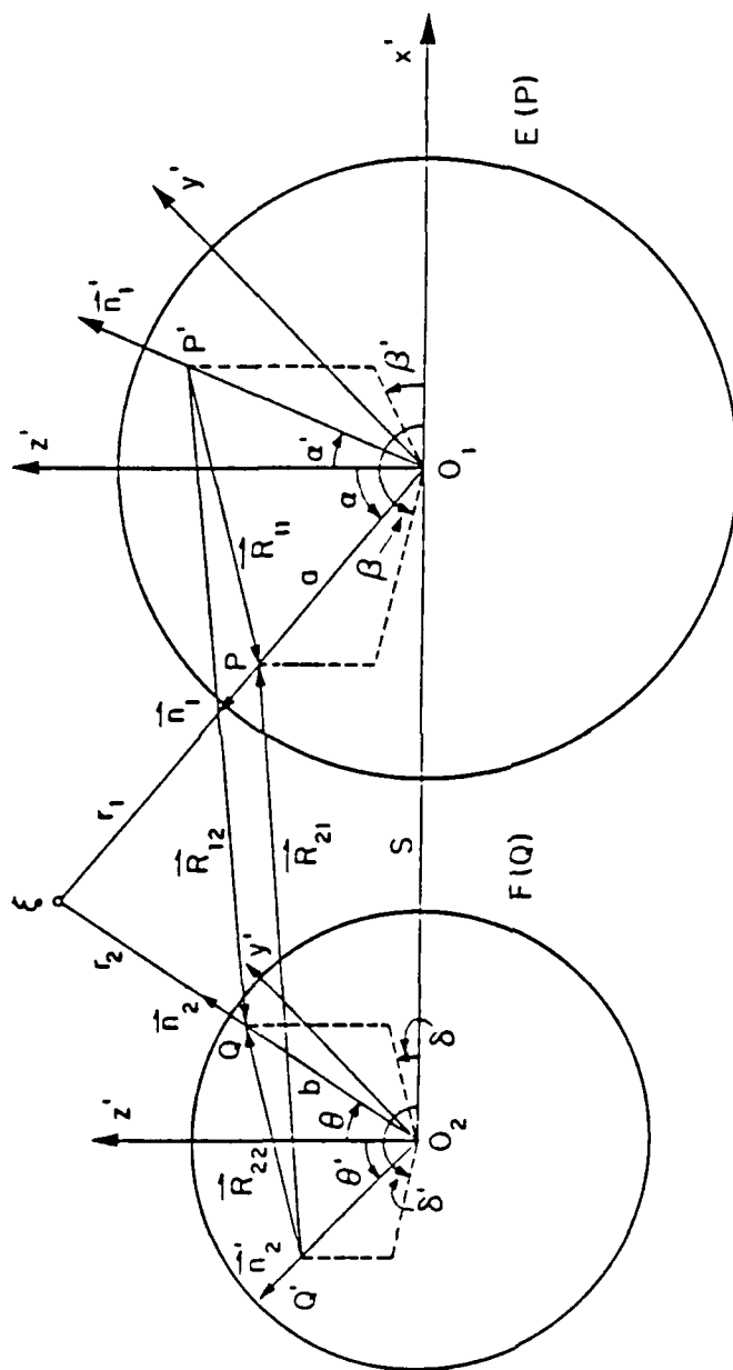
Figure 4. Surface integration of source distributions on spheres 1 and 2.
