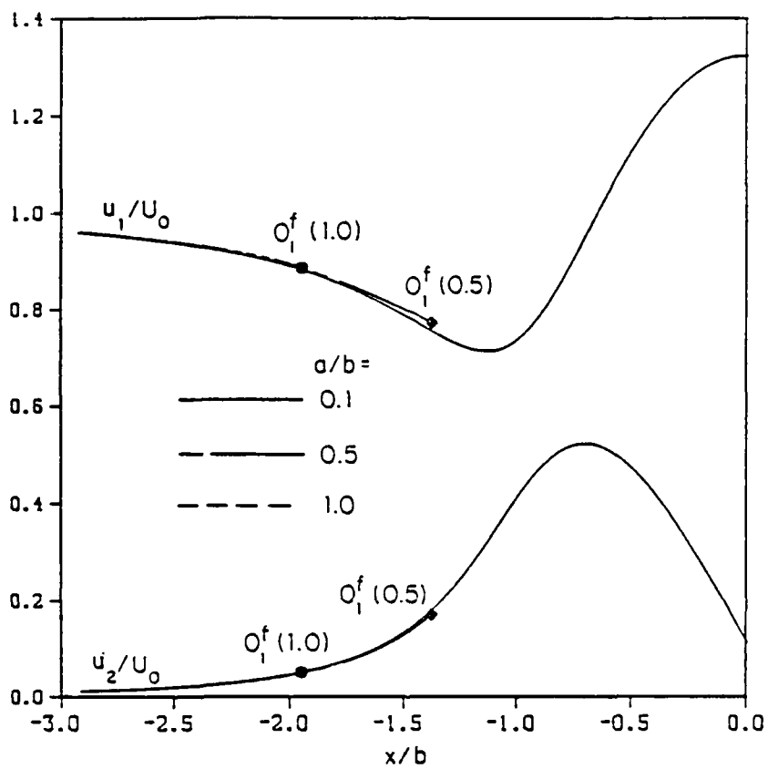
Figure 12. Velocity components u_1 and u_2 of a moving sphere with various radius ratios.
