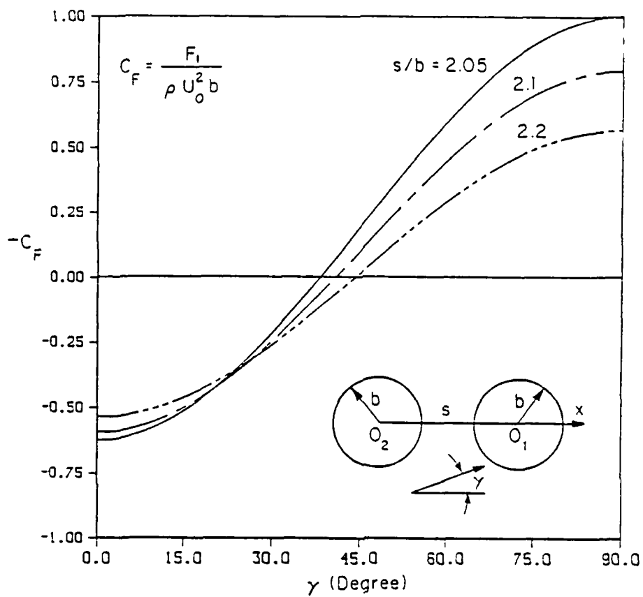
Figure 15. Dependence of interaction forces on the direction of a uniform flow.
