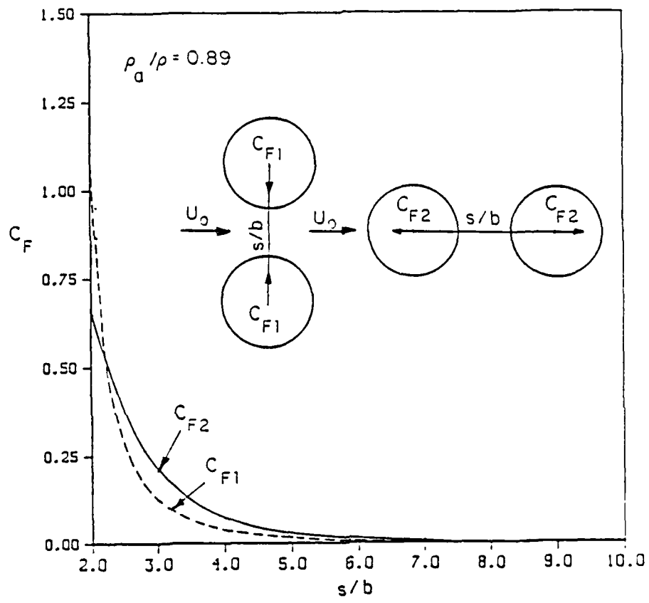
Figure 17. Interaction force between two equal spheres ( a/b=1 ) versus the separation distance s/b .
