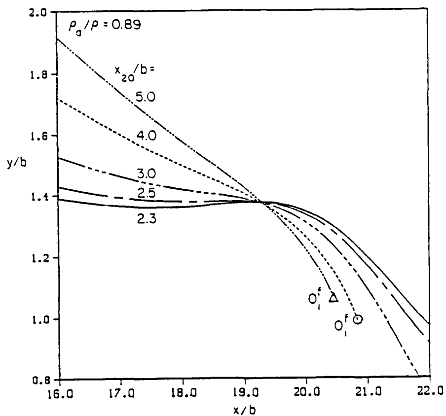
Figure 14. Trajectories of a moving sphere with radius a affected by another sphere with radius b , a/b=0.1 , \rho_a/\rho = 0.89 .
