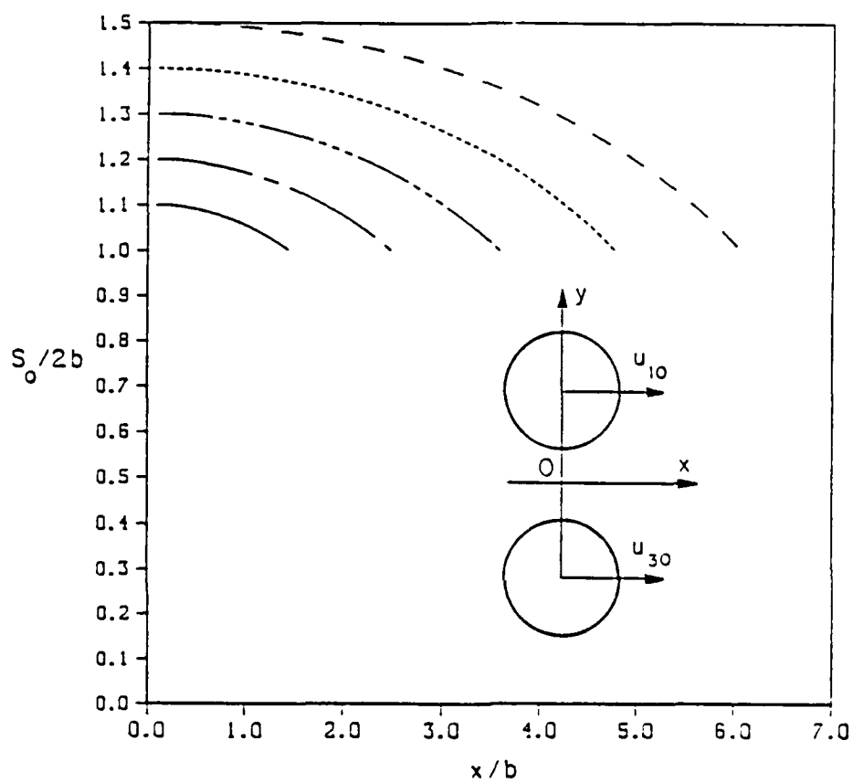
Figure 16. Trajectories of two equal spheres ( a/b=1 ) moving initially perpendicular to their centerline in a stationary fluid with \rho_x/\rho = 0.89 , a/b=1 , x_{10}/b = x_{30}/b = 0 , u_{10} = u_{30} = 1 , and u_{20} = u_{40} = 0 .
