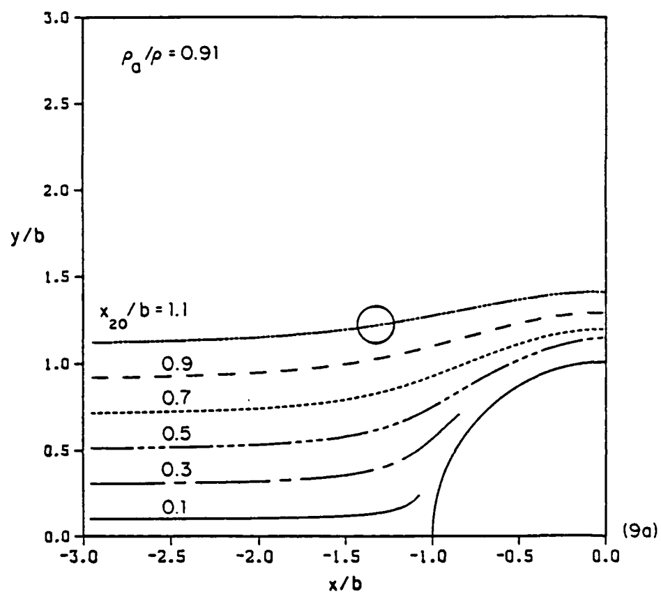
Figure 9. Trajectories of a moving sphere in different fluids with a/b=0.1 , u_{10}/U_0=1 , u_{20}/U_0=0 , and x_{10}/b=-20 .
