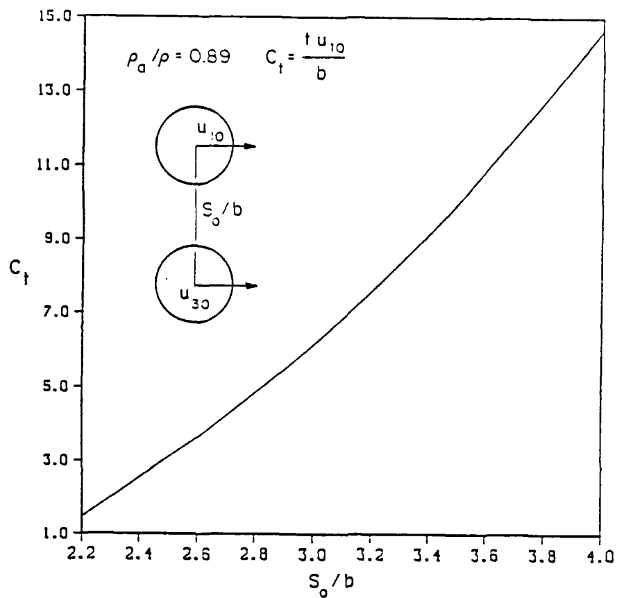
Figure 18. Time required for two equal spheres ( a/b=1 ) to come into contact versus the separation distance s_o/b with \rho_a/\rho = 0.89 , x_{1o}/b = x_{3o}/b = 0 , u_{1o}=u_{2o}=1 , and u_{3o}=u_{4o}=0 .
