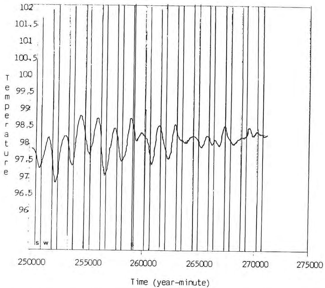
Figure 25. Temperature Pattern of Light Subject JL38. Plotted as in Figure 22. Note the marked attenuation of the rhythm even at the end of the study when bright lights had been discontinued.
