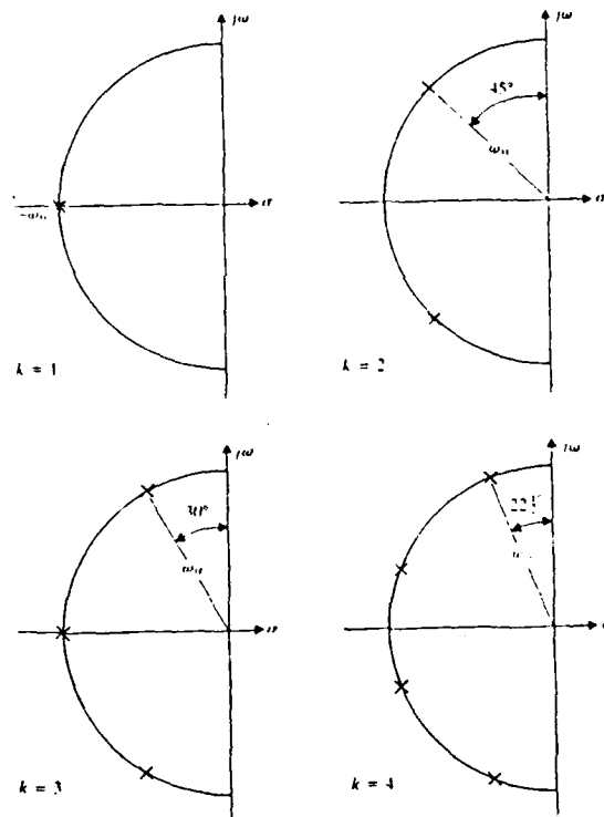
Figure 9. Butterworth pattern of characteristic roots: Here k is the system order. (From Ref 3.)
