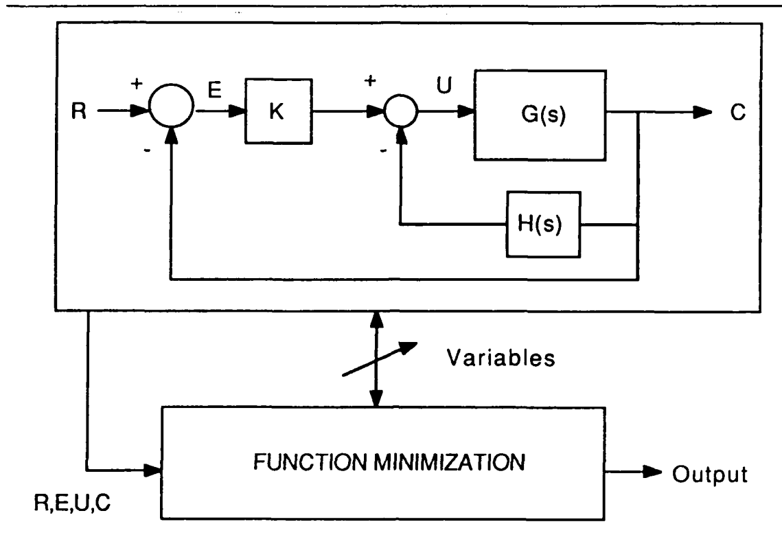
Figure 4. Implementation of function minimization: (From Ref. 1.)
