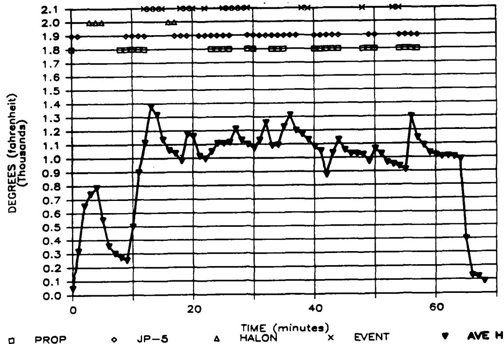
FIGURE 12. Average Temperatures for Horizontal Sonobuoys in Burn 7.
