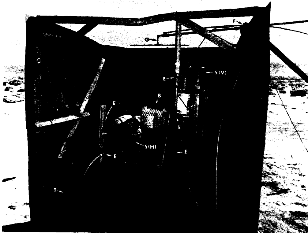
FIGURE 1. Firebox Loaded with 8 Sonobuoys. (B) Basket of batteries, (E) ports for application of extinguishing materials, (G) port for sampling of gases, (F) port from which JP-5 is sprayed into the firebox, (S(H)) sonobuoys stacked in a horizontal position, (S(U)) sonobuoys in a vertical configuration, (T) one of the thermocouples.
