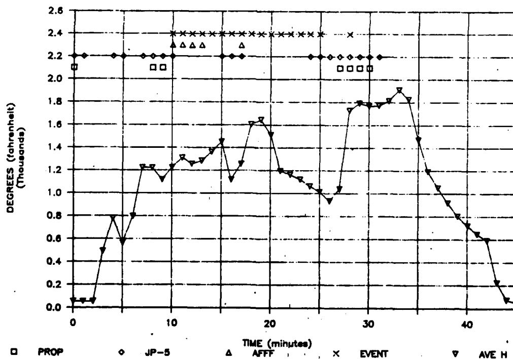
FIGURE 11. Average Temperatures for Horizontal Sonobuoys in Burn 6.
