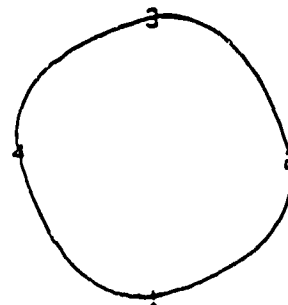
Figure 10. "Quadratic" command
