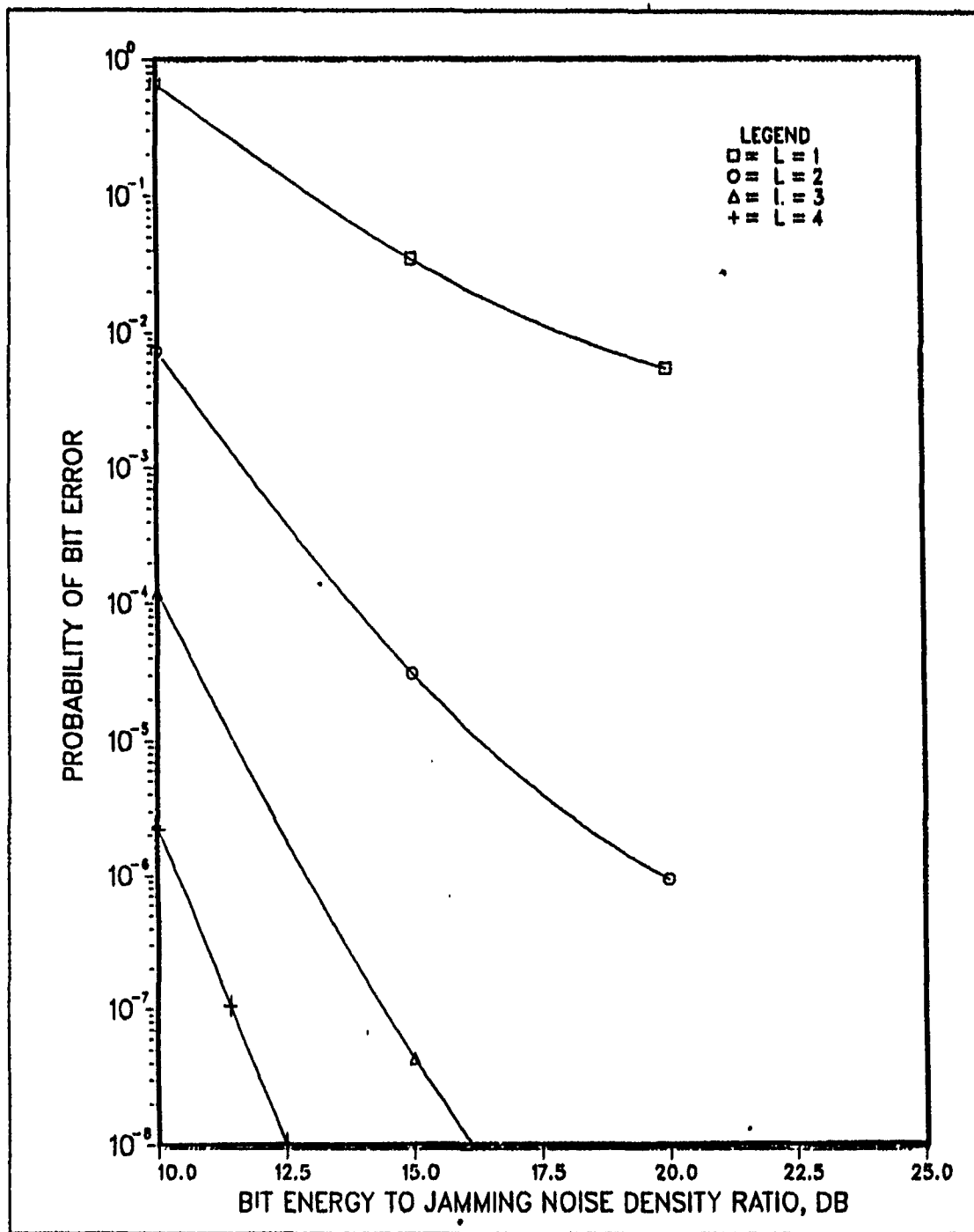
Figure 26. Performance of rate 1/3 convolutional code in Rayleigh fading: \bar{\gamma}^2 = 0 and M = 4 under optimum partial-band jamming conditions with number of hops-per-symbol ( L ) as a parameter when E_b/N_0 = 15 dB.
