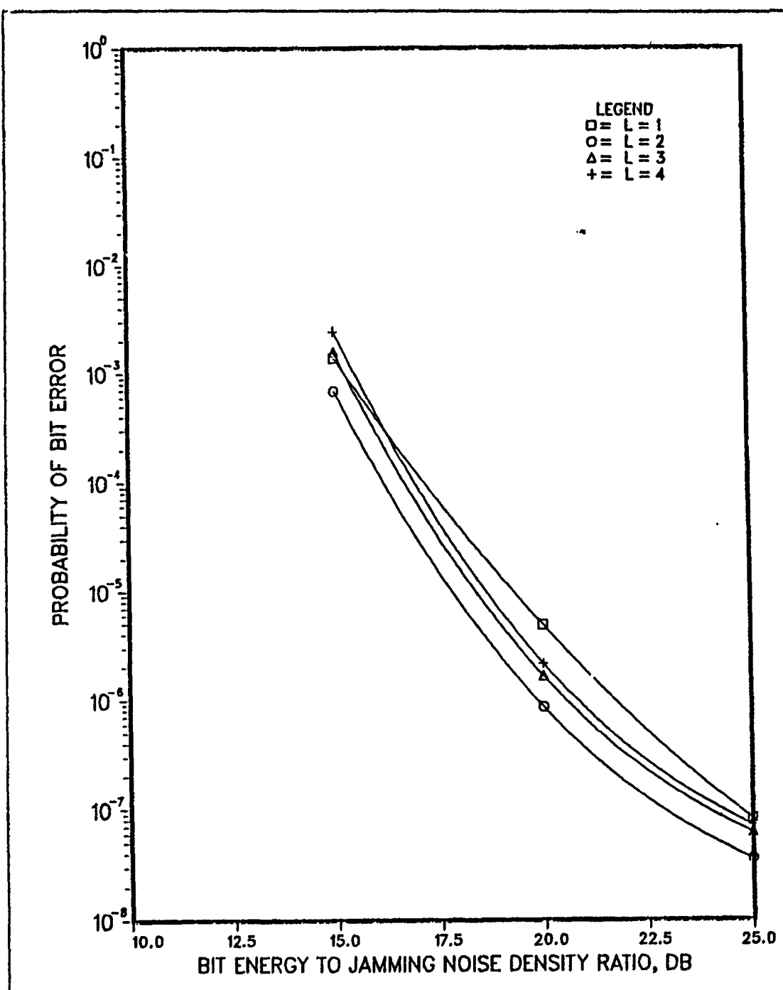
Figure 23. Performance of rate 1/2 convolutional code in Rician fading: \bar{\gamma}^2 = 15 and M=2 under optimum partial-band jamming conditions with number of hops-per-symbol ( L ) as a parameter when E_b/N_0 = 15 dB.
