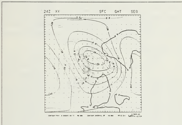
Fig. 14. As in Fig. 12, except for Case 3. Contour interval is 10.
