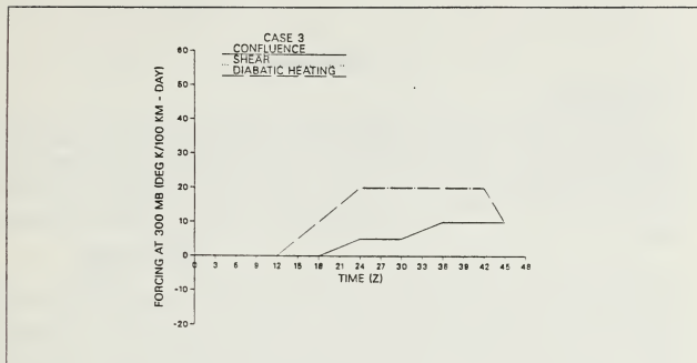
Fig. 42. As in Fig. 38, except for 300 mb.
