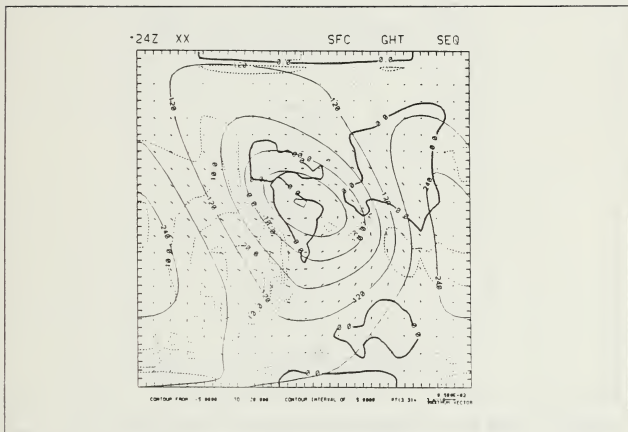
Fig. 12. Total forcing at the surface at 24 h, Case 1. Geopotential height in m (solid), total forcing in K 100 km^{-1} day^{-1} (dashed), and observed wind vectors in m s^{-1} . Wind vectors vary in length according to speed, with the maximum length 50 m s^{-1} . Contour interval of forcing is 5. Heavy lines denote zero contours.
