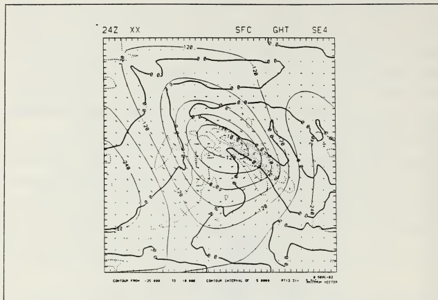
Fig. 34. 24-h surface forcing due to diabatic heating, Case 3. Contour interval is 5.
