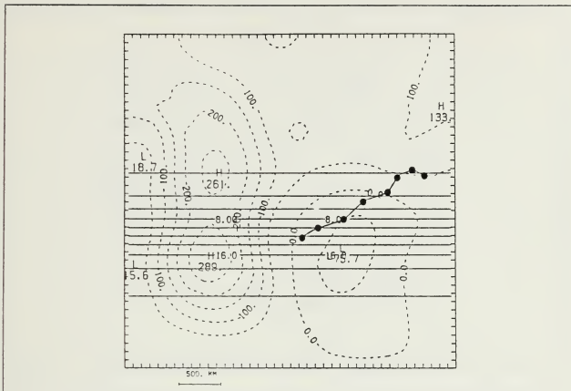
Fig. 9. Case 1 and Case 2 SSI distribution. SST in ^{\circ}\text{C} (solid), with the initial total (latent plus sensible) heat flux distribution in \text{W m}^{-2} , and the cyclone track and position at six-hour intervals from 00 h to 48 h indicated for Case 1.
