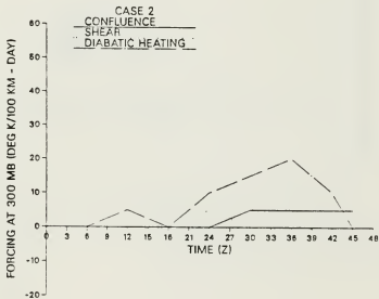
Fig. 41. As in Fig. 37, except for 300 mb.
