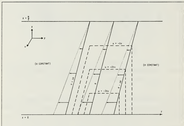
Fig. 2. Idealized cross section through a warm front. The initial position of the potential temperature surfaces is indicated by the solid lines, and their position after they have been slightly advected is indicated by dotted lines. The dashed lines are isotachs of the along-front wind field in geostrophic balance with the initial potential temperature field. From Gidel (1978).
