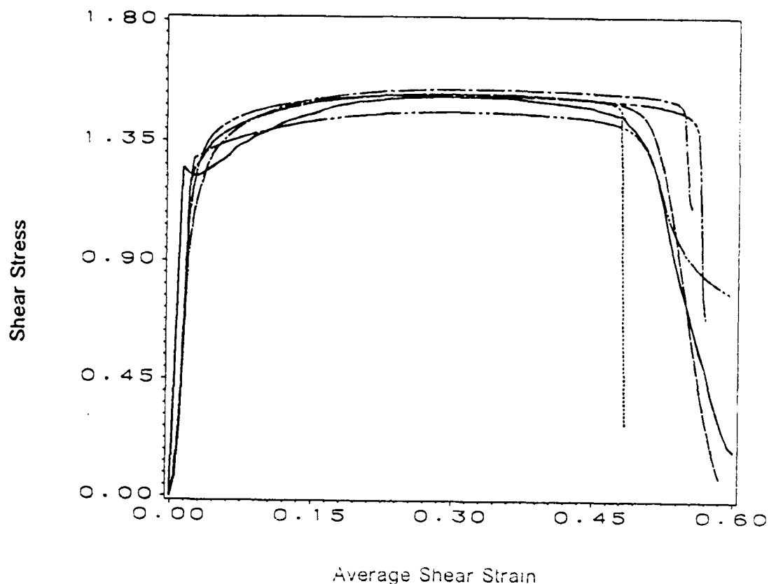
Fig. 1. Shear stress-shear strain curves computed with different flow rules and with different initial temperature perturbations. _____ experimental, _____. Bodner-Partom, ..... Litonski (non-polar), _____ Litonski (dipolar) _____ Power, _____ Johnson-Cook.
