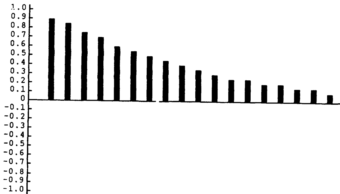
Figure 26. Autocorrelation of I=4 Data
