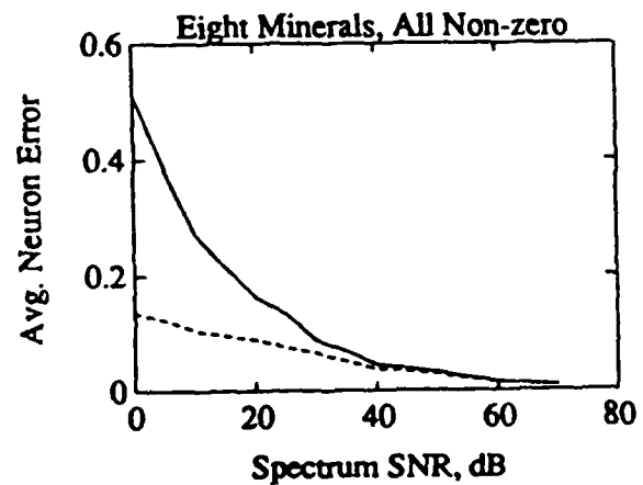
Figure 7. Accuracy vs. noise for pseudoinverse (solid line) and neural net (dotted line).
