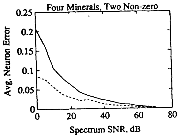
Figure 6. Accuracy vs. noise for pseudoinverse (solid line) and neural net (dotted line).
