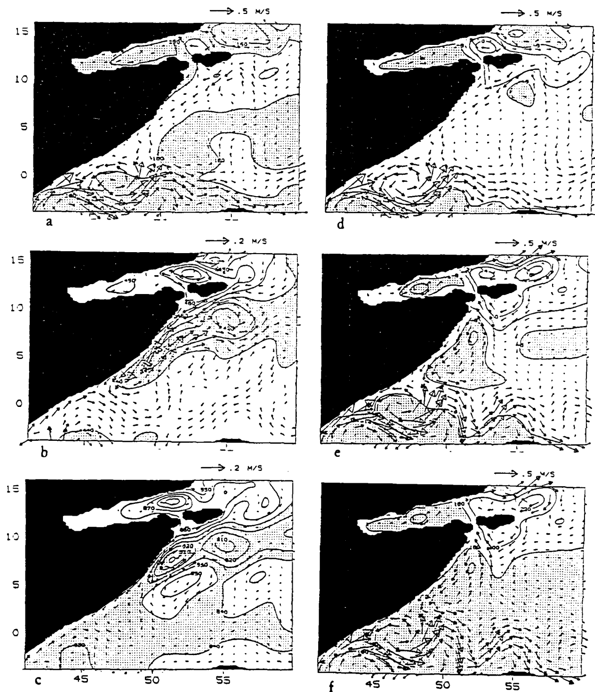
Figure 28. Ten year average November 16. Velocity and depth to the bottom of layer 1, (a), layer 2, (b), layer 3, (c) and surface elevation, (d) in the 3.5 layer model. Panels (e) and (f) show the surface elevation and upper layer thickness with velocity vectors in the 1.5 layer model.
