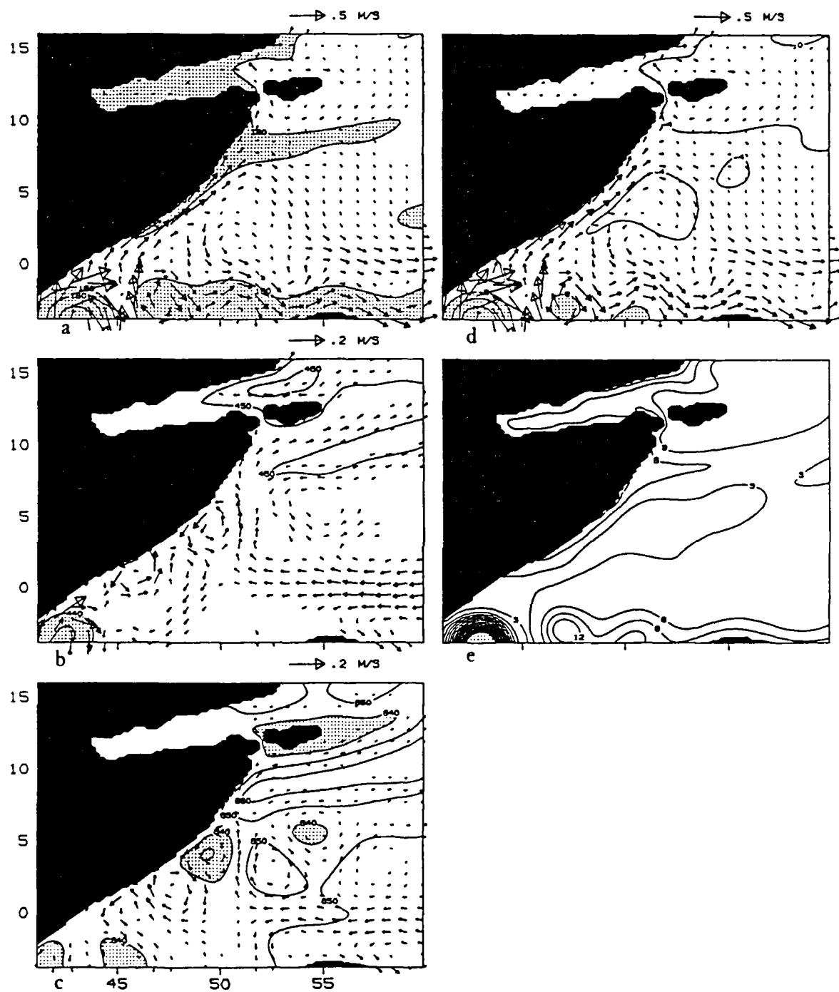
Figure 33. May 28, year 21, 3.5 layer model. Velocity and depth (m) to the bottom of layer 1, (a), layer 2, (b), layer 3, (c), velocity of upper layer and surface elevation (cm), (d). Panel (e): Available potential energy, (kJ/m 2 ).
