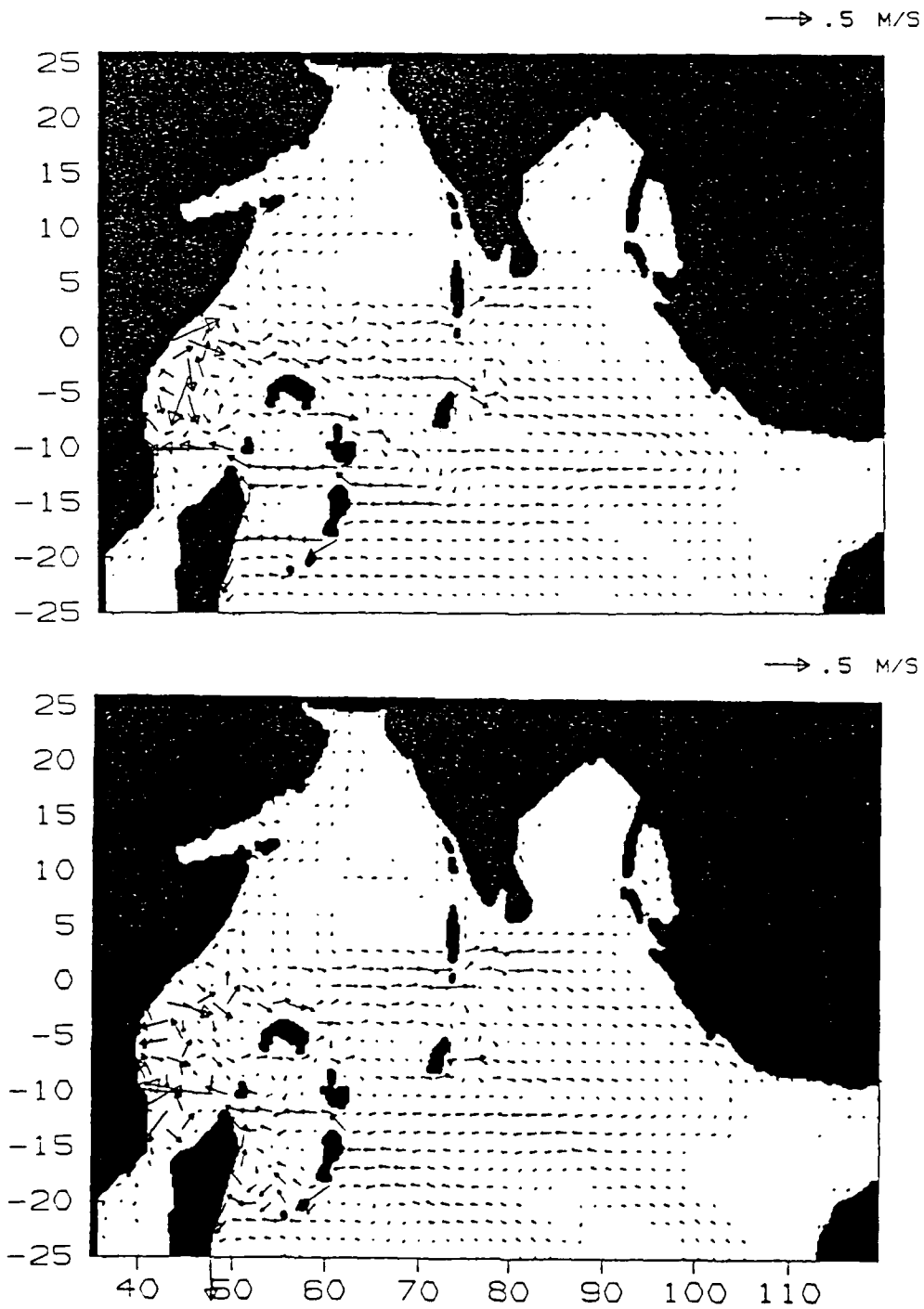
Figure 10. Current velocity in the upper layer of the Indian Ocean. Ten year average of May 16. top: 1.5 layer model. bottom: 3.5 layer model
