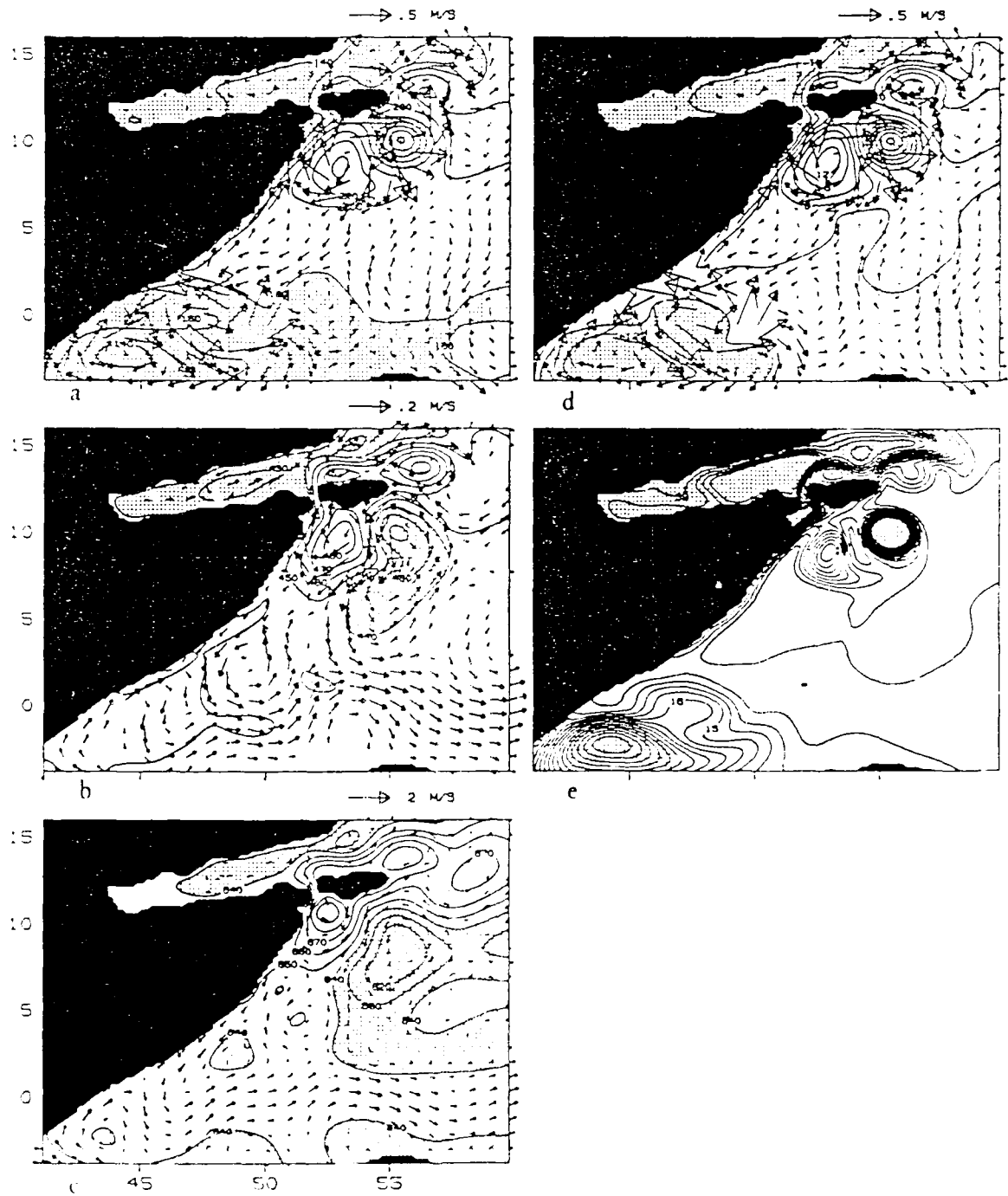
Figure 15. September 22, year 21, 3.5 layer model. Velocity and depth (m) to the bottom of layer 1, (a), layer 2, (b), layer 3, (c), velocity of upper layer and surface elevation (cm), (d). Panel (e). Available potential energy ( \text{kJ m}^2 )
