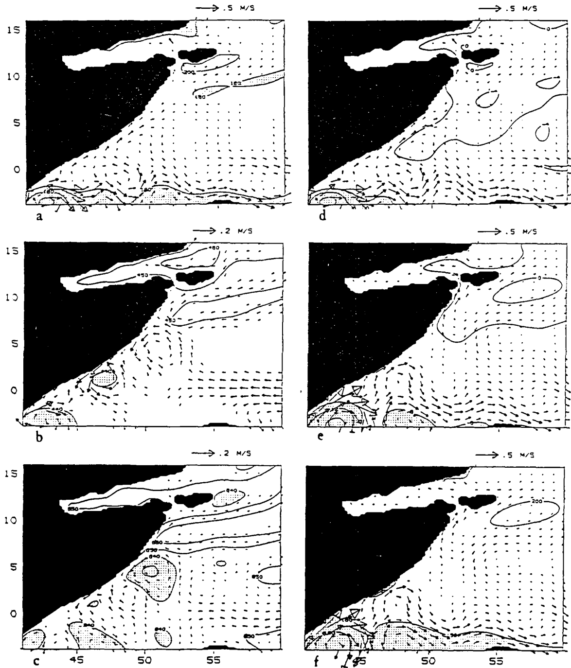
Figure 25. Ten year average May 16. Velocity and depth to the bottom of layer 1, (a), layer 2, (b), layer 3, (c) and surface elevation, (d) in the 3.5 layer model. Panels (e) and (f) show the surface elevation and upper layer thickness with velocity vectors in the 1.5 layer model.
