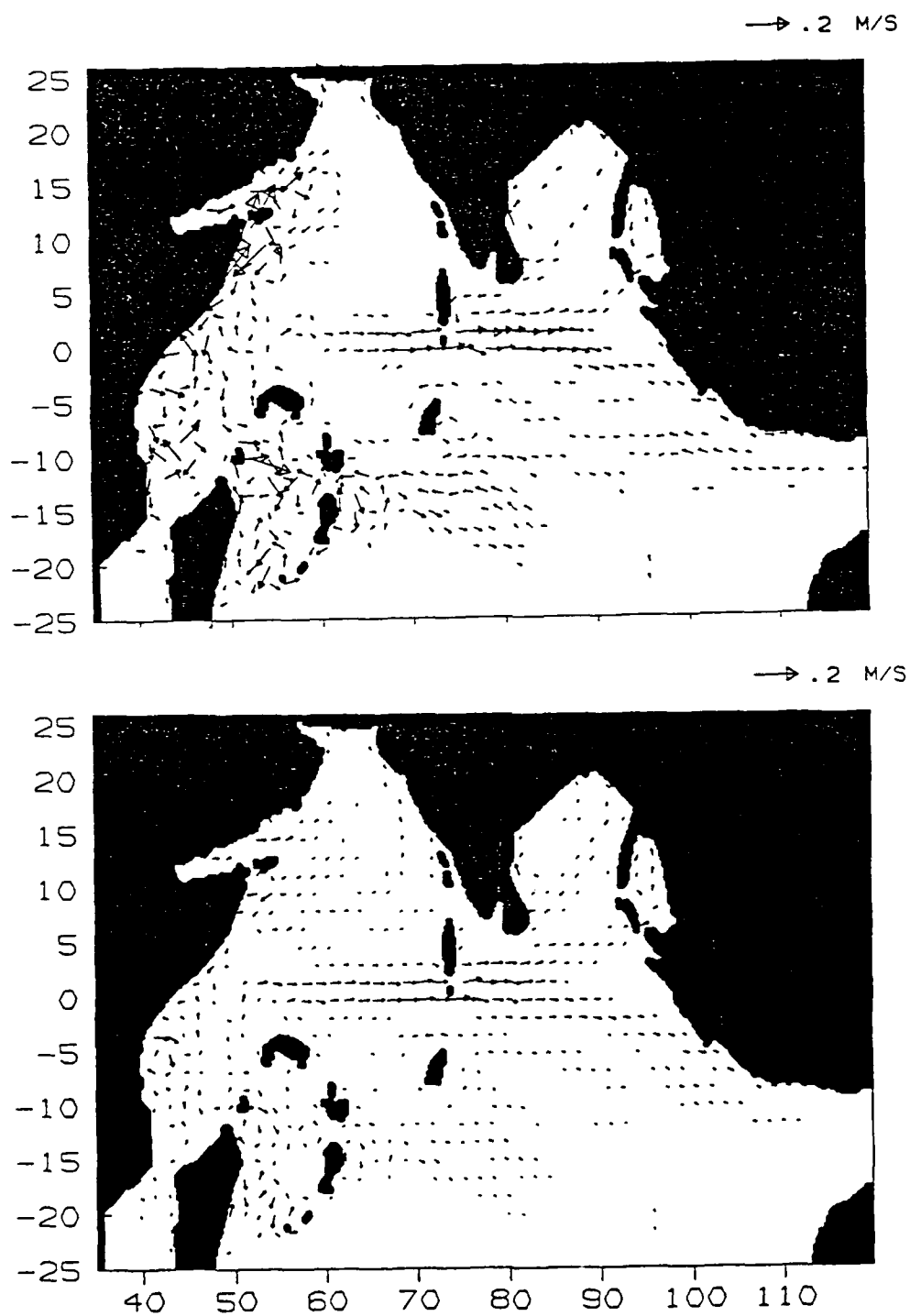
Figure 14. Current velocity in the second (top) and third (bottom) layer of the Indian Ocean. Ten year average of August 16.
