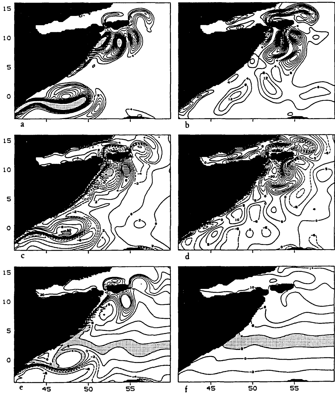
Figure 48. October 4, year 21, 3.5 layer model. Kinetic energy ( \text{kJ/m}^2 , shading: E_{kin} > 40 ) in layer 1, (a), and layer (2), (b), ( 100 \text{ J/m}^2 , shading: E_{kin} > 50 ). Relative vorticity in layer 1 ( 10^{-6} \text{ s}^{-1} , shading: |\zeta| > 10 ), (c), and layer 2 ( 10^{-7} \text{ s}^{-1} , shading: |\zeta| > 30 ), (d). Potential vorticity in layer 1, (e), and layer 2, (f), ( 10^{-8} \text{ m}^{-1} \text{ s}^{-1} , 2 \leq \Pi \leq 4 is shaded).
