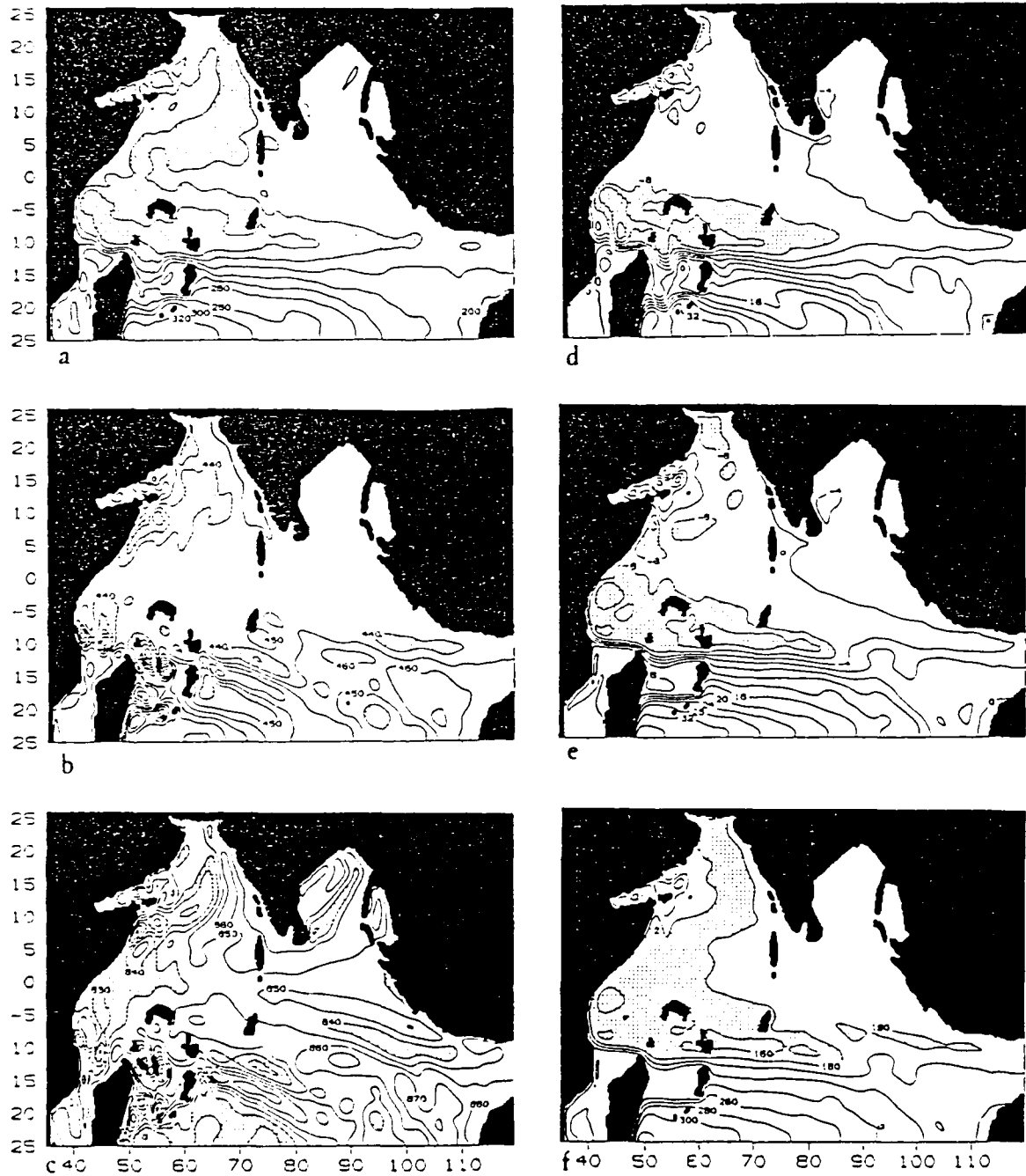
Figure 18. Ten year average November 16. Depth to the bottom of layer 1 (a), layer 2 (b), layer 3, (c) and surface elevation (d) in the 3.5 layer model. Panels (e) and (f) show the surface elevation and upper layer thickness in the 1.5 layer model.
