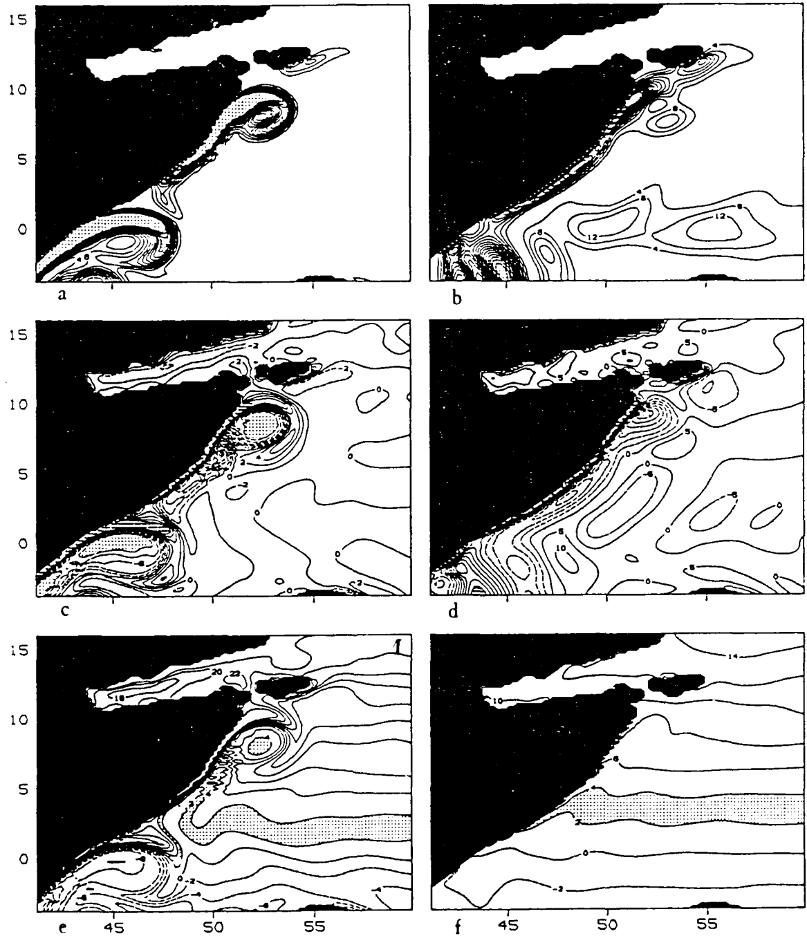
Figure 38. July 16, year 21, 3.5 layer model. Kinetic energy ( \text{kJ/m}^2 , shading: E_{\text{kin}} > 40 ) in layer 1, (a), and layer 2, (b), ( 100 \text{ J/m}^2 , shading: E_{\text{kin}} > 50 ). Relative vorticity in layer 1 ( 10^{-6} \text{ s}^{-1} , shading: |\zeta| > 10 ), (c), and layer 2 ( 10^{-7} \text{ s}^{-1} , shading: |\zeta| > 30 ), (d). Potential vorticity in layer 1, (e), and layer 2, (f), ( 10^{-8} \text{ m}^{-1} \text{ s}^{-1} , 2 \leq \Pi \leq 4 is shaded).
