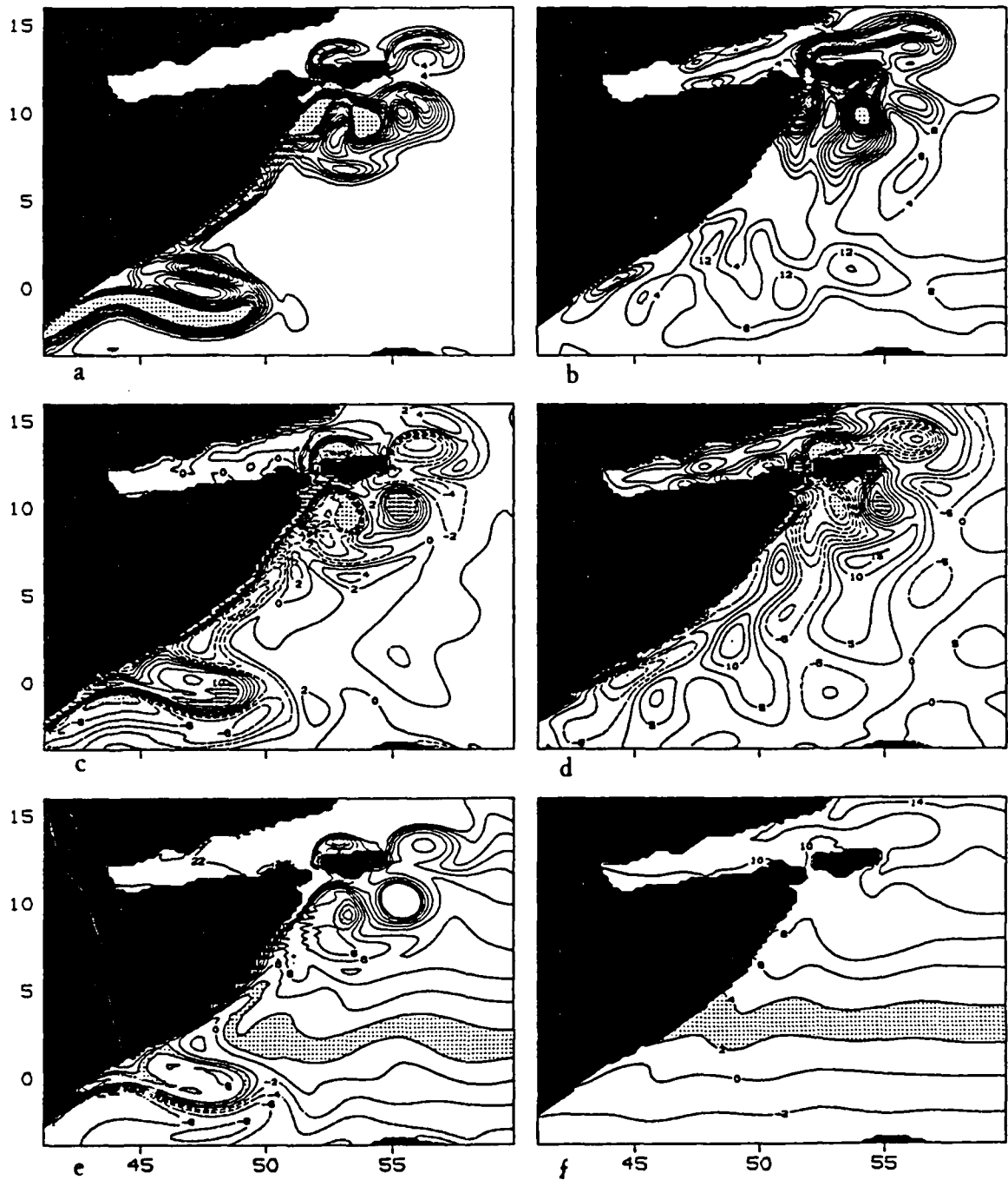
Figure 46. September 22, year 21, 3.5 layer model. Kinetic energy ( \text{kJ/m}^2 , shading: E_{kin} > 40 ) in layer 1, (a), and layer (2), (b), ( 100 \text{ J/m}^2 , shading: E_{kin} > 50 ). Relative vorticity in layer 1 ( 10^{-6} s^{-1} , shading: |\zeta| > 10 ), (c), and layer 2 ( 10^{-7} s^{-1} , shading: |\zeta| > 30 ), (d). Potential vorticity in layer 1, (e), and layer 2, (f), ( 10^{-8} m^{-1} s^{-1} , 2 \leq \Pi \leq 4 is shaded).
