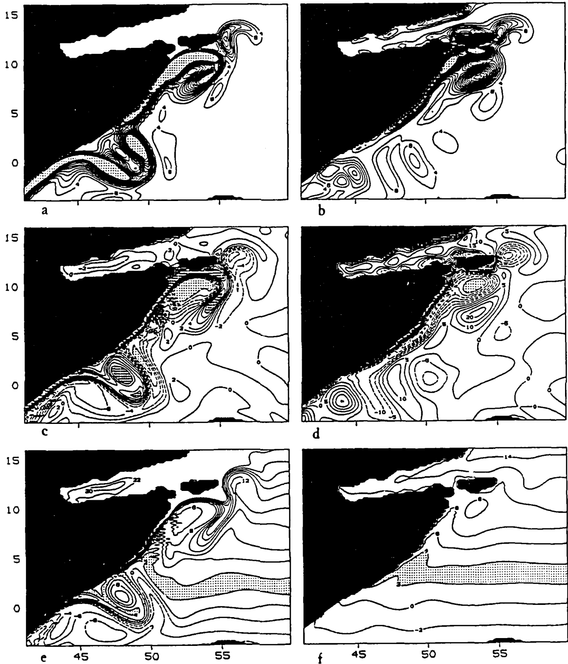
Figure 42. August 22, year 21, 3.5 layer model. Kinetic energy ( \text{kJ/m}^2 , shading: E_{\text{kin}} > 40 ) in layer 1, (a), and layer (2), (b), ( 100 \text{ J/m}^2 , shading: E_{\text{kin}} > 50 ). Relative vorticity in layer 1 ( 10^{-6} \text{ s}^{-1} , shading: |\zeta| > 10 ), (c), and layer 2 ( 10^{-7} \text{ s}^{-1} , shading: |\zeta| > 30 ), (d). Potential vorticity in layer 1, (e), and layer 2, (f), ( 10^{-8} \text{ m}^{-1} \text{ s}^{-1} , 2 \leq \Pi \leq 4 is shaded).
