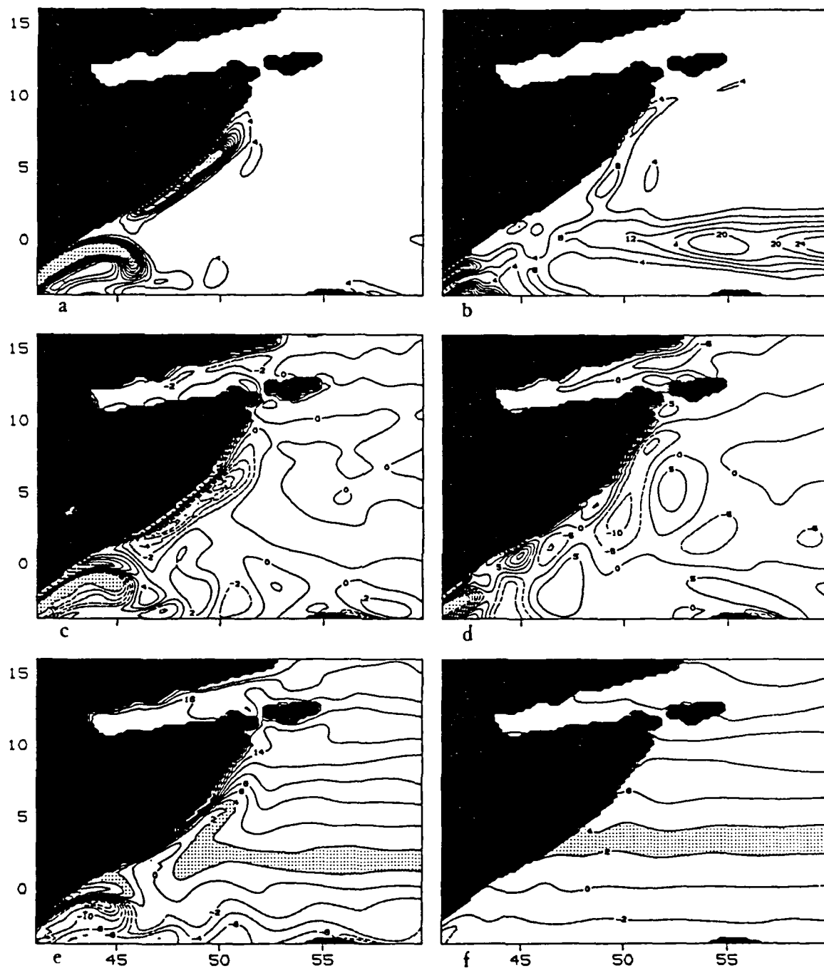
Figure 36. June 16, year 21, 3.5 layer model. Kinetic energy ( \text{kJ/m}^2 , shading: E_{\text{kin}} > 40 ) in layer 1, (a), and layer 2, (b), ( 100 \text{ J/m}^2 , shading: E_{\text{kin}} > 50 ). Relative vorticity in layer 1 ( 10^{-6} \text{ s}^{-1} , shading: |\zeta| > 10 ), (c), and layer 2 ( 10^{-7} \text{ s}^{-1} , shading: |\zeta| > 30 ), (d). Potential vorticity in layer 1, (e), and layer 2, (f), ( 10^{-8} \text{ m}^{-1} \text{ s}^{-1} , 2 \leq \Pi \leq 4 is shaded).
