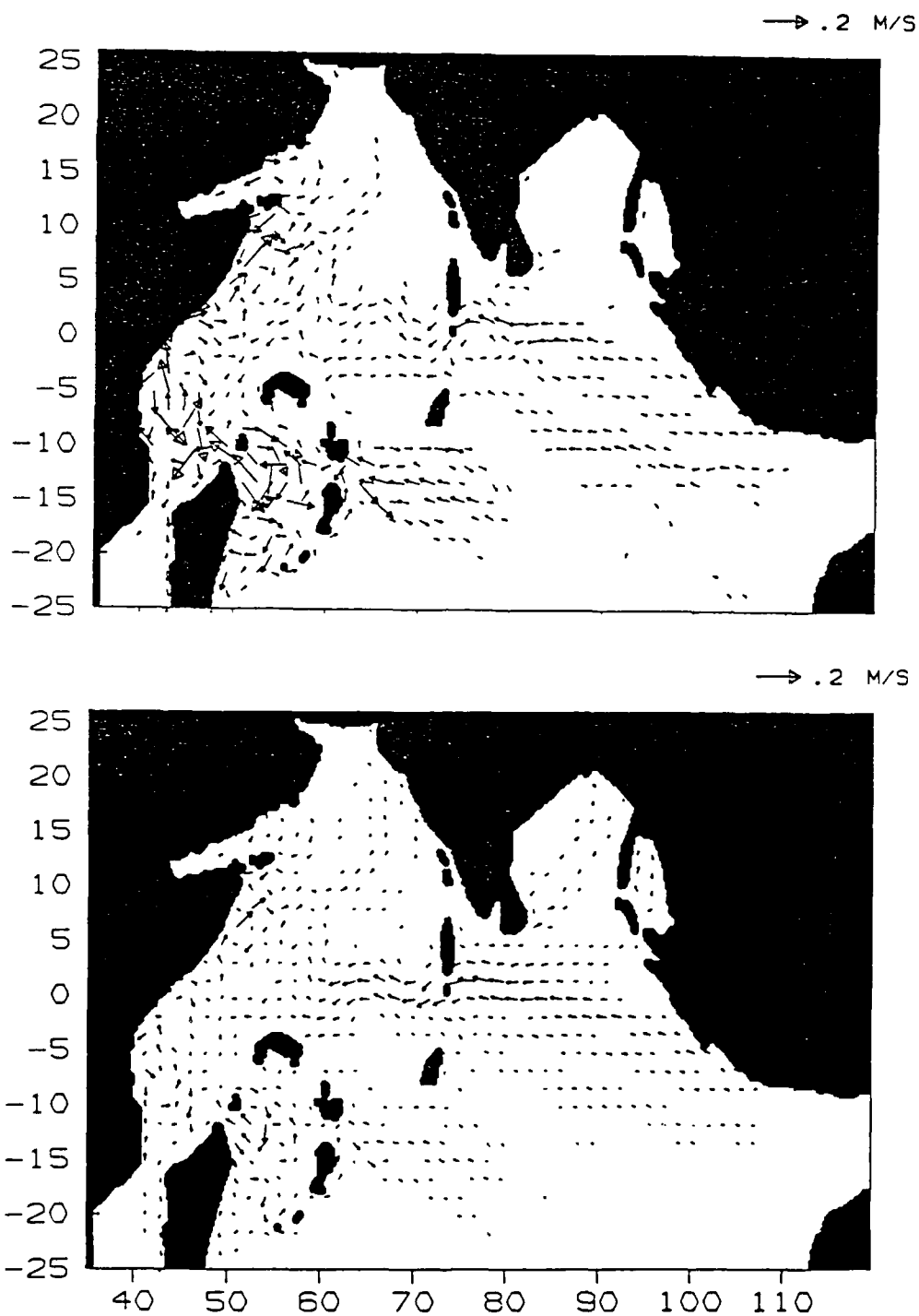
Figure 17. Current velocity in the second (top) and third (bottom) layer of the Indian Ocean. Ten year average of November 16.
