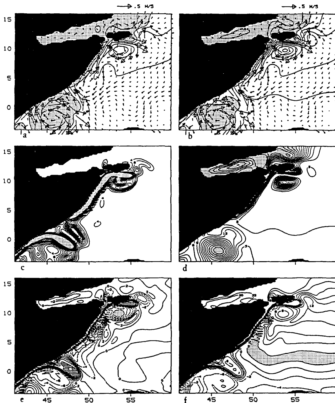
Figure 49. August 10, year 21, 1.5 layer model. Velocity and depth (m) to the bottom of active layer, (a) and surface elevation, (b). Kinetic energy ( \text{kJ/m}^2 , shading: E_{\text{kin}} > 40 ), (c). Available potential energy, ( \text{kJ/m}^2 ), (d). Relative vorticity ( 10^{-6} \text{s}^{-1} , shading: |\zeta| > 10 ), (e). Potential vorticity, (f). ( 10^{-8} \text{m}^{-1} \text{s}^{-1} , 2 \leq \Pi \leq 4 ) is shaded.
