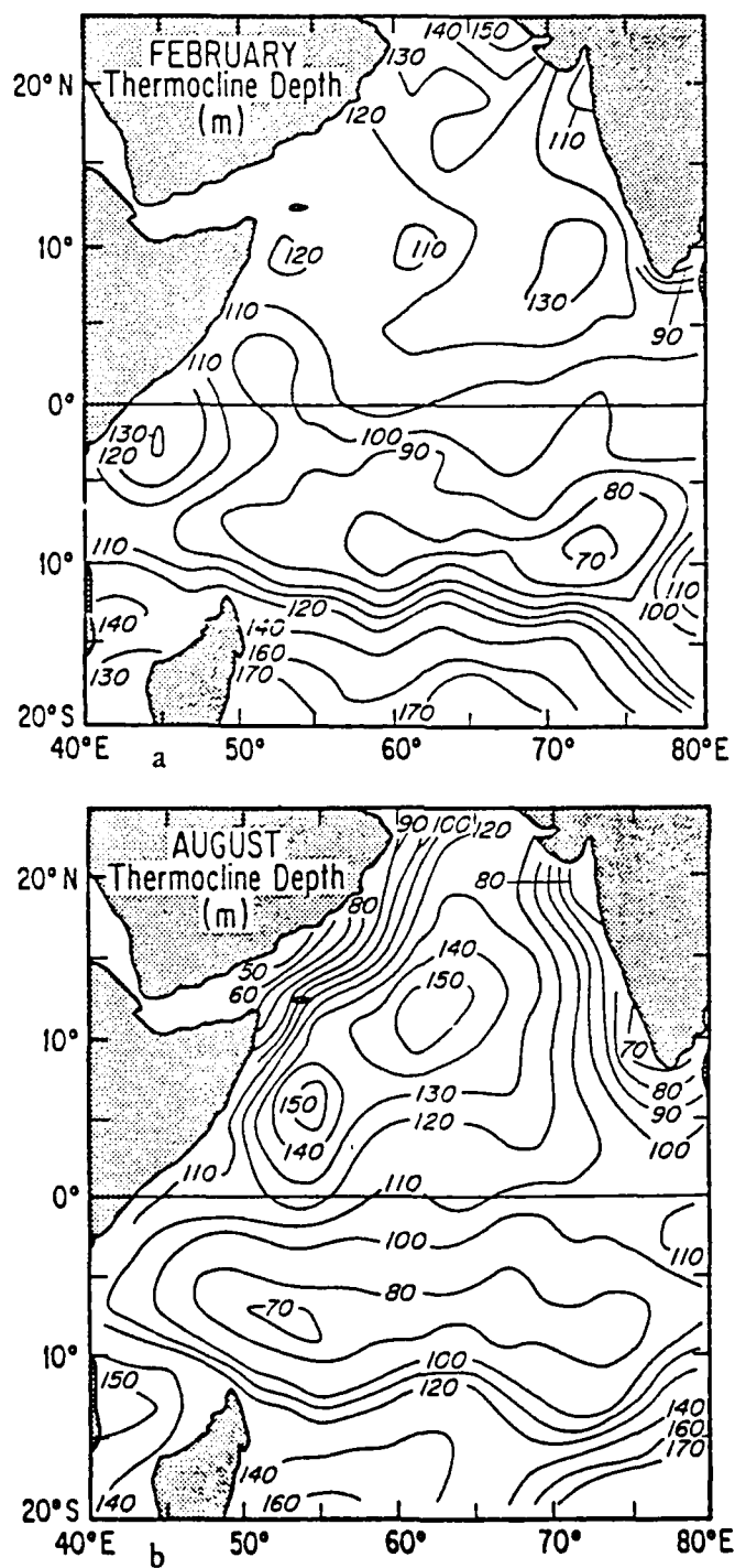
Figure 20. Thermocline depth climatology for February (a) and August (b). From Molinari, Festa and Swallow (1986).
