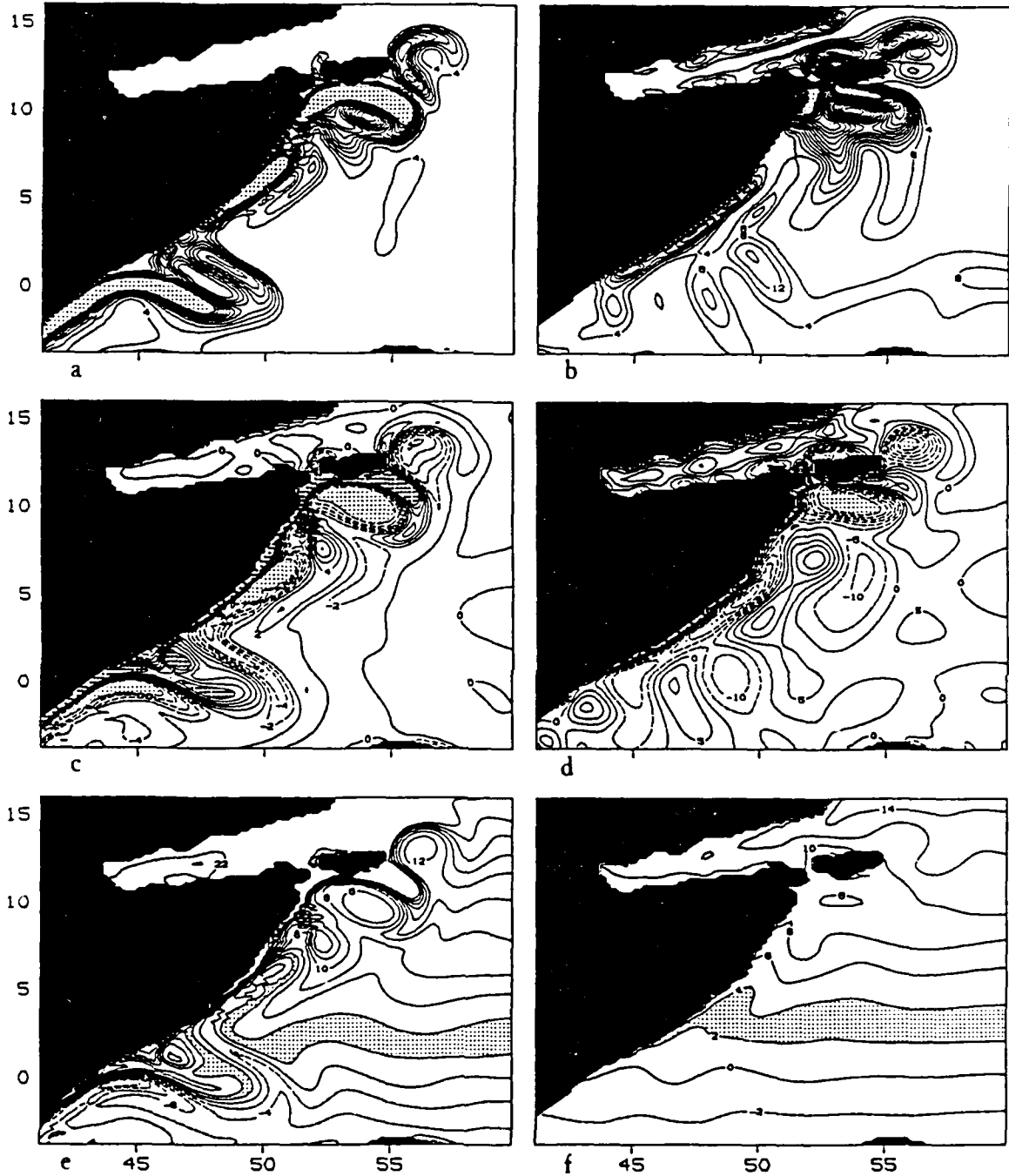
Figure 44. September 4, year 21, 3.5 layer model. Kinetic energy ( \text{kJ/m}^2 , shading: E_{kin} > 40 ) in layer 1, (a), and layer (2), (b), ( 100 \text{ J/m}^2 , shading: E_{kin} > 50 ). Relative vorticity in layer 1 ( 10^{-6} \text{s}^{-1} , shading: |\zeta| > 10 ), (c), and layer 2 ( 10^{-7} \text{s}^{-1} , shading: |\zeta| > 30 ), (d). Potential vorticity in layer 1, (e), and layer 2, (f), ( 10^{-8} \text{m}^{-1} \text{s}^{-1} , 2 \leq \Pi \leq 4 is shaded).
