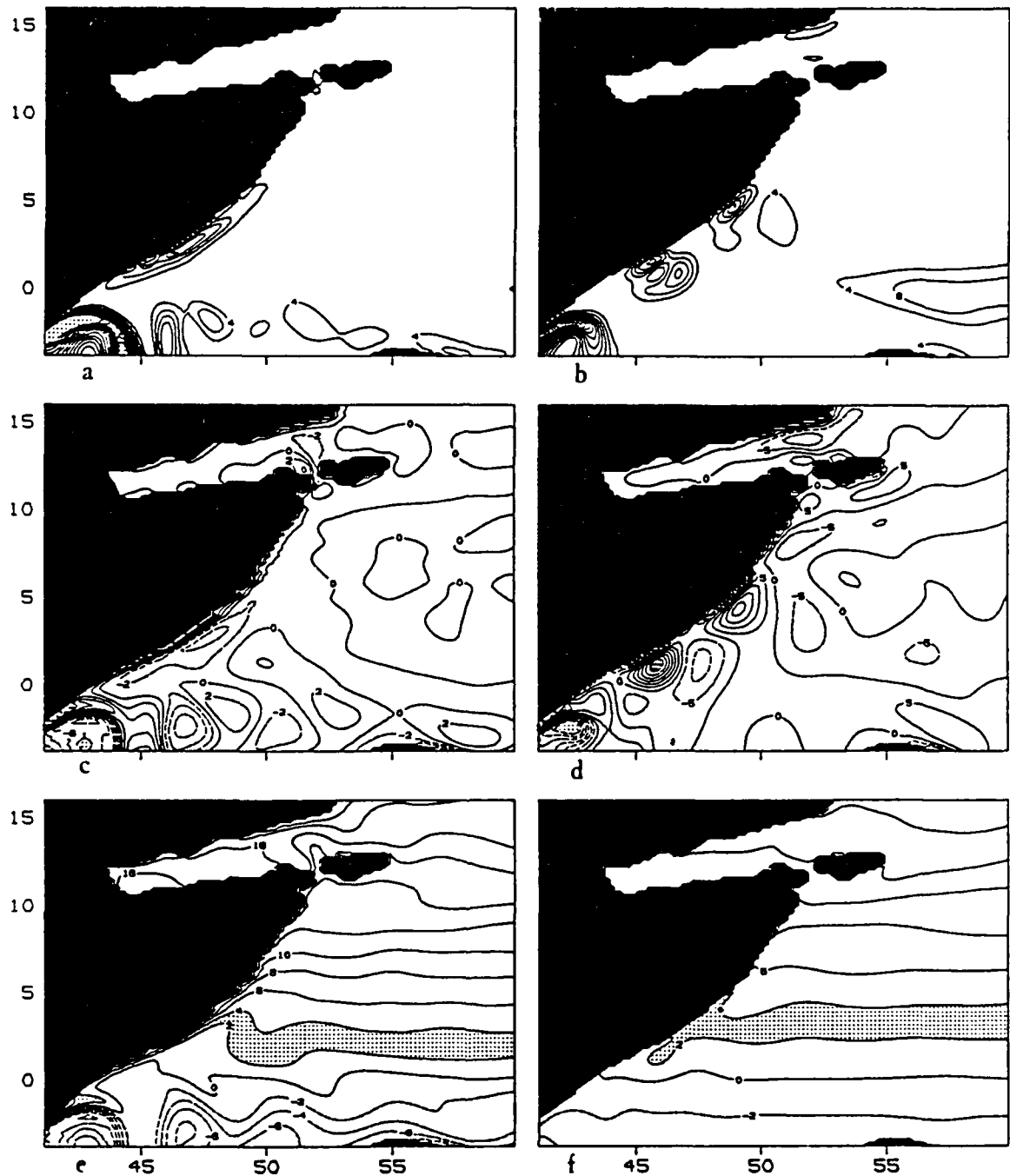
Figure 34. May 28, year 21, 3.5 layer model. Kinetic energy ( \text{kJ/m}^2 , shading: E_{\text{kin}} > 40 ) in layer 1, (a), and layer 2, (b), ( 100 \text{ J/m}^2 , shading: E_{\text{kin}} > 50 ). Relative vorticity in layer 1 ( 10^{-6} \text{ s}^{-1} , shading: |\zeta| > 10 ), (c), and layer 2 ( 10^{-7} \text{ s}^{-1} , shading: |\zeta| > 30 ), (d). Potential vorticity in layer 1, (e), and layer 2, (f), ( 10^{-8} \text{ m}^{-1} \text{ s}^{-1} , 2 \leq \Pi \leq 4 is shaded).
