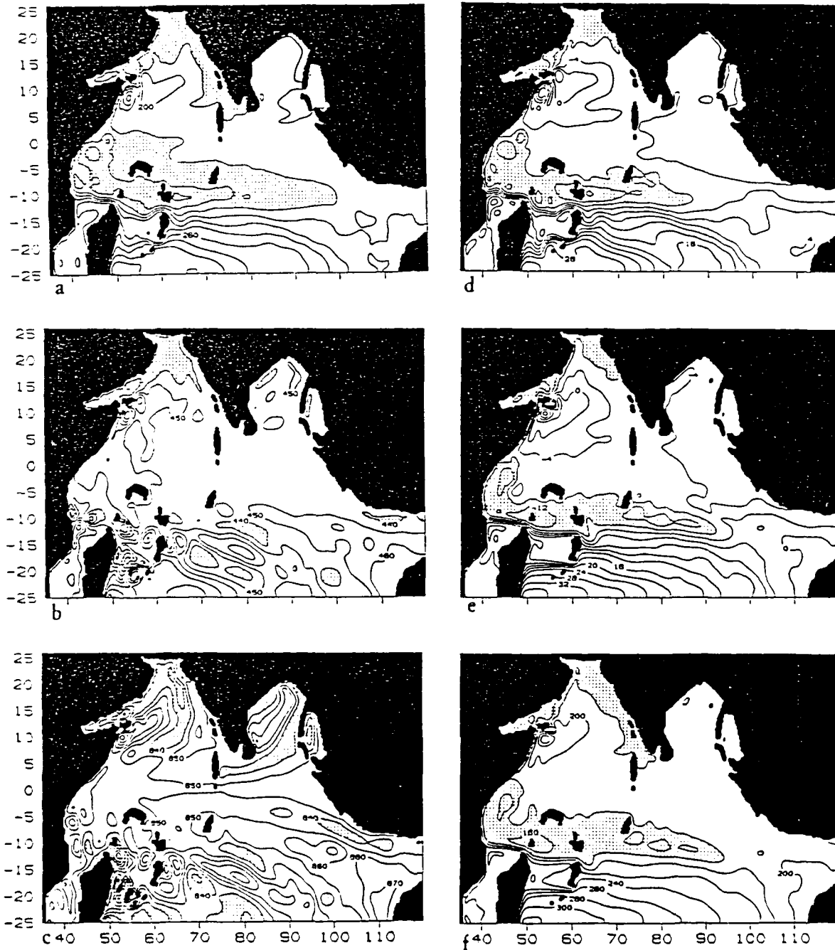
Figure 15. Ten year average August 16. Depth to the bottom of layer 1 (a), layer 2 (b), layer 3, (c) and surface elevation (d) in the 3.5 layer model. Panels (e) and (f) show the surface elevation and upper layer thickness in the 1.5 layer model.
