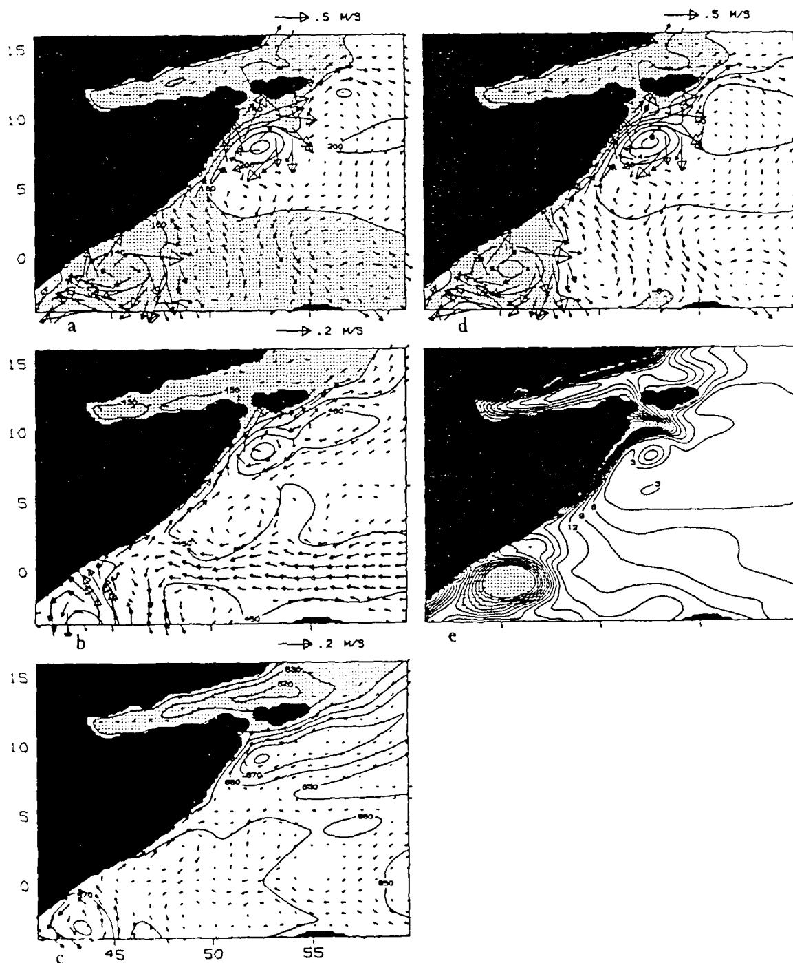
Figure 37. July 16, year 21, 3.5 layer model. Velocity and depth (m) to the bottom of layer 1, (a), layer 2, (b), layer 3, (c), velocity of upper layer and surface elevation (cm), (d). Panel (e): Available potential energy, ( \text{kJ/m}^2 ).
