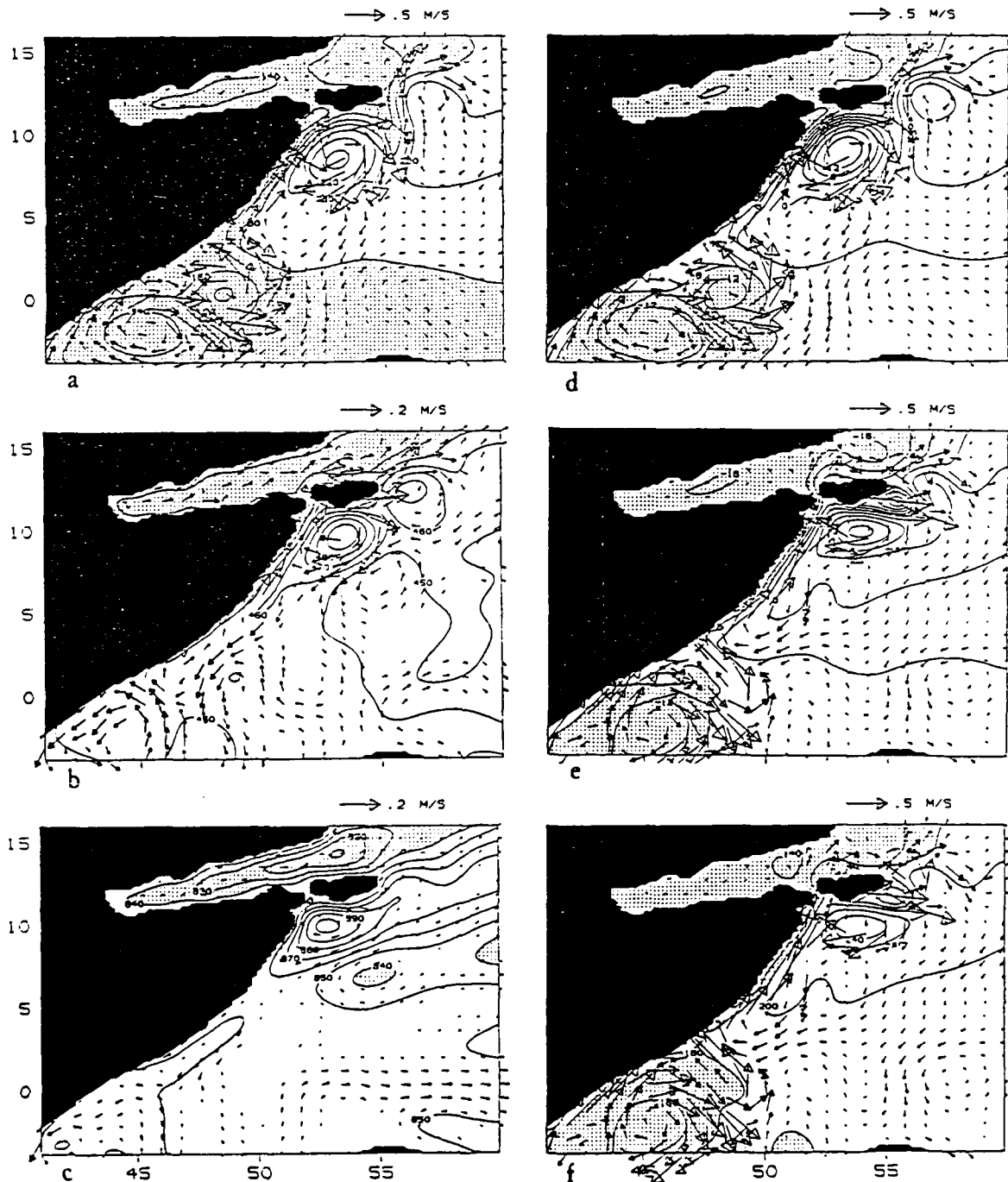
Figure 26. Ten year average August 16. Velocity and depth to the bottom of layer 1, (a), layer 2, (b), layer 3, (c) and surface elevation, (d) in the 3.5 layer model. Panels (e) and (f) show the surface elevation and upper layer thickness with velocity vectors in the 1.5 layer model.
