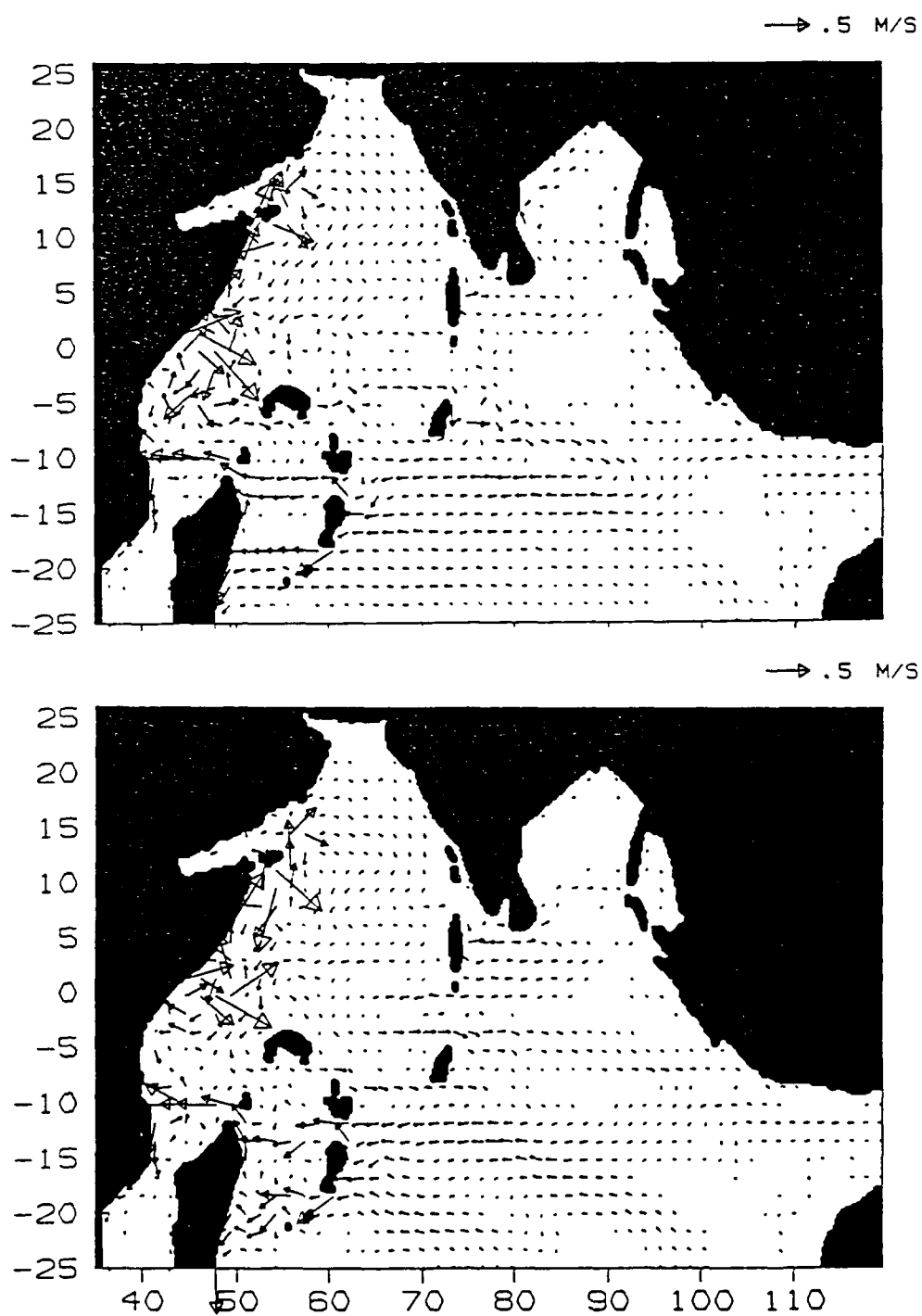
Figure 13. Current velocity in the upper layer of the Indian Ocean. Ten year average of August 16. top: 1.5 layer model. bottom: 3.5 layer model
