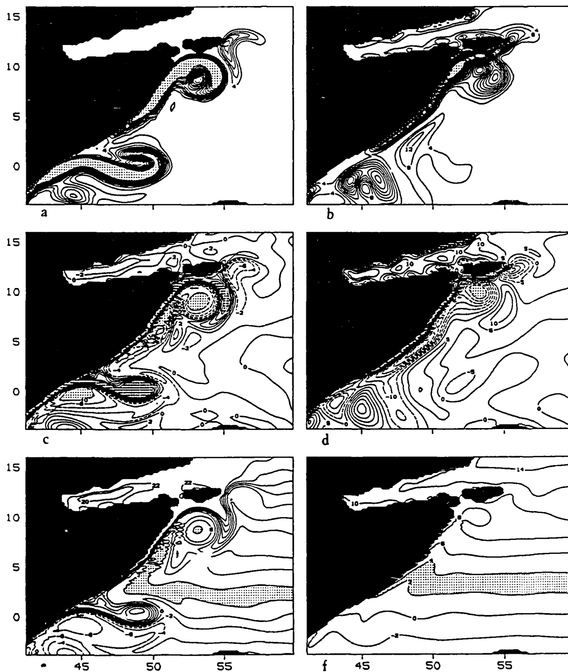
Figure 40. August 10, year 21, 3.5 layer model. Kinetic energy ( \text{kJ/m}^2 , shading: E_{kin} > 40 ) in layer 1, (a), and layer (2), (b), ( 100 \text{ J/m}^2 , shading: E_{kin} > 50 ). Relative vorticity in layer 1 ( 10^{-6} \text{ s}^{-1} , shading: |\zeta| > 10 ), (c), and layer 2 ( 10^{-7} \text{ s}^{-1} , shading: |\zeta| > 30 ), (d). Potential vorticity in layer 1, (e), and layer 2, (f), ( 10^{-8} \text{ m}^{-1} \text{ s}^{-1} , 2 \leq \Pi \leq 4 is shaded).
