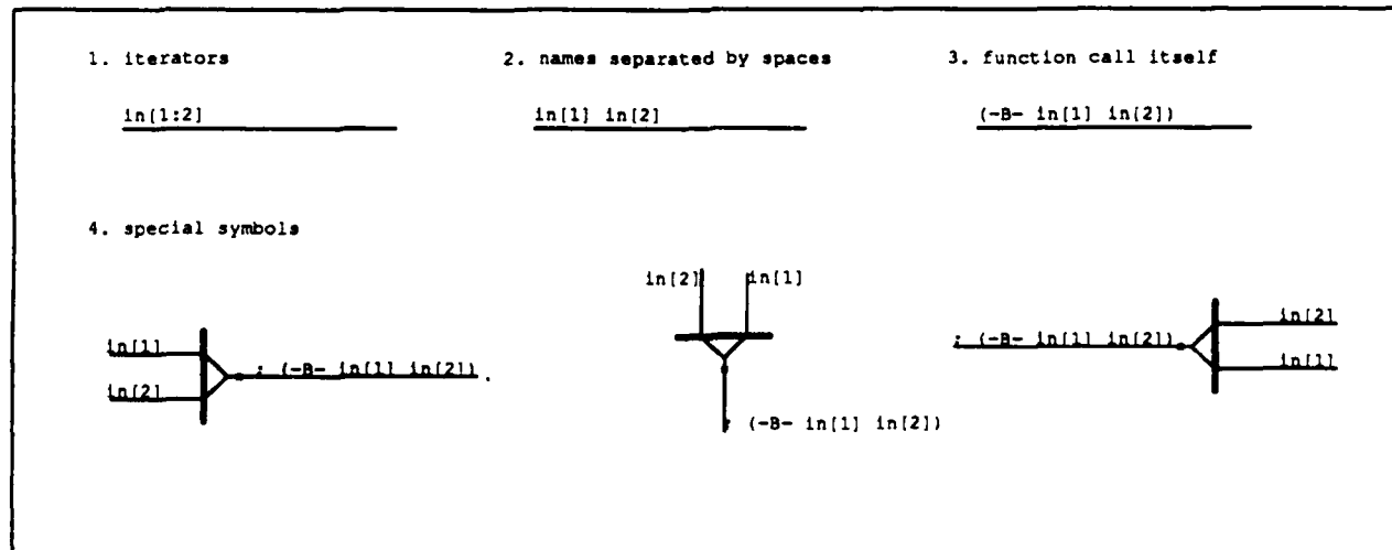
(b) various ways of bundling signals: (-B- in[1] in[2])
