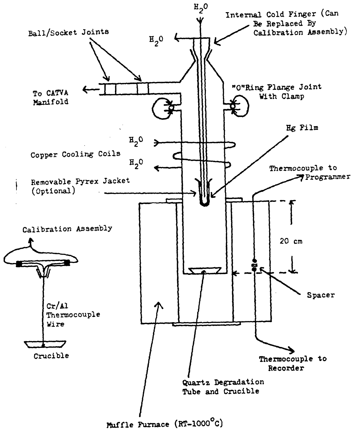
FIGURE 12 OVEN ASSEMBLY
