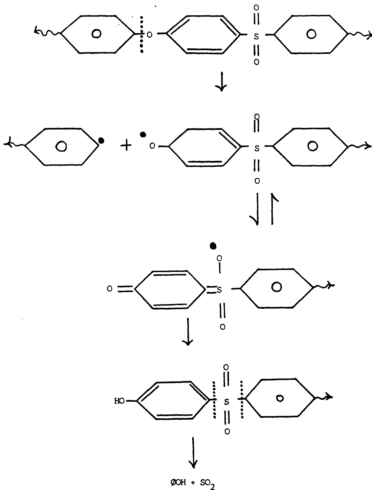
FIGURE 112 CONCERTED PRODUCTION OF SULFUR DIOXIDE AND PHENOL IN PROCESS I OF DEGRADATION
