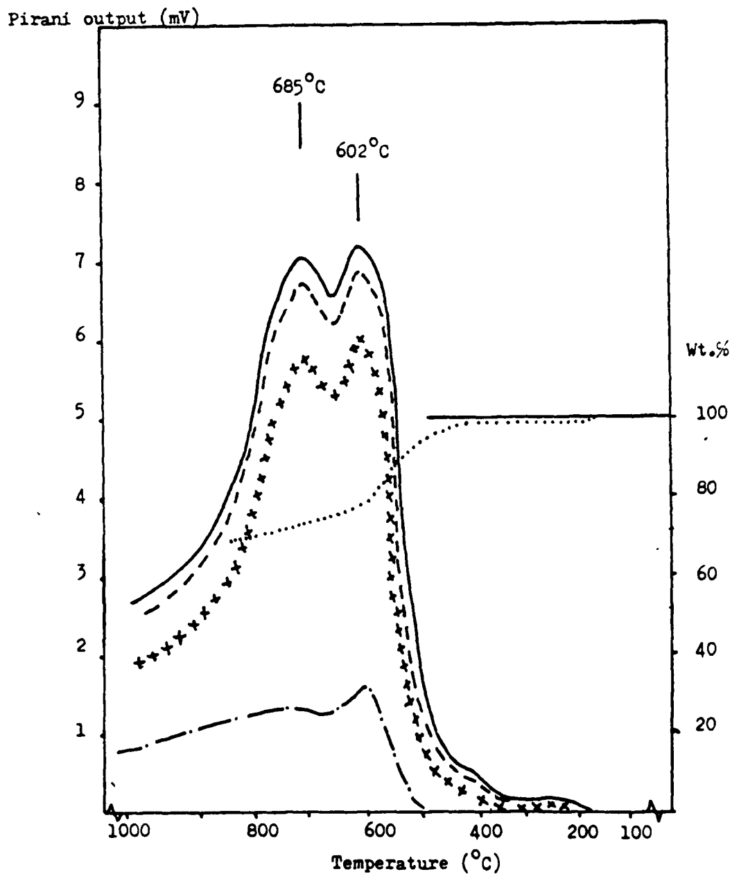
FIGURE 53 CATVA/TGA OF ATP MONOMER
