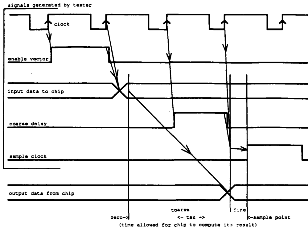
Figure 11: Tester timing
