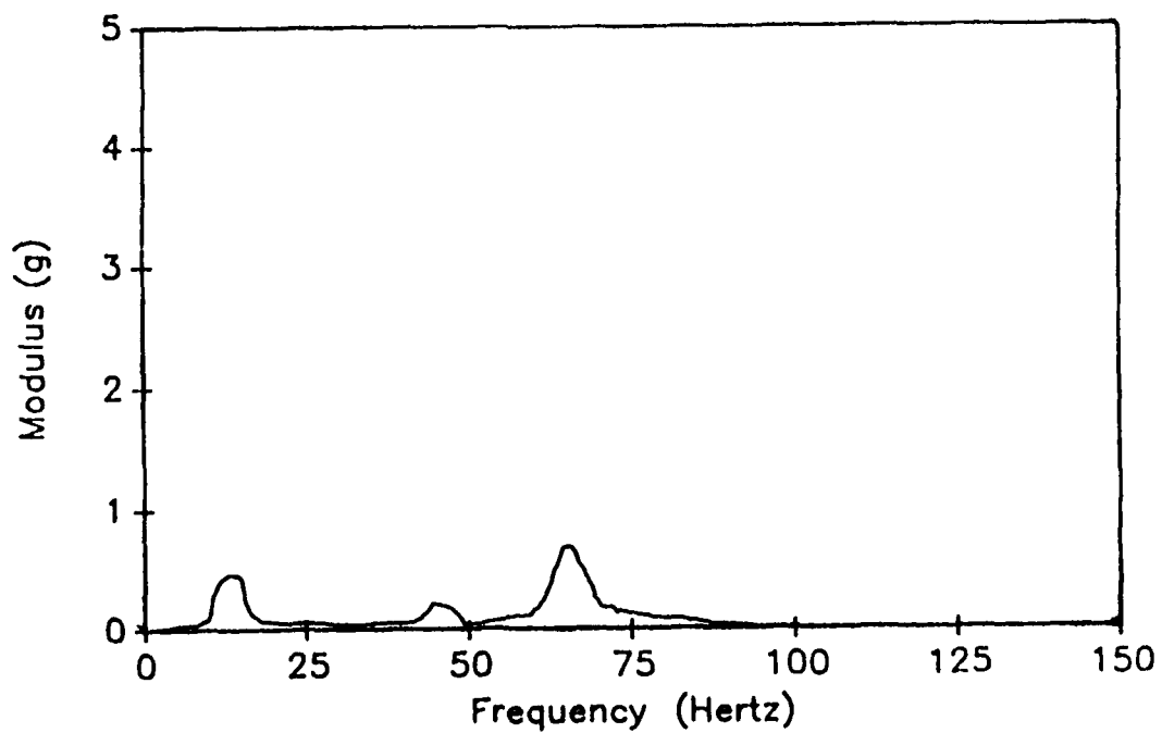
Figure 3.11. Modulus of Acceleration #5 Record for Continuous Beam.
