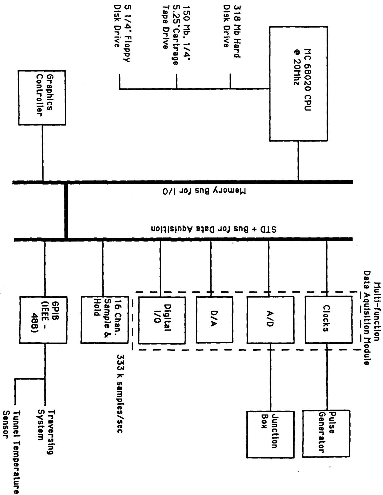
Fig. 14 Schematic of the MASSCOMP MC5450-01 Scientific Laboratory System
