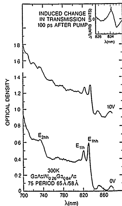
Fig.1. Absorption spectra of the MQW p-i-n modulator (vertically shifted for clarity). Inset: differential transmission at 10 V and 100 ps after the pump. Arrow: wavelength used for time-resolved measurements at 10 V.
