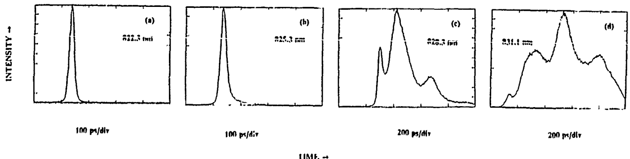
Fig 3. Diode laser output pulse shape of different spectral components. The x-axis represents only the pulse duration but not the delay.
