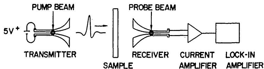
Figure 1. Schematic of the COMITS experimental setup.
