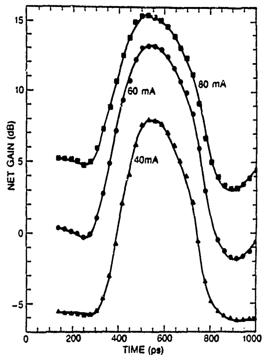
Fig. 2: Measured gain versus time
