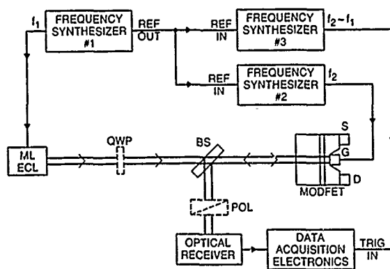
Figure 1: Experimental schematic. ML ECL = modelocked external cavity semiconductor laser.
