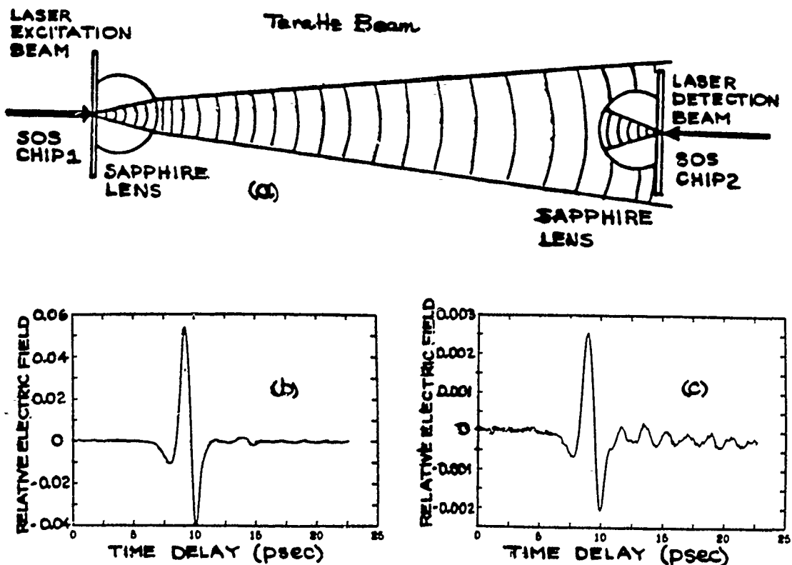
Figure 1. (a) Schematic diagram of the collimating and focusing terahertz optics. (b) Measured electrical pulse of the freely propagating terahertz beam with the detector located 10 cm from the source. (c) Measured pulse with the detector 100 cm from the source.
