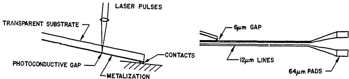
Figure 1 a) Cross-section of the probe. Optical pulses are focused thru the probe onto a photoconducting switch. The electrical pulse propagates to or from the device under test across the contacts at the end of the probe. b) Metalization on the bottom of the probe. The length of the line is 1.8 cm long. The third line is used to provide electrical contact for the side gap. Gold contacts are bonded to the end of the tapers.
