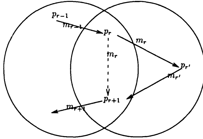
Figure 3: Causal Reversal
