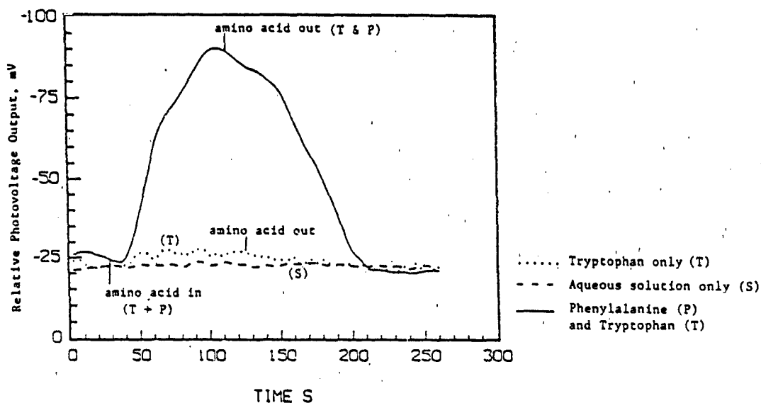
Figure 15. Comparison of optical waveguide sensor response to a) aqueous 0.1N HClO 4 , b) tryptophan (1g/200ml), and c) phenylalanine (1g/200ml + tryptophan (1g/200ml) at an evanescent wave optical sensor coated with quinoline chromagenic host (VIII). Solution flow rate 12ml/min.
