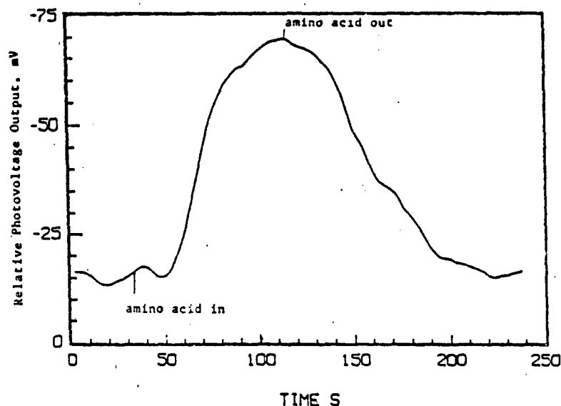
Figure 17. 3-hydroxytyrosine (dopa) response at an evanescent wave optical sensor. Solution = 1g/200ml H_2O (0.1N HClO_4 ). pH = 2-3. Fiber was spray coated with 20ml of solution containing .02g quinoline chromagenic host and 0.05 cellulose acetate. Solution flow rate 10ml/min.
