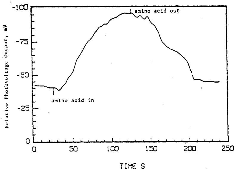
Figure 16. 3-hydroxytyrosine (dopa) response at an evanescent wave optical sensor. Solution = 1g/200ml H 2 O (0.1N HClO 4 ). pH = 2-3. Fiber was spray coated with 20ml of solution containing .005g quinoline chromagenic host (VIII) and 0.05g cellulose acetate. Solution flow rate 12ml/min -1 .
