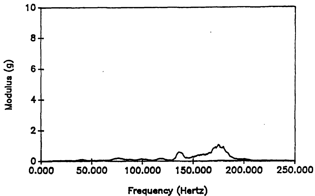
Figure A1.44. Modulus of Acceleration Record of Mass 3 for Antisymmetric Test Specimen of Test Run 5.
