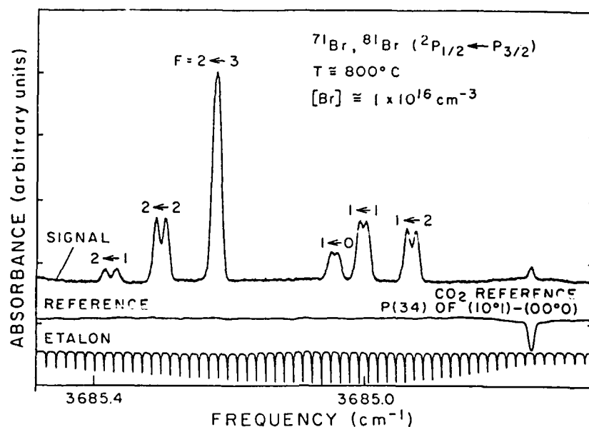
Fig. 2. Single mode continuous scan over the spin orbit transition in atomic bromine, \text{Br}^*(^2P_{1/2}) \leftarrow \text{Br}(^2P_{3/2}) .
