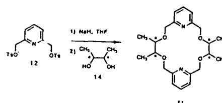
Scheme II. Preparation of Chiral Tetramethyl-bis-pyridino-18-crown-6
