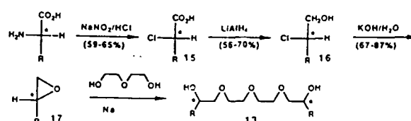
Scheme III. Preparation of Chiral Glycols
