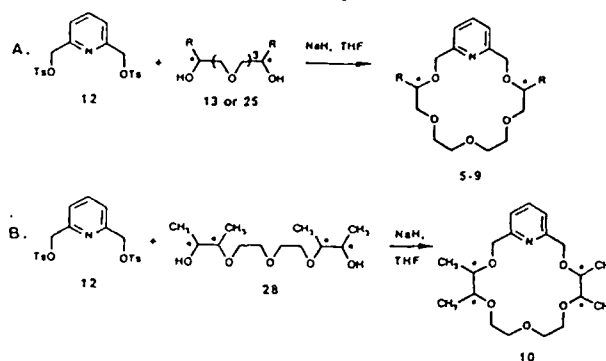
Scheme I. Preparation of Chiral Dialkyl-, Di-3-butenyl-, and Tetramethyl-crowns
