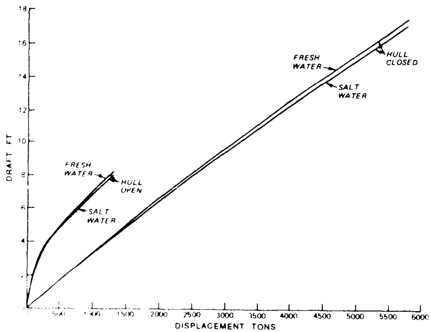
Figure 4. Barge load versus draft relationship
