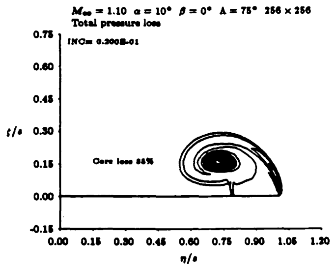
Figures 5 and 6 - Total pressure losses; 64 \times 64 & 256 \times 256 grids.
