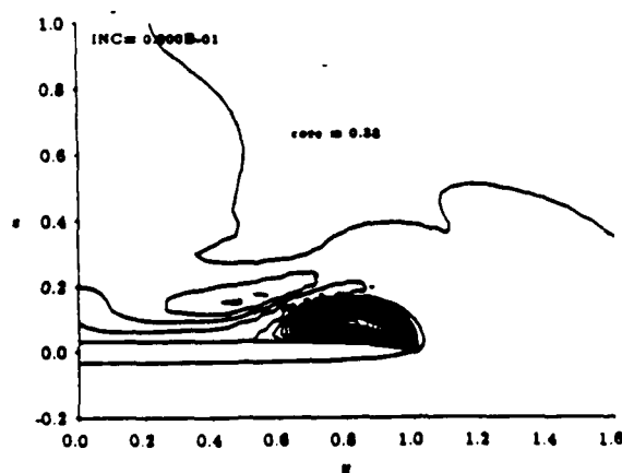
Figure 25: (1 - P_t/P_{t\infty}) at 78% chord, O-H grid. \alpha = 20^\circ , M_\infty = .85 .
