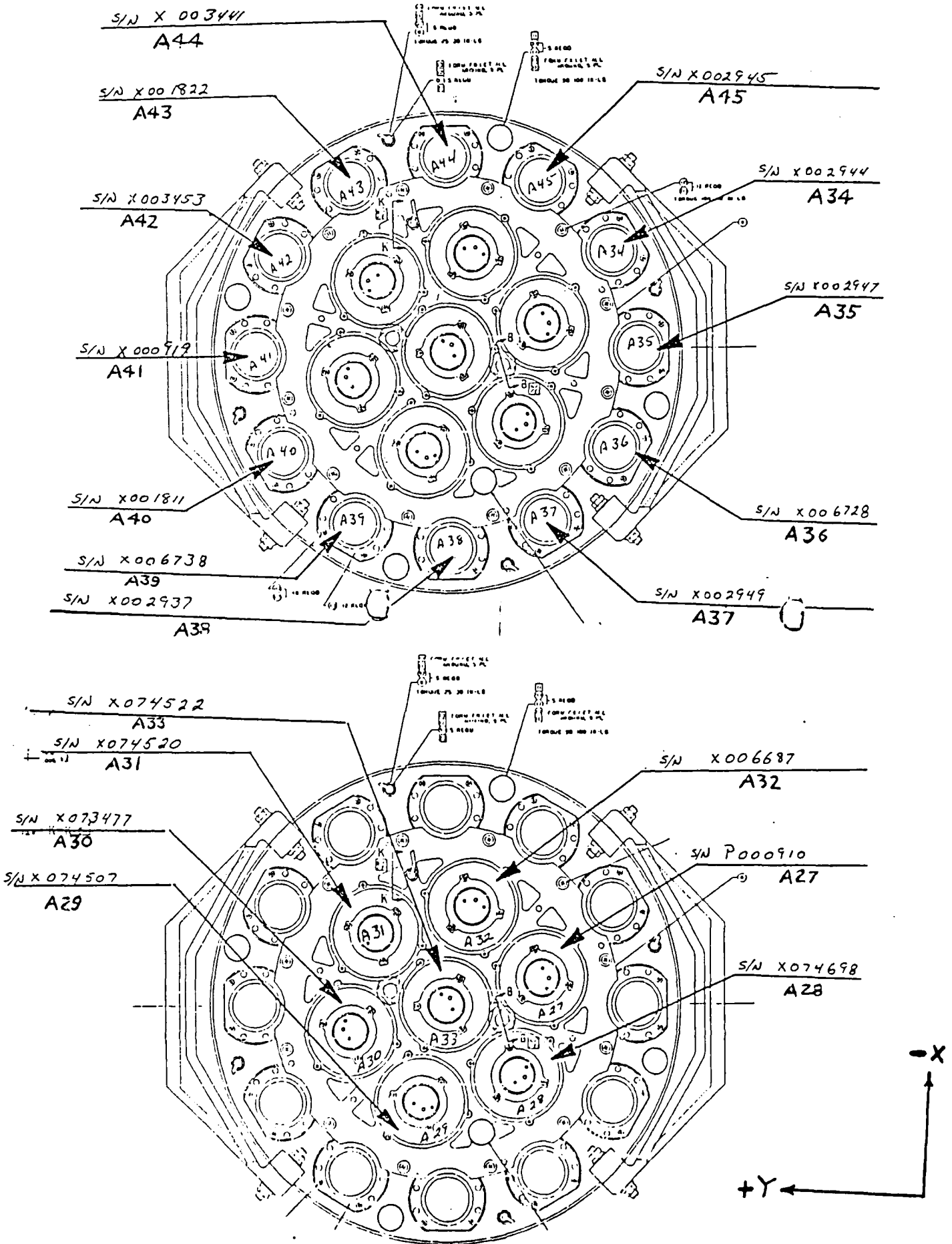
FIGURE 2-2. DETECTOR A2 PMT IDENTIFICATION
