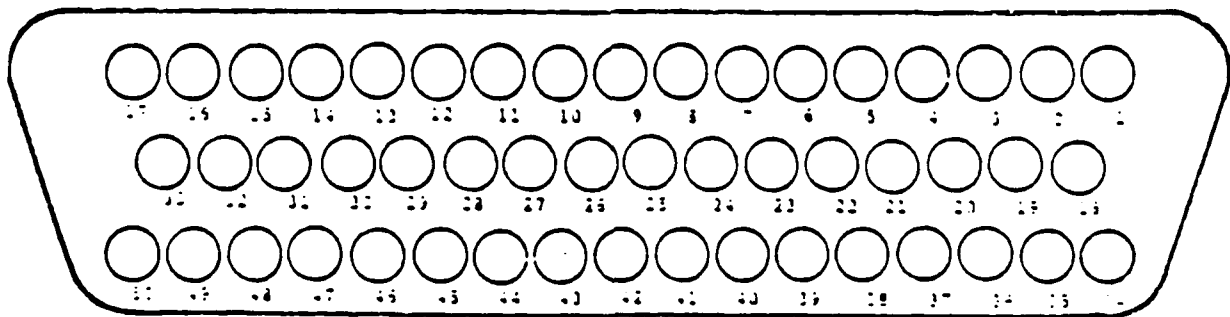
THE BOX/CHASSIS MATING/ENGAGING FACE IS SHOWN
