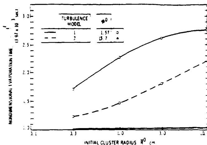
FIG. 6 Variation of a non-dimensional evaporation time with the initial radius of the cluster: T_{\infty} = 1000 K, T_0 = 350 K, Y_{F,\infty} = 0 , R^0 = 2 \times 10^{-1} cm, u_0 = 500 cm s ^{-1} .
