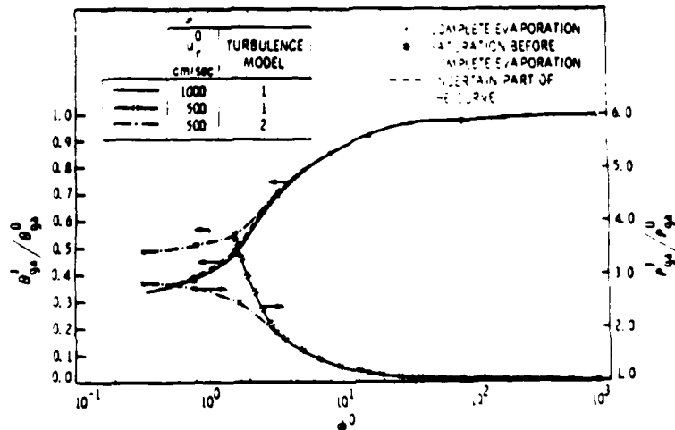
FIG. 3. Variation of \theta_g^0, \theta_m^0 and \rho_g^0, \rho_m^0 with the initial air fuel mass ratio. T_{\infty}^0 = 1000 K, T_p^0 = 350 K, Y_{F,\infty}^0 = 0 , R^0 = 10 cm, R^0 = 2 \times 10^{-3} cm.
