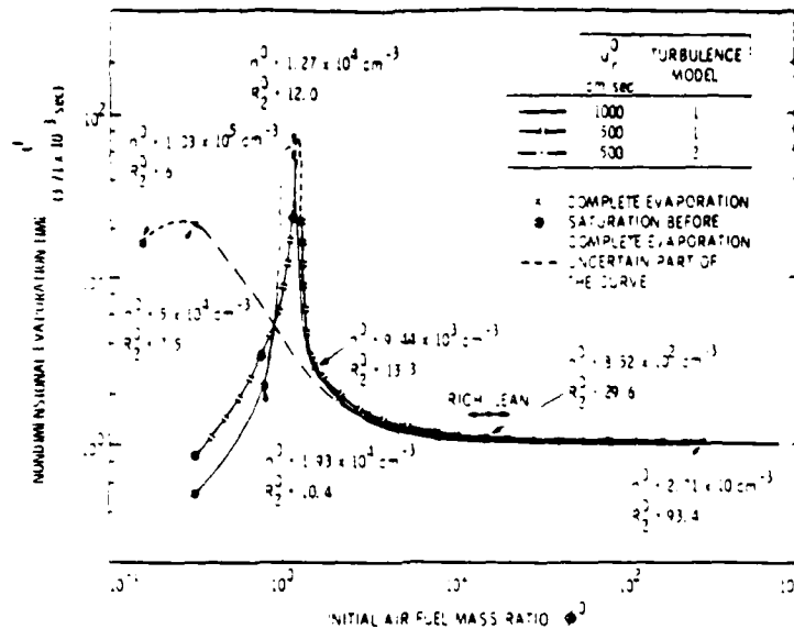
FIG. 2. Variation of \tau , non-dimensional evaporation time with the initial air fuel mass ratio. T_{\infty}^0 = 1000 K, T_p^0 = 350 K, Y_{F,\infty}^0 = 0 , R^0 = 10 cm, R^0 = 2 \times 10^{-3} cm.
