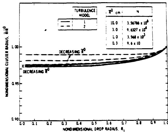
FIG. 9 Variation of the residual cluster radius with R_1 for different initial cluster radii for a dilute cluster of drops: T_{\infty}^0 = 1000 K, T_p^0 = 350 K, Y_{F,\infty}^0 = 0 , R^0 = 2 \times 10^{-3} cm, u^0 = 500 cm s ^{-1} , \phi^0 = 15.7 ( n^0 = 8.52 \times 10^2 cm ^{-3} , R_1^0 = 29.6 ).
