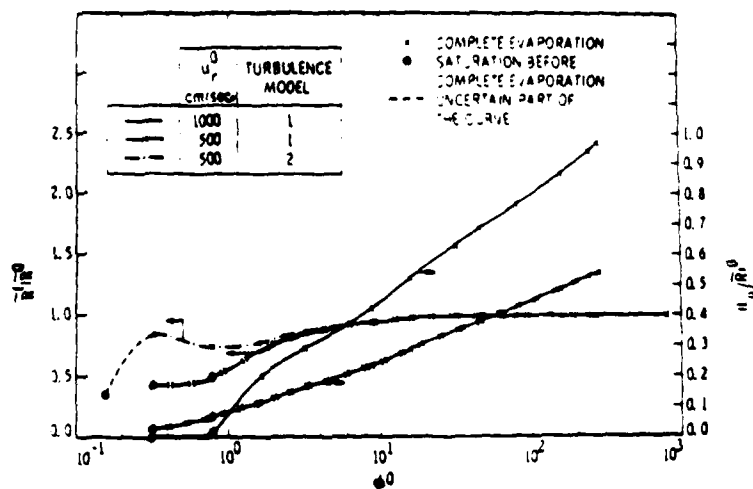
FIG. 5 Initial penetration ratio and final position of the cluster surface vs the initial air fuel mass ratio T_a^0 = 1000 K, T_a^0 = 350 K, Y_{F,a}^0 = 0 , \bar{R}^0 = 10 cm, R^0 = 2 \times 10^{-1} cm.
