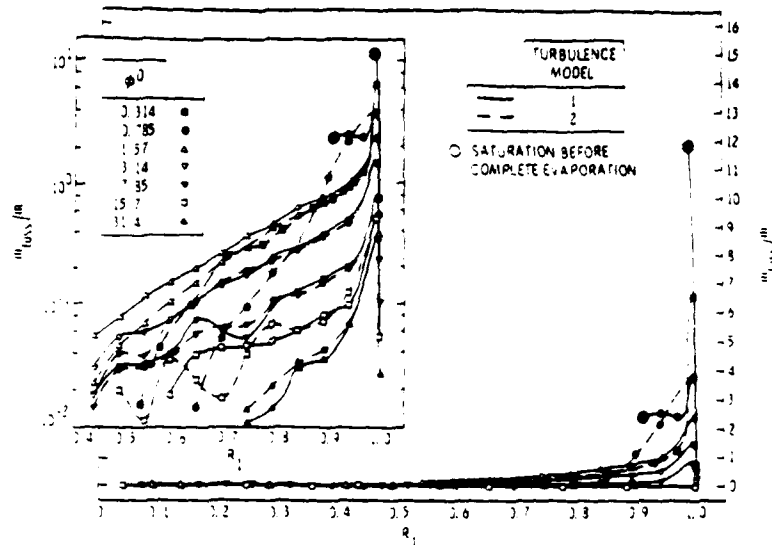
FIG. 4 Loss fraction vs R_i for various initial air fuel mass ratios T_a^0 = 1000 K, T_a^0 = 350 K, Y_{F,a}^0 = 0 , \bar{R}^0 = 10 cm, R^0 = 2 \times 10^{-1} cm, u^0 = 500 cm s ^{-1} .
