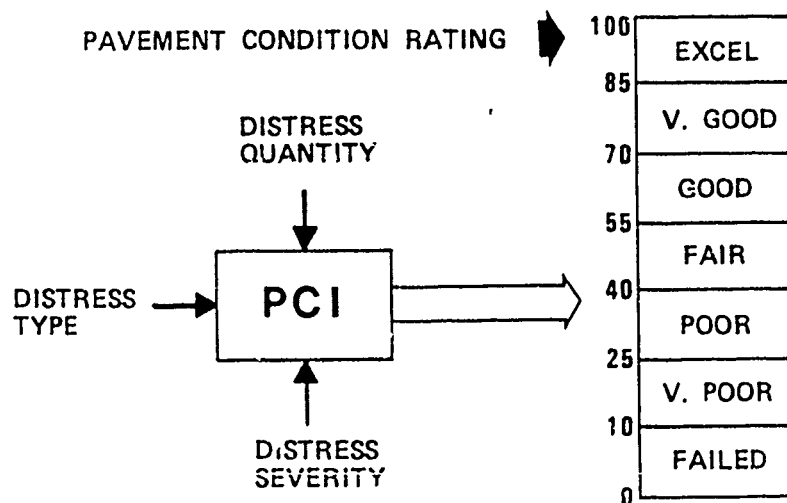
Figure 3. Pavement Condition Index (PCI).
