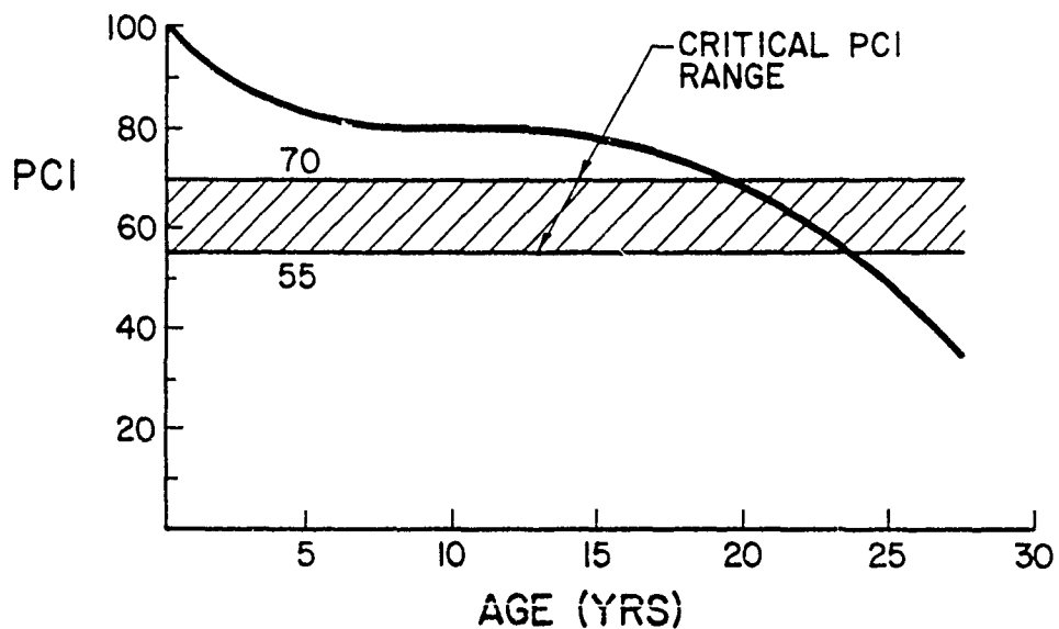
Figure 7. Critical PCI range.
