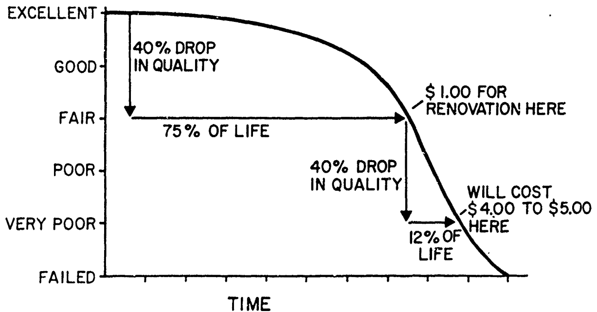
Figure 2. Typical pavement condition life cycle.
